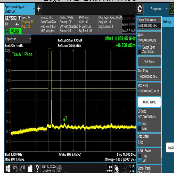
NTNV-N77-3700-3980-PC2-30-40-H-DFT-QPSK-
