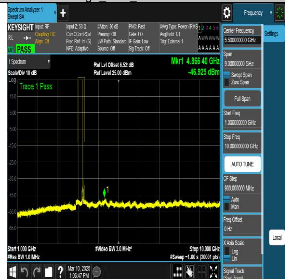
NTNV-N77-3700-3980-PC2-30-70-H-DFT-QPSK- Edge 1RB Left-Ant1-PASS
