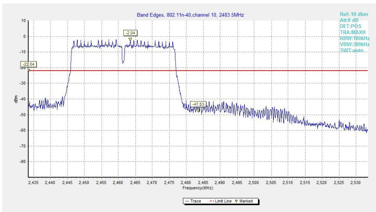
Fig.A.5.15 Band Edges (802.11n-HT40, Ch 10)
