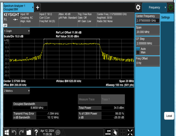
Band38-10MHz-16QAM-37800-50RB#0-PASS
