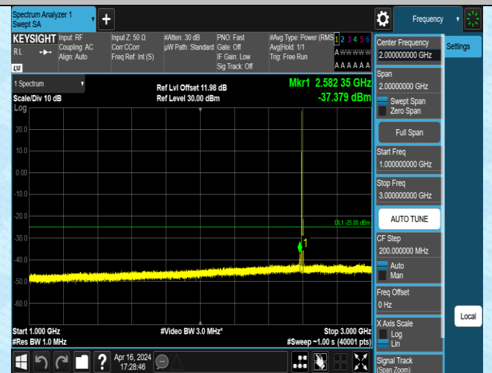
Band38_5MHz_QPSK_38000_1RB#0_1000~3000_1000~3000
