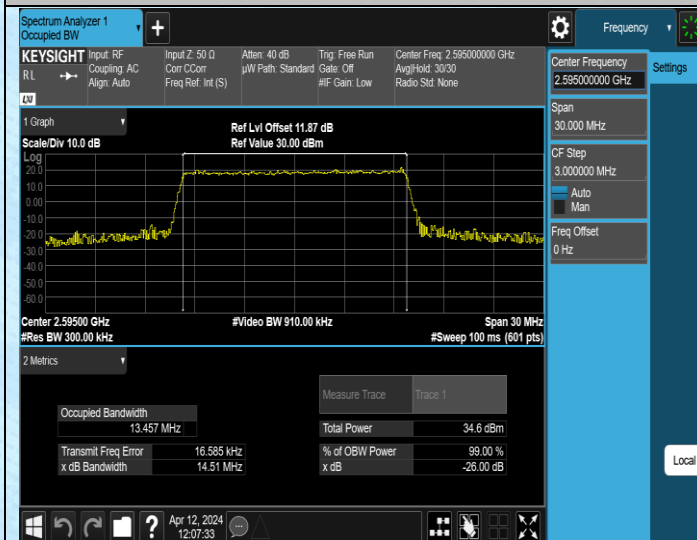
Band38-15MHz-16QAM-38000-75RB#0-PASS
