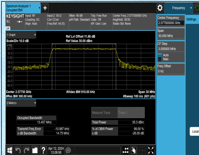
Band38-15MHz-QPSK-37825-75RB#0-PASS
