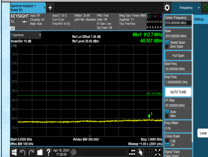
Band38_5MHz_QPSK_37775_1RB#0_30~1000_30~1000
