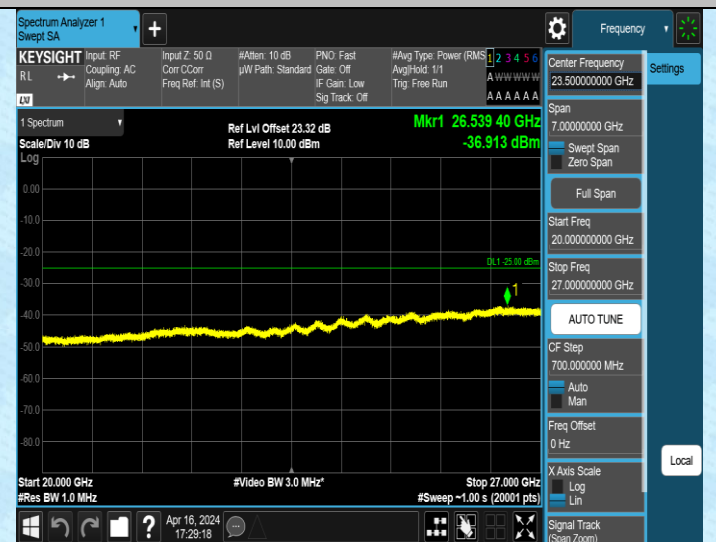
Band38_5MHz_QPSK_38000_1RB#0_20000~27000_20000~27000
