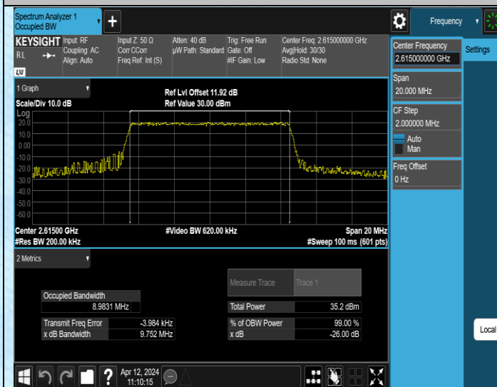
Band38-10MHz-QPSK-38200-50RB#0-PASS
