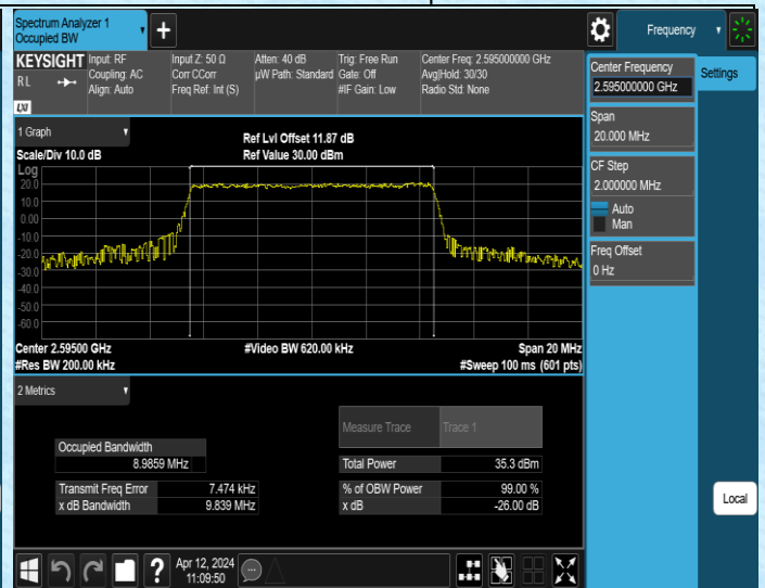
Band38-10MHz-QPSK-38000-50RB#0-PASS
