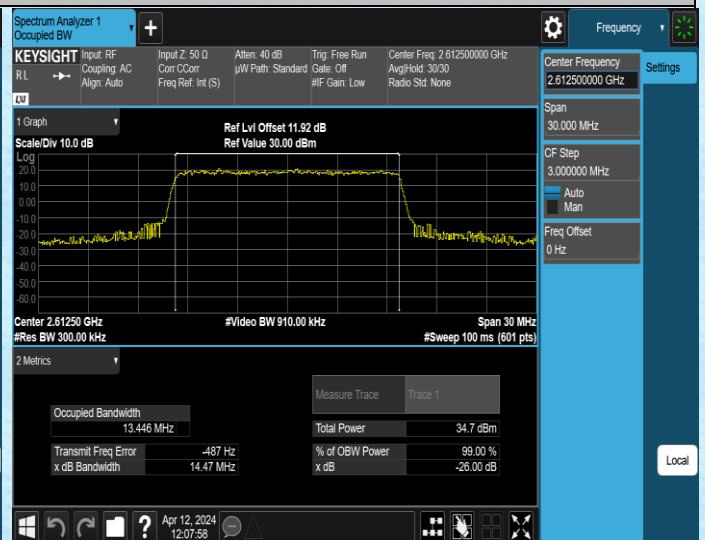
Band38-15MHz-16QAM-38175-75RB#0-PASS
