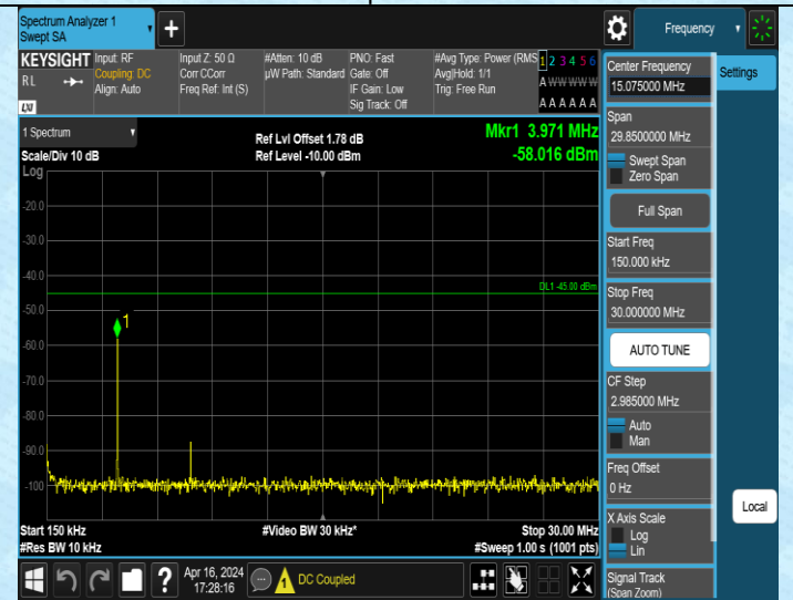
Band38_5MHz_QPSK_38000_1RB#0_0.15~30_0.15~30
