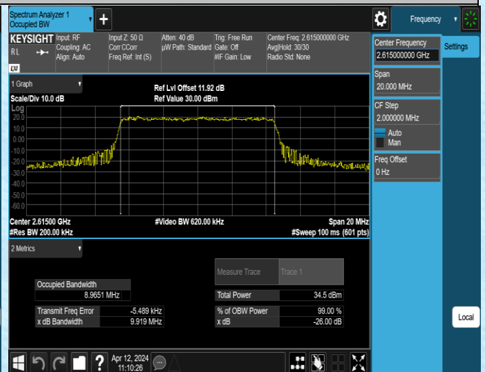
Band38-10MHz-16QAM-38200-50RB#0-PASS
