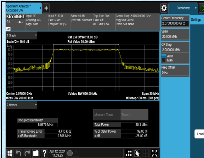
Band38-10MHz-QPSK-37800-50RB#0-PASS
