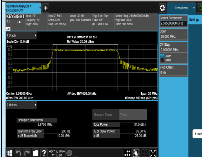
Band38-10MHz-16QAM-38000-50RB#0-PASS
