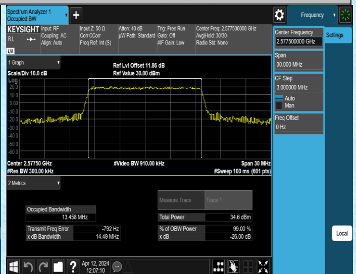
Band38-15MHz-16QAM-37825-75RB#0-PASS
