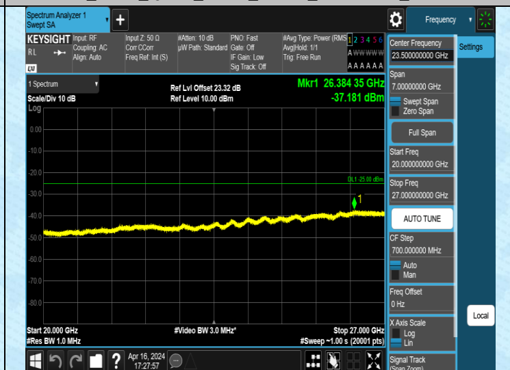
Band38_5MHz_QPSK_37775_1RB#0_20000~27000_20000~27000
