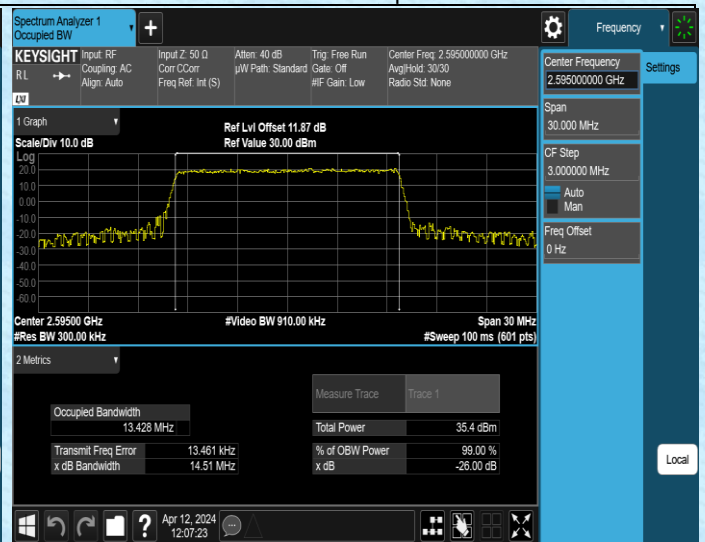
Band38-15MHz-QPSK-38000-75RB#0-PASS
