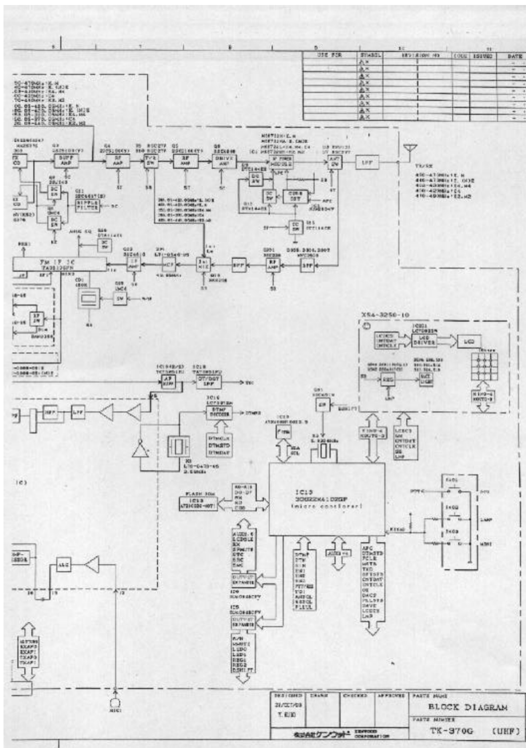
Block diagram(Right) Model name]TK-370GK2/TK-360GK2 FCC ID:ALH29473120
