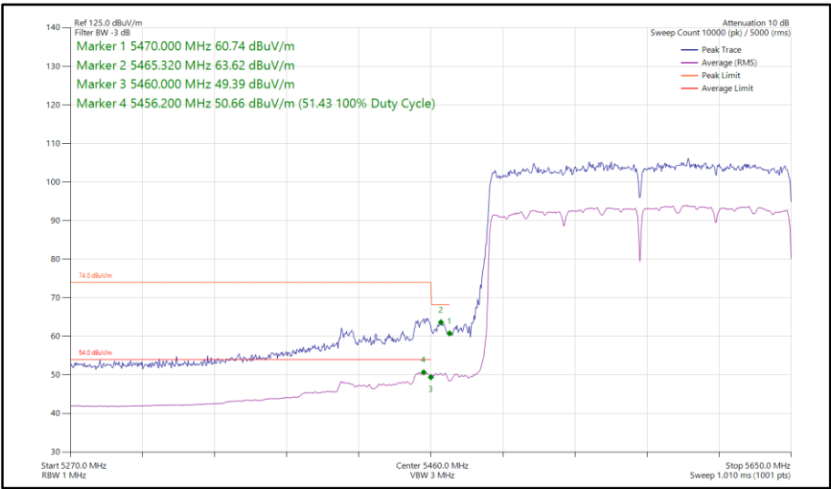
Figure 665 - 802.11ax HE160, SU, SISO, Core 1 - 5570 MHz Band Edge Frequency 5470 MHz
