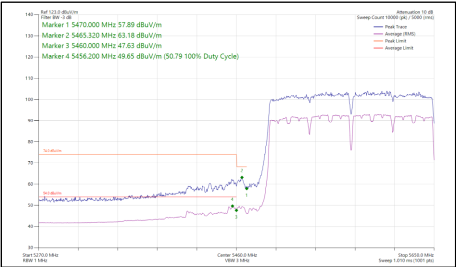
Figure 664 - 802.11ac VHT160, SISO, Core 1 - 5570 MHz Band Edge Frequency 5470 MHz
