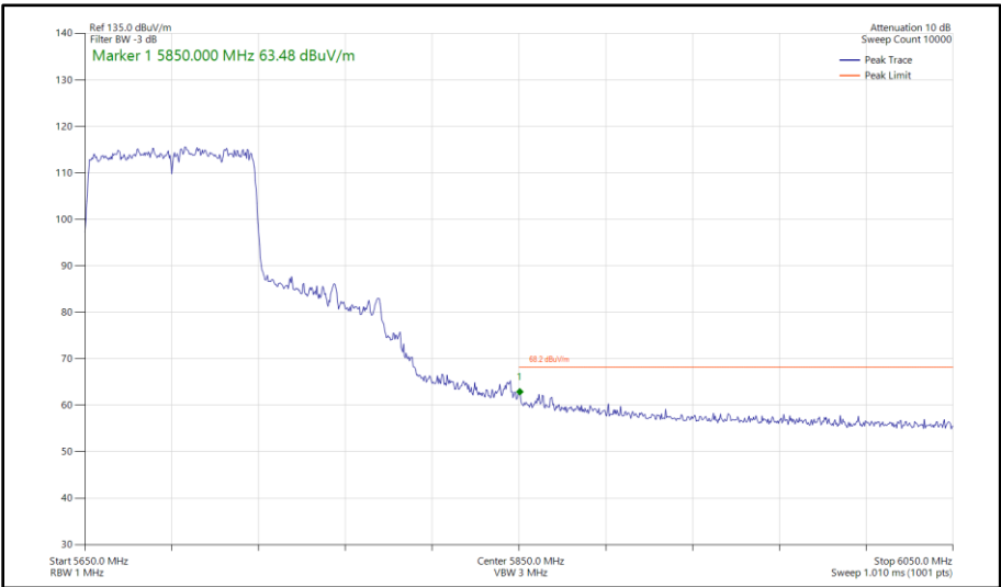
Figure 642 - 802.11ac VHT80, SDM, Core 0 - Core 1 - 5690 MHz Band Edge Frequency 5850 MHz
