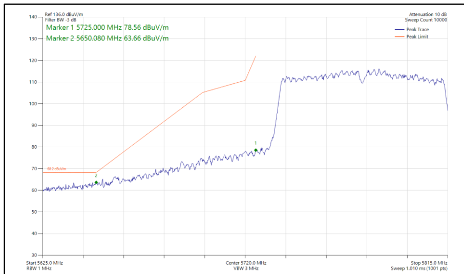
Figure 622 - 802.11ac VHT80, CDD, Core 0 - Core 1 - 5775 MHz Band Edge Frequency 5725 MHz
