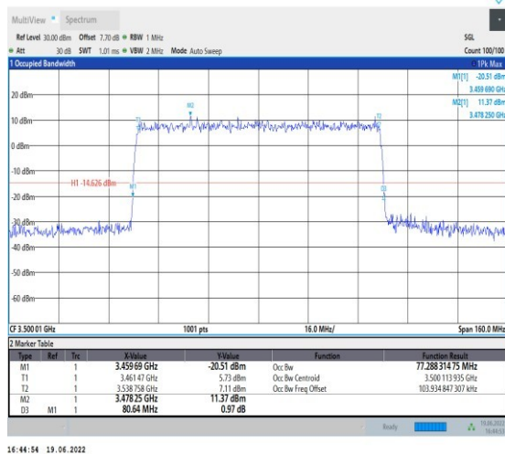
1-N78-3450-3550-PC2-30-80-M-9-CP-256QAM-Out er_Full-217@0-Ant1-77.288-80.640-≤80-PASS
