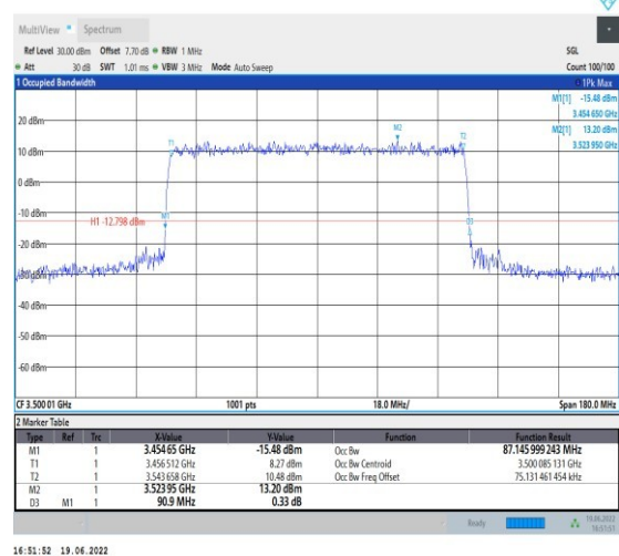
1-N78-3450-3550-PC2-30-90-M-7-CP-16QAM-Outer_Full-245@0-Ant1-87.146-90.900-≤90-PASS
