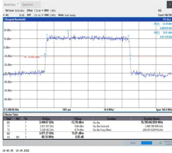
1-N78-3450-3550-PC2-30-80-L-4-DFT-64QAM-Outer_Full-216@0-Ant1-76.785-80.160-≤80-PASS
