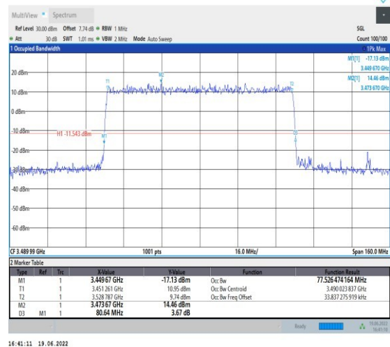
1-N78-3450-3550-PC2-30-80-L-7-CP-16QAM-Outer_Full-217@0-Ant1-77.526-80.640-≤80-PASS
