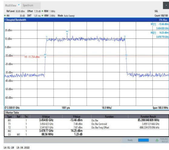
1-N78-3450-3550-PC2-30-90-M-5-DFT-256QAM-Out er_Full-240@0-Ant1-85.398-88.560-≤90-PASS
