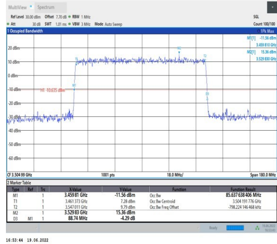
1-N78-3450-3550-PC2-30-90-H-4-DFT-64QAM-Oute_r_Full-240@0-Ant1-85.638-88.740-≤90-PASS
