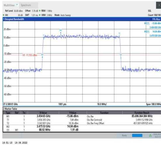
1-N78-3450-3550-PC2-30-90-M-4-DFT-64QAM-Out er_Full-240@0-Ant1-85.696-88.920-≤90-PASS
