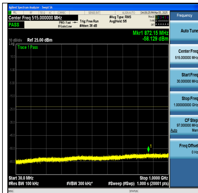
NTNV-n66-PC3-15-45-H-CP-QPSK-Edge_1RB_Left-30-1000-PASS
