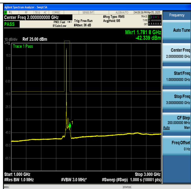
NTNV-n66-PC3-15-45-H-CP-QPSK-Edge_1RB_Left-1000-3000-PASS
