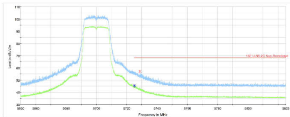
Fig. 4 Band Edges (802.11a, Ch140, 5700MHz, CHAIN 0)
