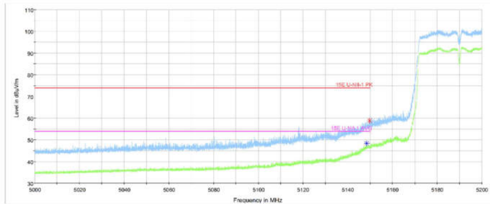
Fig. 9 Band Edges (802.11n-HT40 , Ch38, 5190MHz, MIMO)
