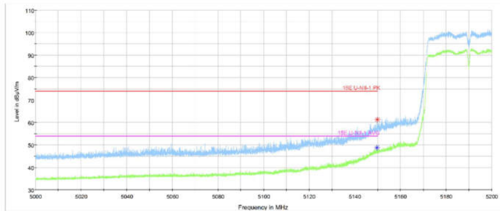
Fig. 17 Band Edges (802.11ac-HT40 , Ch38, 5190MHz, MIMO)
