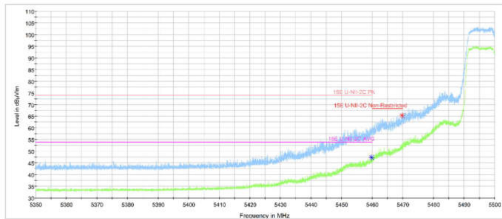
Fig. 7 Band Edges (802.11n-HT20 , Ch100, 5500MHz, MIMO)
