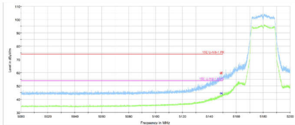
Fig. 13 Band Edges (802.11ac-HT20 , Ch36, 5180MHz, MIMO)
