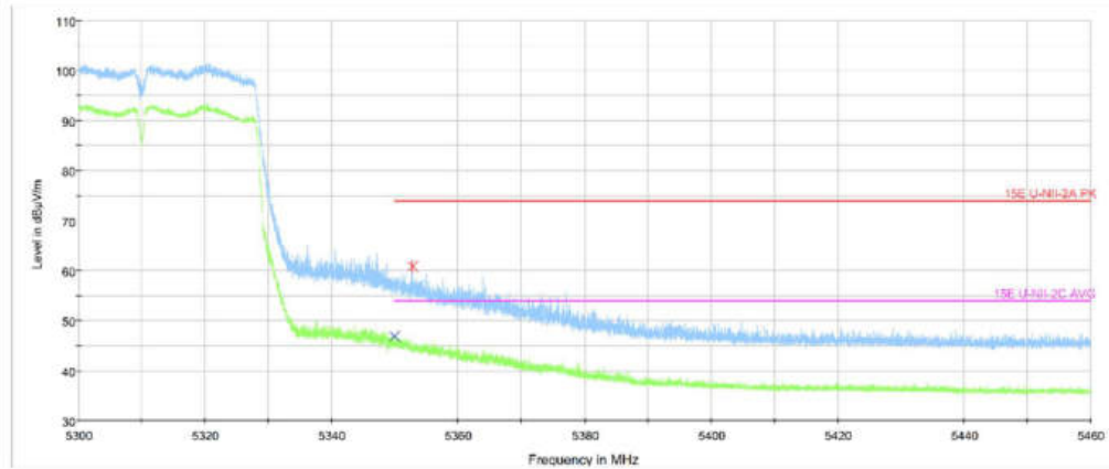
Fig. 18 Band Edges (802.11ac-HT40 , Ch62, 5310MHz, MIMO)
