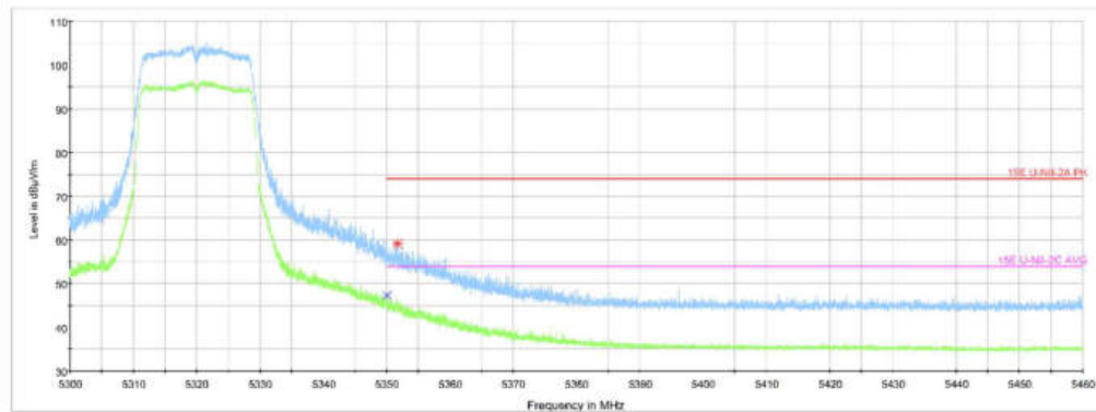
Fig. 6 Band Edges (802.11n-HT20 , Ch64, 5320MHz, MIMO)
