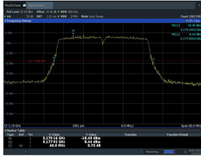
11AC40SISO_ANT10_5190
