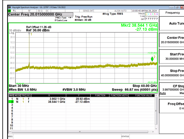
5G NR n77 80MHz QPSK Mid Channel RB1-1
