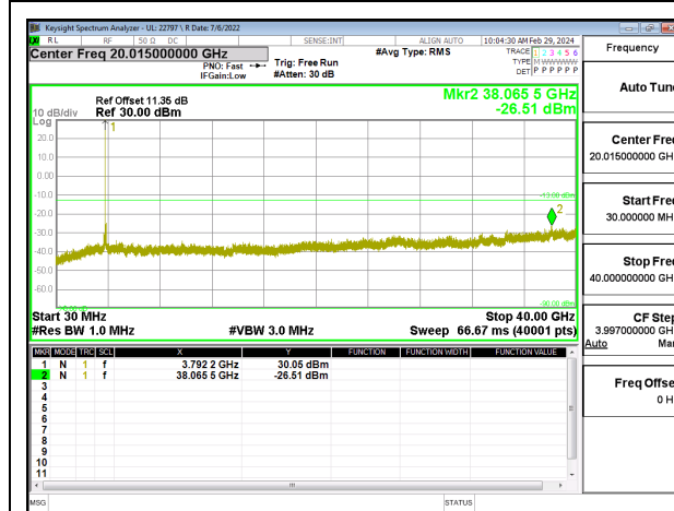
5G NR n77 100MHz QPSK High Channel RB1-105
