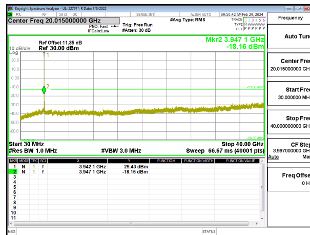
5G NR n77 40MHz QPSK Mid Channel RB1-1
