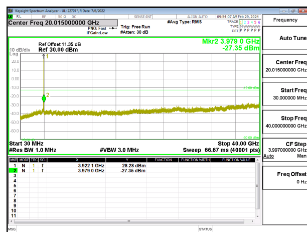
5G NR n77 60MHz QPSK High Channel RB1-77
