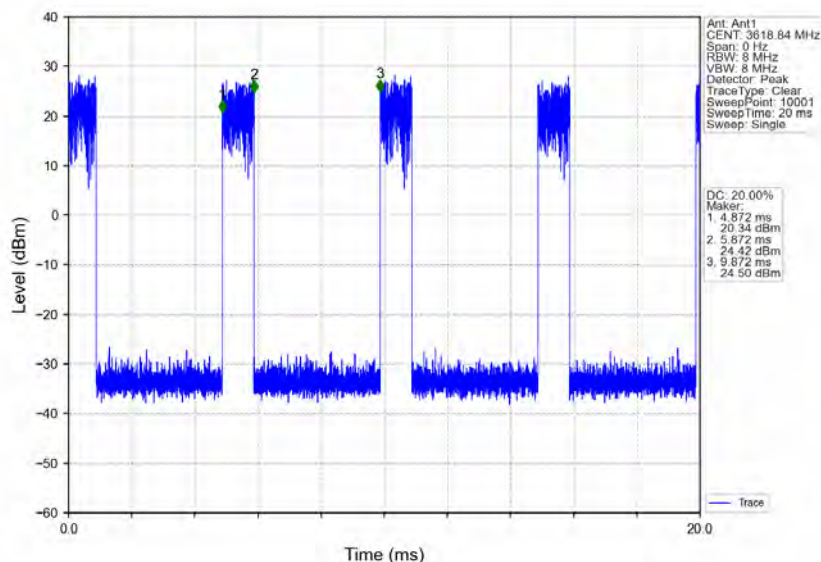
n78d_30kHz_MIMO_NTNV_70MHz_CP-OFDM_256_QAM_3585MHz_Edge_1RB_Right
