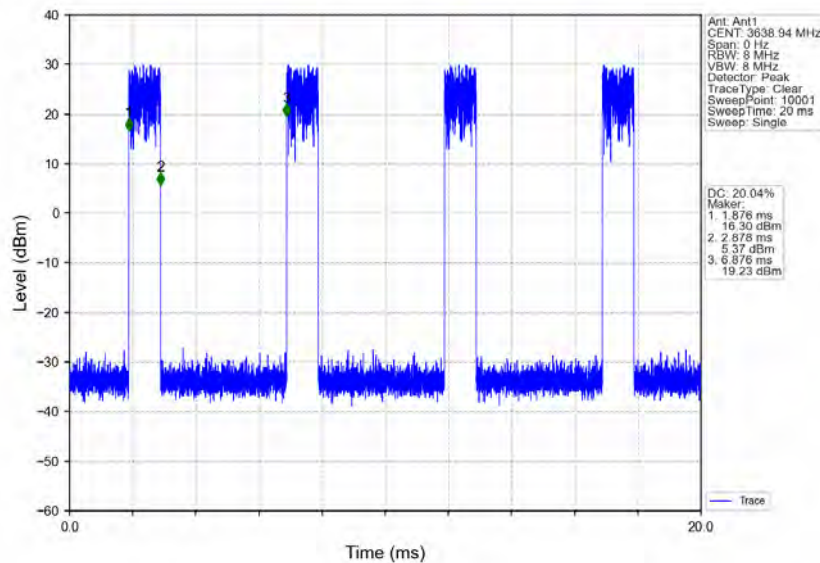
n78d_30kHz_MIMO_NTNV_90MHz_CP-OFDM_16_QAM_3595.02MHz_Edge_1RB_Right
