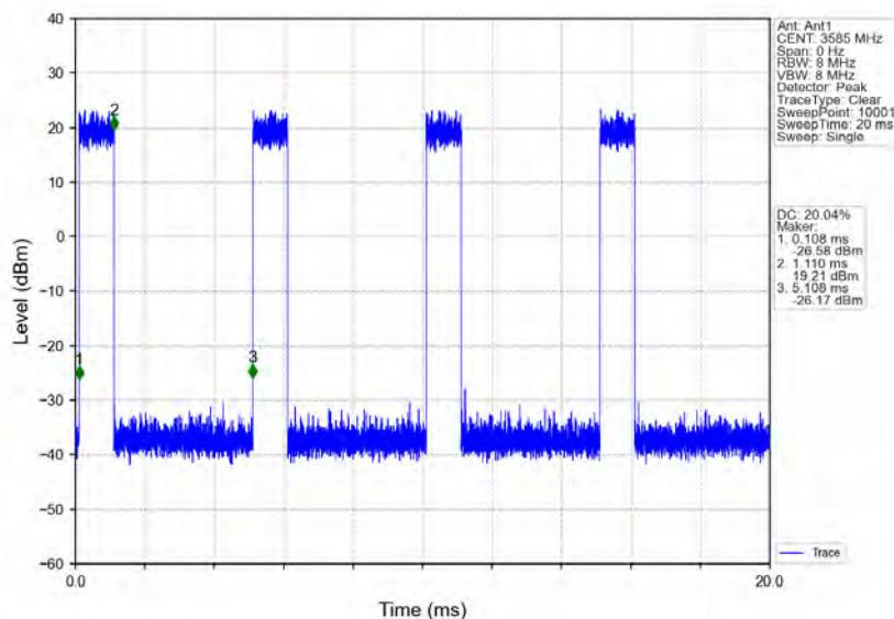
n78d_30kHz_MIMO_NTNV_70MHz_CP-OFDM_64_QAM_3585MHz_Inner_Full
