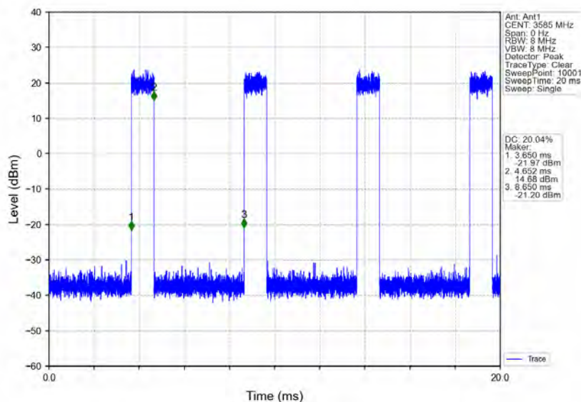
n78d_30kHz_MIMO_NTNV_70MHz_CP-OFDM_QPSK_3585MHz_Inner_Full
