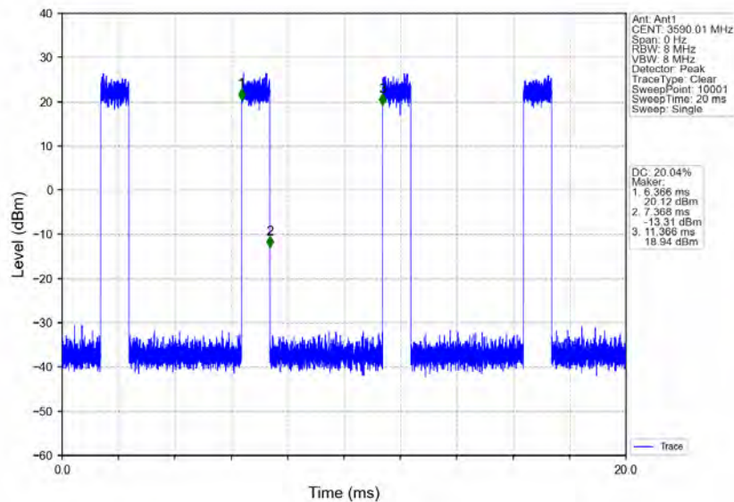
n78d_30kHz_MIMO_NTNV_80MHz_CP-OFDM_16_QAM_3590.01MHz_Inner_Full
