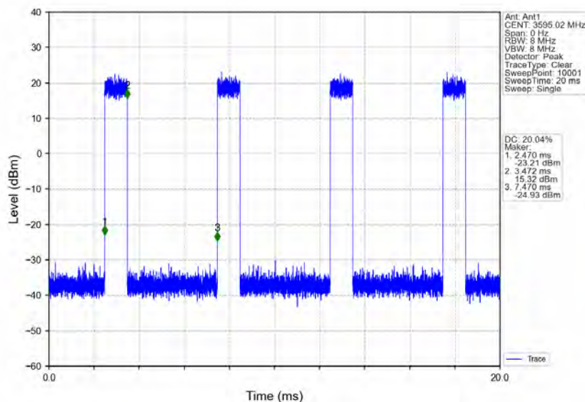
n78d_30kHz_MIMO_NTNV_90MHz_CP-OFDM_QPSK_3595.02MHz_Inner_Full
