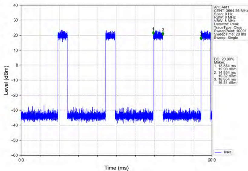
n78d_30kHz_MIMO_NTNV_70MHz_CP-OFDM_QPSK_3664.98MHz_Inner_Full
