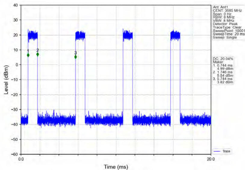
n78d_30kHz_MIMO_NTNV_70MHz_CP-OFDM_16_QAM_3585MHz_Inner_Full
