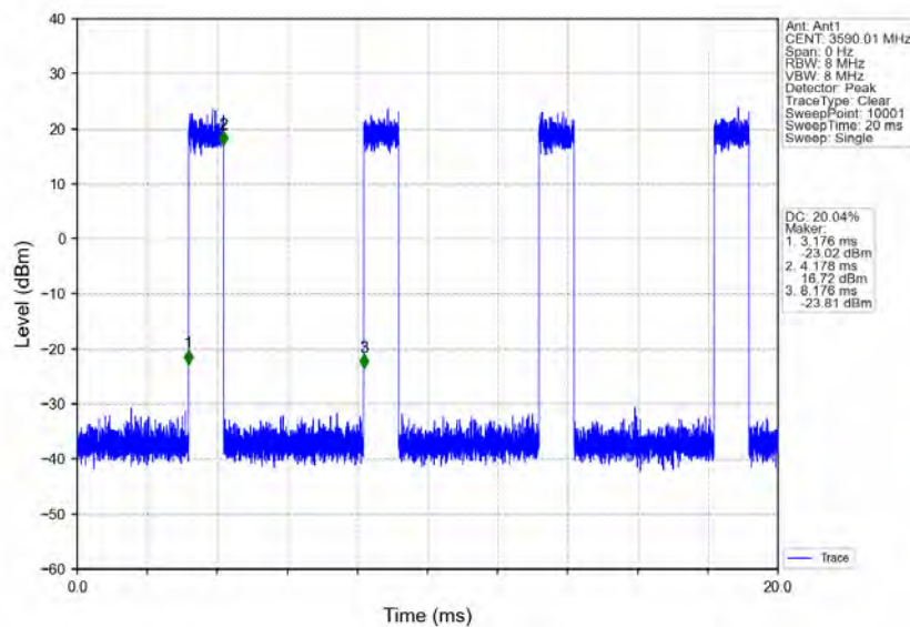
n78d_30kHz_MIMO_NTNV_80MHz_CP-OFDM_QPSK_3590.01MHz_Inner_Full
