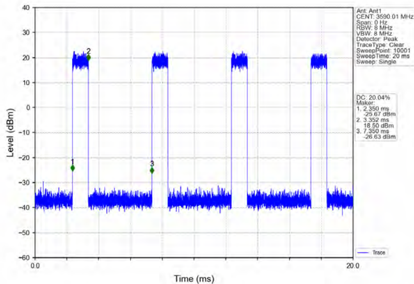
n78d_30kHz_MIMO_NTNV_80MHz_CP-OFDM 64 QAM_3590.01MHz_Inner_Full
