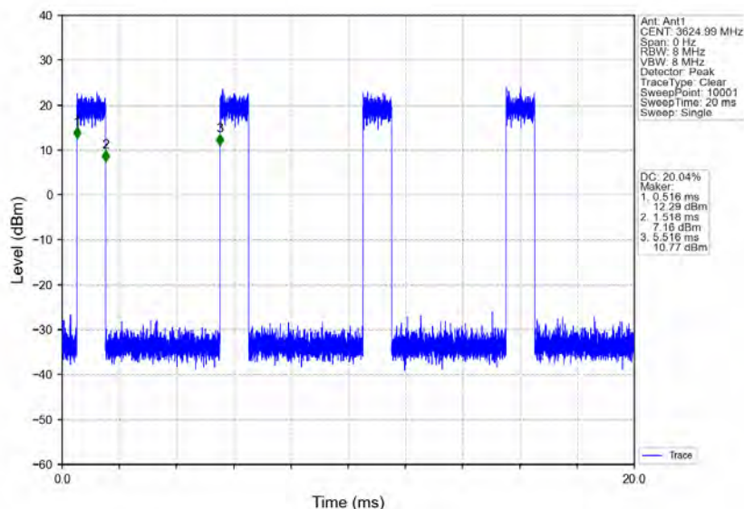
n78d_30kHz_MIMO_NTNV_80MHz_CP-OFDM_256_QAM_3624.99MHz_Inner_Full
