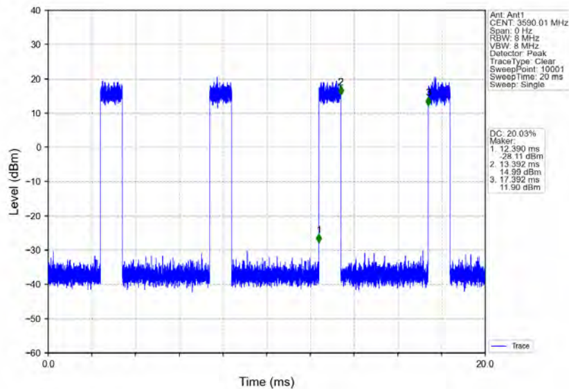
n78d_30kHz_MIMO_NTNV_80MHz_CP-OFDM_256_QAM_3590.01MHz_Inner_Full
