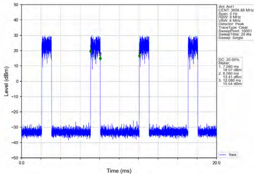
n78d_30kHz_MIMO_NTNV_80MHz_CP-OFDM_64_QAM_3660MHz_Edge_1RB_Right
