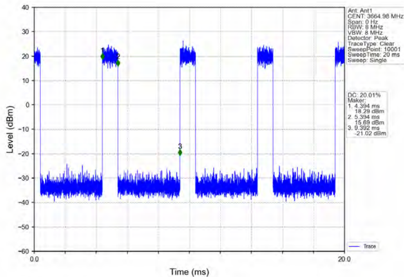
n78d_30kHz_MIMO_NTNV_70MHz_CP-OFDM_16_QAM_3664.98MHz_Inner_Full
