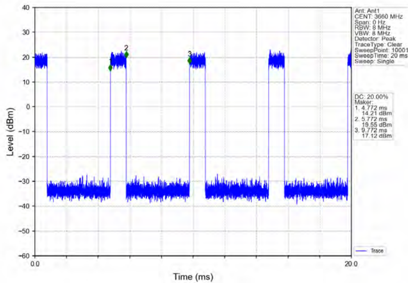
n78d_30kHz_MIMO_NTNV_80MHz_CP-OFDM_64_QAM_3660MHz_Inner_Full
