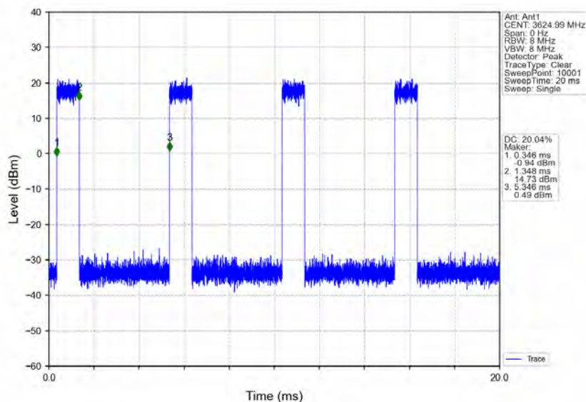
n78d_30kHz_MIMO_NTNV_60MHz_CP-OFDM_256_QAM_3624.99MHz_Inner_Full
