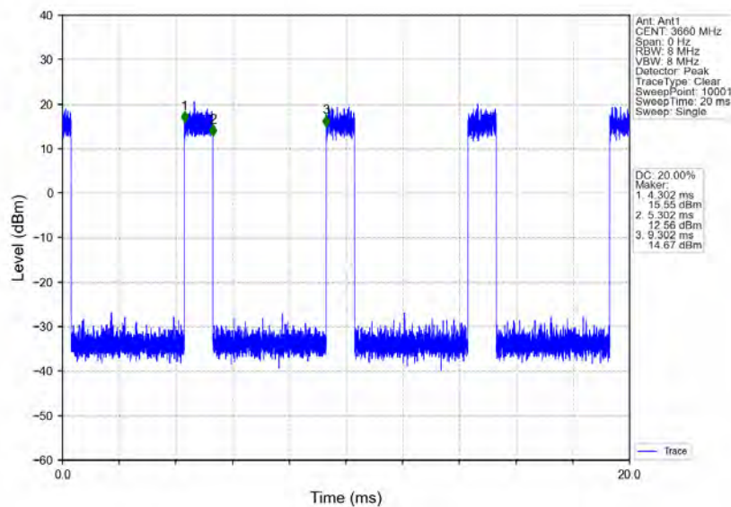
n78d_30kHz_MIMO_NTNV_80MHz_CP-OFDM_256_QAM_3660MHz_Inner_Full
