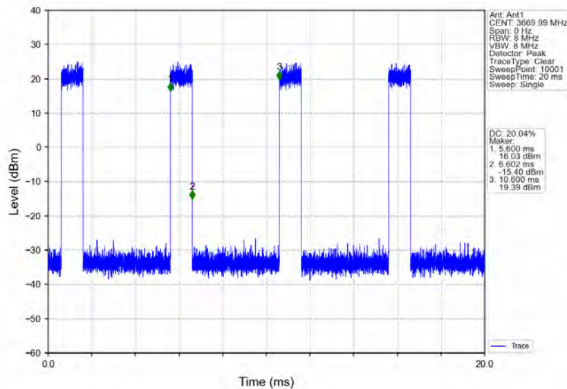
n78d_30kHz_MIMO_NTNV_60MHz_CP-OFDM_16_QAM_3669.99MHz_Inner_Full
