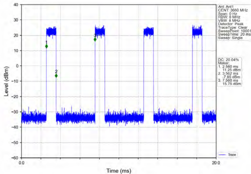
n78d_30kHz_MIMO_NTNV_80MHz_CP-OFDM_16_QAM_3660MHz_Inner_Full
