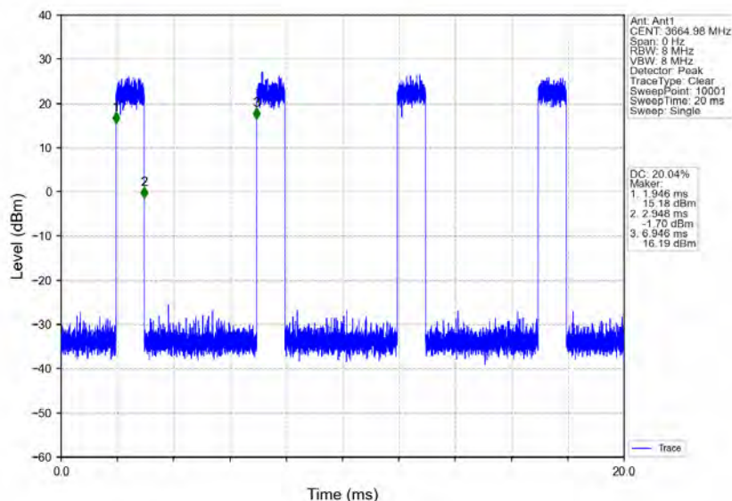
n78d_30kHz_MIMO_NTNV_70MHz_CP-OFDM_64_QAM_3664.98MHz_Inner_Full
