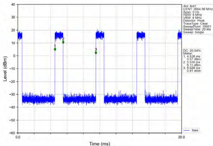
n78d_30kHz_MIMO_NTNV_70MHz_CP-OFDM_256_QAM_3664.98MHz_Inner_Full
