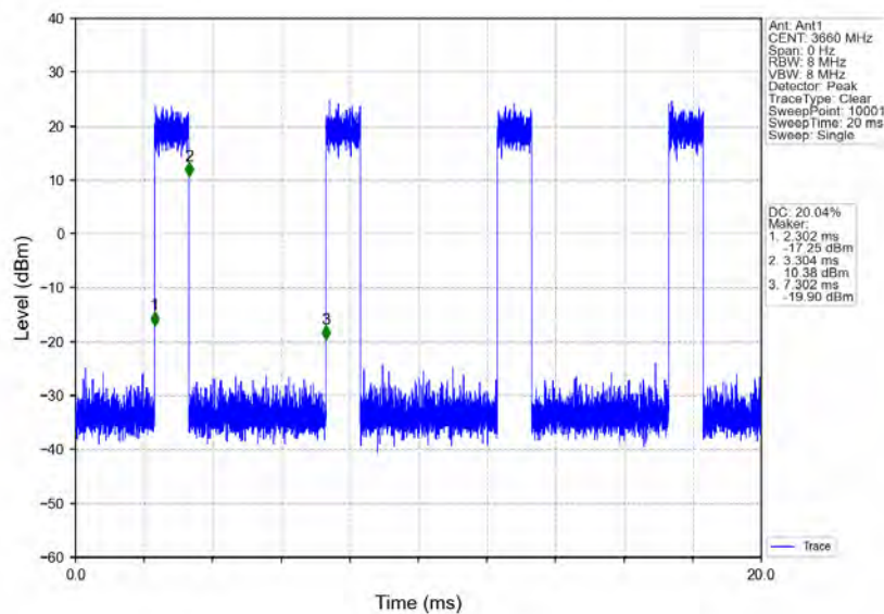
n78d_30kHz_MIMO_NTNV_80MHz_CP-OFDM_QPSK_3660MHz_Inner_Full
