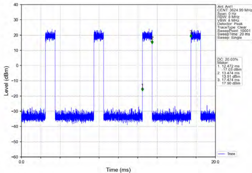
n78d_30kHz_MIMO_NTNV_80MHz_CP-OFDM_QPSK_3624.99MHz_Inner_Full
