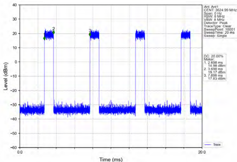
n78d_30kHz_MIMO_NTNV_80MHz_CP-OFDM_64_QAM_3624.99MHz_Inner_Full
