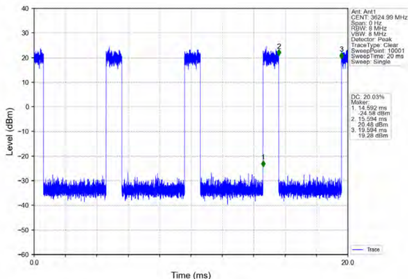
n78d_30kHz_MIMO_NTNV_70MHz_CP-OFDM_256_QAM_3624.99MHz_Inner_Full
