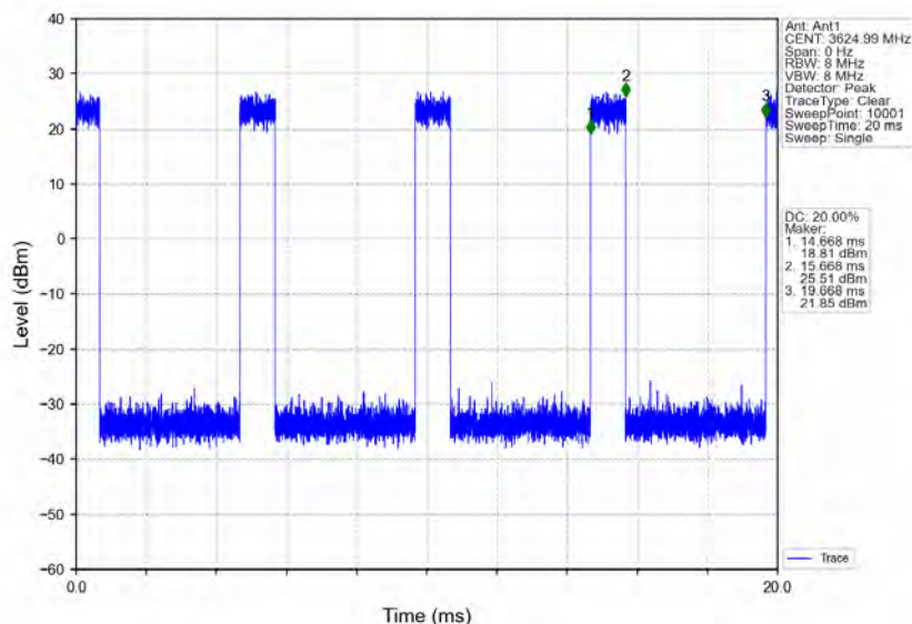
n78d_30kHz_MIMO_NTNV_70MHz_CP-OFDM_16_QAM_3624.99MHz_Inner_Full
