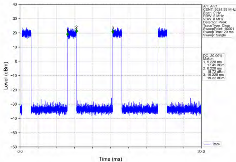
n78d_30kHz_MIMO_NTNV_70MHz_CP-OFDM 64 QAM_3624.99MHz_Inner_Full
