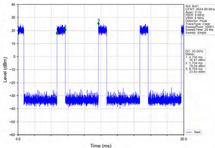
n78d_30kHz_MIMO_NTNV_70MHz_CP-OFDM_QPSK_3624.99MHz_Inner_Full
