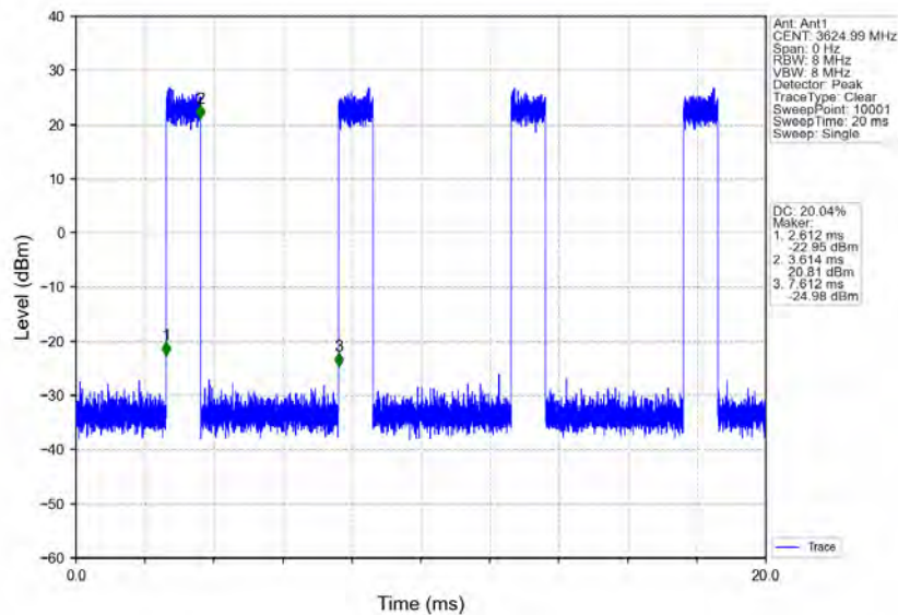
n78d_30kHz_MIMO_NTNV_80MHz_CP-OFDM_16_QAM_3624.99MHz_Inner_Full
