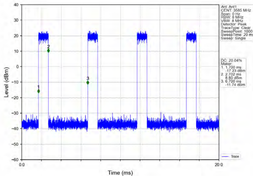
n78d_30kHz_MIMO_NTNV_70MHz_CP-OFDM_256_QAM_3585MHz_Inner_Full
