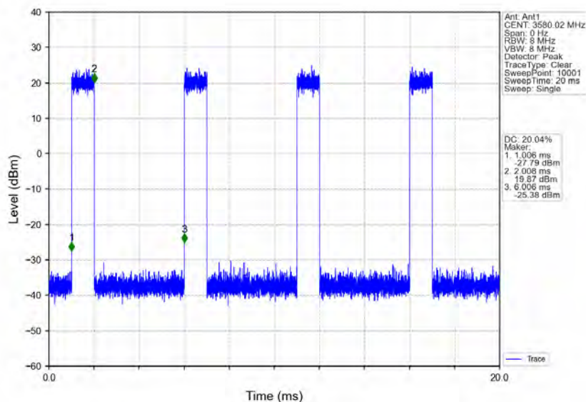
n78d_30kHz_MIMO_NTNV_60MHz_CP-OFDM 64 QAM_3580.02MHz_Inner_Full
