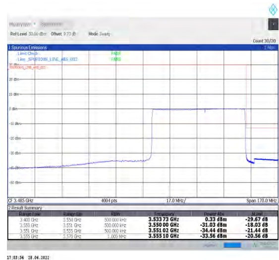
1-N77-3450-3550--30-60-H-6-CP-QPSK-Outer_Fu ll-162@0-Ant1-PASS-see graph
