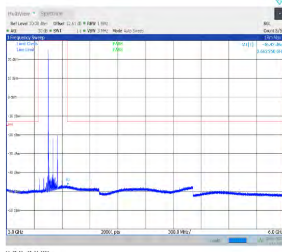
1-N77-3450-3550--30-100-M-1-DFT-QPSK-Edge_1R B_Left-1@0-3000-6000-Ant2--46.92--13-PASS
