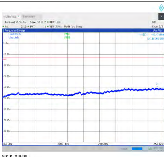
1-N77-3450-3550--30-100-M-1-DFT-QPSK-Edge_1R B_Left-1@0-6000-26000-Ant2--40.47--13-PASS
