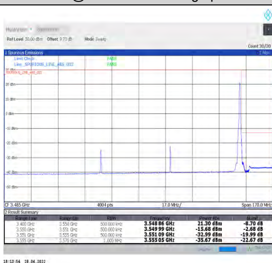
1-N77-3450-3550--30-90-H-5-CP-QPSK-Edge_1RB_Ri ght-1@244-Ant2-PASS-see graph
