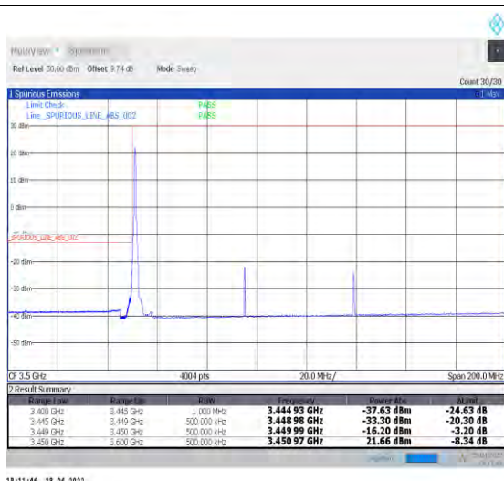
1-N77-3450-3550--30-90-L-4-CP-QPSK-Edge_1RB_Le ft-1@0-Ant2-PASS-see graph
