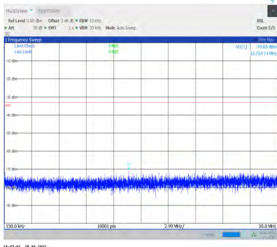
1-N77-3450-3550--30-100-M-1-DFT-QPSK-Edge_1R B_Left-1@0-0.15-30-Ant2--70.65--33-PASS
