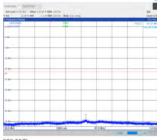
1-N77-3450-3550--30-100-M-1-DFT-QPSK-Edge_1R B_Left-1@0-30-1000-Ant2--67.21--23-PASS
