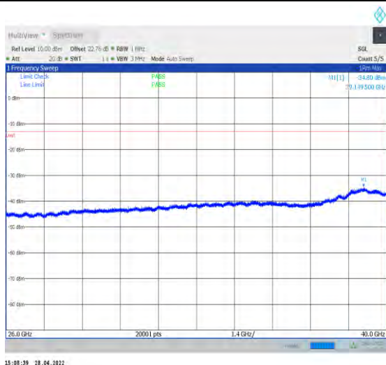
1-N77-3450-3550--30-100-L-1-DFT-QPSK-Edge_1R B_Left-1@0-26000-40000-Ant1--34.80--13-PASS
