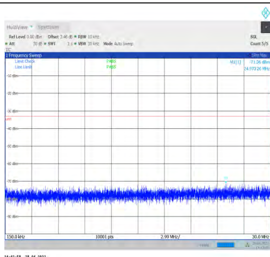
1-N77-3450-3550--30-100-M-1-DFT-QPSK-Edge_1R B_Left-1@0-0.15-30-Ant1--71.36--33-PASS
