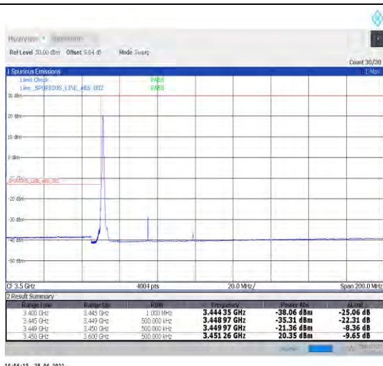
1-N77-3450-3550--30-50-L-4-CP-QPSK-Edge_1RB_Le ft-1@0-Ant1-PASS-see graph
