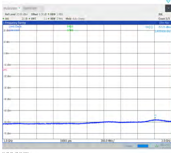
1-N77-3450-3550--30-100-M-1-DFT-QPSK-Edge_1R B_Left-1@0-1000-3000-Ant2--57.31--13-PASS
