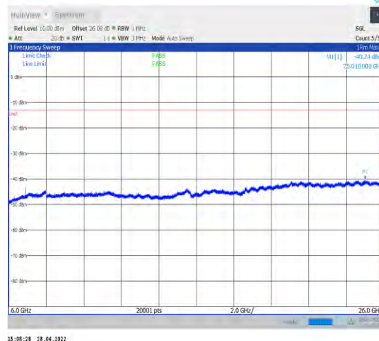
1-N77-3450-3550--30-100-L-1-DFT-QPSK-Edge_1R B_Left-1@0-6000-26000-Ant1--40.24--13-PASS
