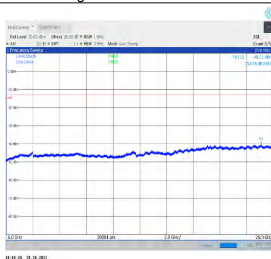
1-N77-3450-3550--30-100-L-1-DFT-QPSK-Edge_1R B_Left-1@0-6000-26000-Ant2--40.31--13-PASS
