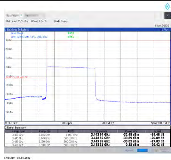
1-N77-3450-3550--30-60-L-6-CP-QPSK-Outer_Ful I-162@0-Ant1-PASS-see graph
