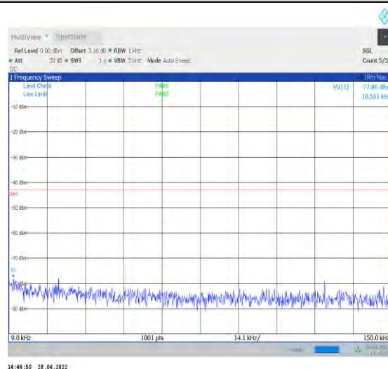
1-N77-3450-3550--30-100-M-1-DFT-QPSK-Edge_1R B_Left-1@0-0.009-0.15-Ant2--77.86--43-PASS
