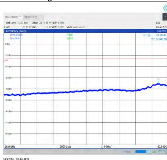
1-N77-3450-3550--30-100-M-1-DFT-QPSK-Edge_1R B_Left-1@0-26000-40000-Ant2--34.70--13-PASS
