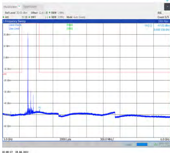
1-N77-3450-3550--30-100-L-1-DFT-QPSK-Edge_1R B_Left-1@0-3000-6000-Ant1--47.02--13-PASS
