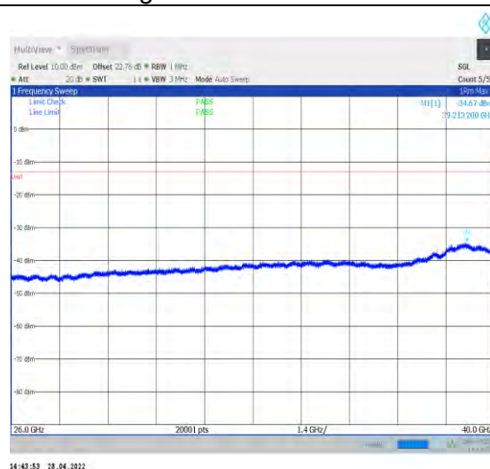
1-N77-3450-3550--30-100-M-1-DFT-QPSK-Edge_1R B_Left-1@0-26000-40000-Ant1--34.67--13-PASS
