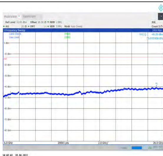
1-N77-3450-3550--30-100-M-1-DFT-QPSK-Edge_1R B_Left-1@0-6000-26000-Ant1--40.39--13-PASS
