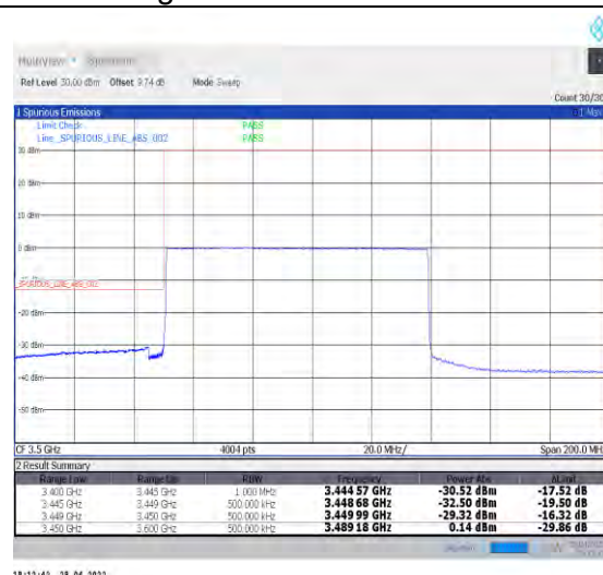
1-N77-3450-3550--30-90-L-6-CP-QPSK-Outer_Ful I-245@0-Ant2-PASS-see graph
