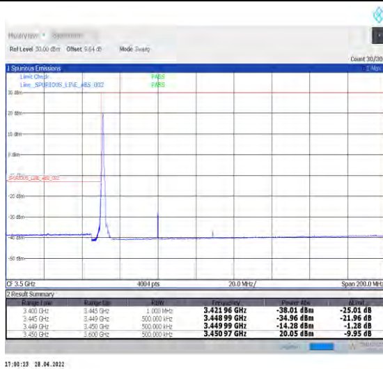
1-N77-3450-3550--30-60-L-4-CP-QPSK-Edge_1RB_Le ft-1@0-Ant1-PASS-see graph
