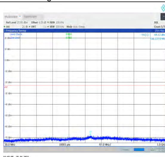
1-N77-3450-3550--30-100-M-1-DFT-QPSK-Edge_1R B_Left-1@0-30-1000-Ant1--68.12--23-PASS
