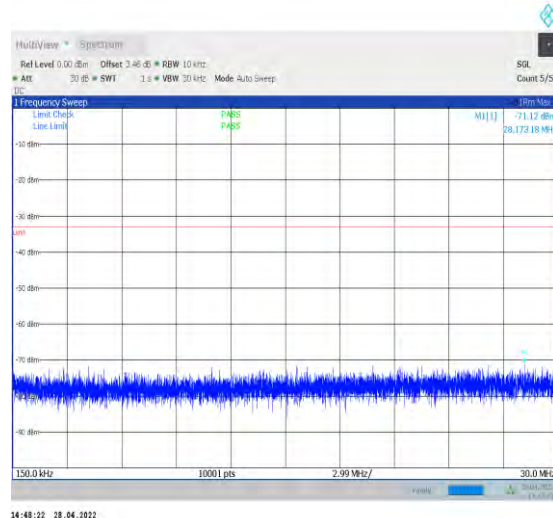
1-N77-3450-3550--30-100-H-1-DFT-QPSK-Edge_1R B_Left-1@0-0.15-30-Ant2--71.12--33-PASS
