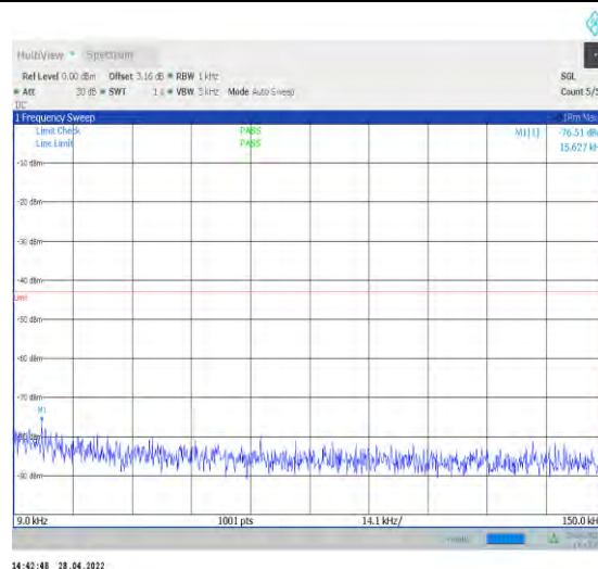
1-N77-3450-3550--30-100-M-1-DFT-QPSK-Edge_1R B_Left-1@0-0.009-0.15-Ant1--76.51--43-PASS
