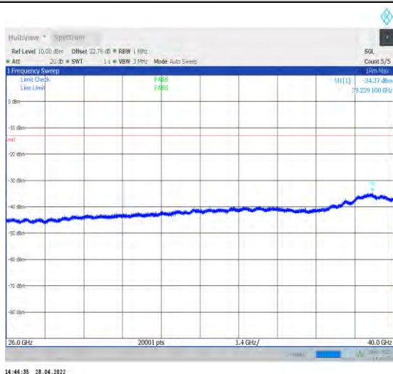
1-N77-3450-3550--30-100-L-1-DFT-QPSK-Edge_1R B_Left-1@0-26000-40000-Ant2--34.37--13-PASS
