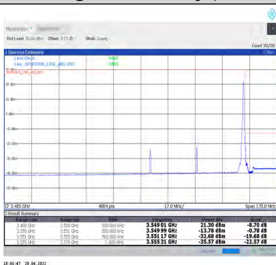
1-N77-3450-3550--30-60-H-5-CP-QPSK-Edge_1RB_Ri ght-1@161-Ant2-PASS-see graph
