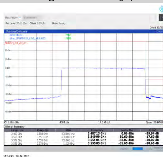
1-N77-3450-3550--30-90-H-6-CP-QPSK-Outer_Fu ll-245@0-Ant2-PASS-see graph
