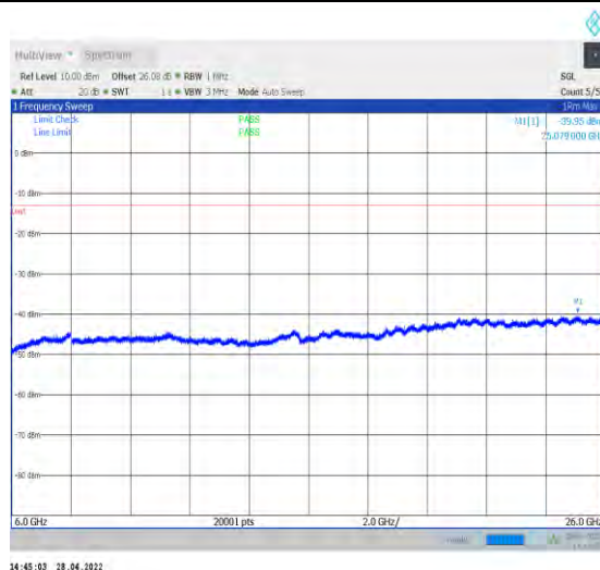
1-N77-3450-3550--30-100-H-1-DFT-QPSK-Edge_1R B_Left-1@0-6000-26000-Ant1--39.95--13-PASS
