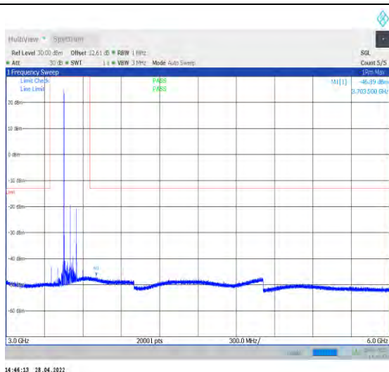
1-N77-3450-3550--30-100-L-1-DFT-QPSK-Edge_1R B_Left-1@0-3000-6000-Ant2--46.89--13-PASS
