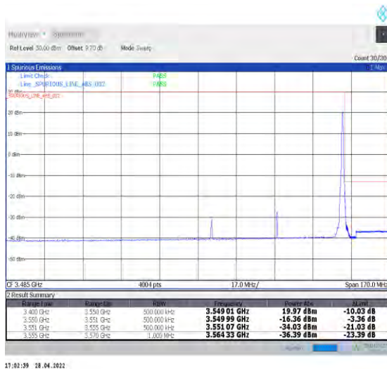
1-N77-3450-3550--30-60-H-5-CP-QPSK-Edge_1RB_Ri ght-1@161-Ant1-PASS-see graph
