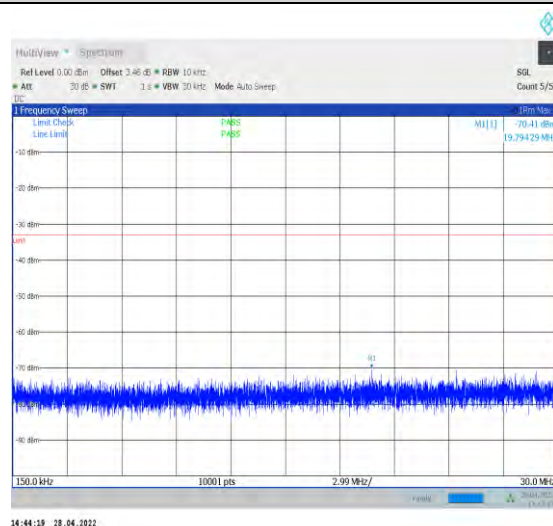
1-N77-3450-3550--30-100-H-1-DFT-QPSK-Edge_1R B_Left-1@0-0.15-30-Ant1--70.41--33-PASS
