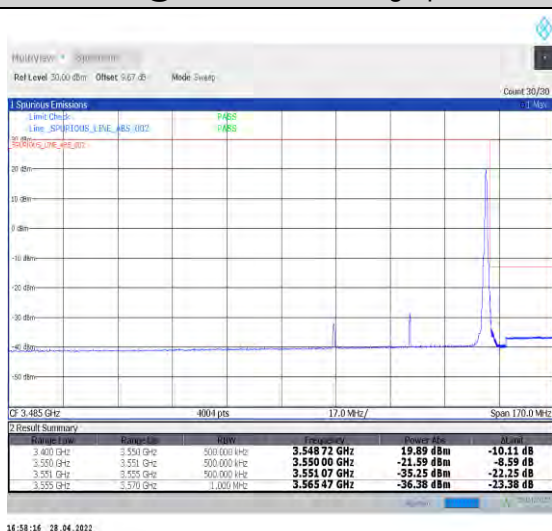
1-N77-3450-3550--30-50-H-5-CP-QPSK-Edge_1RB_Ri ght-1@132-Ant1-PASS-see graph
