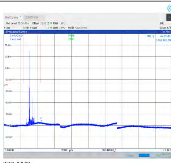
1-N77-3450-3550--30-100-M-1-DFT-QPSK-Edge_1R B_Left-1@0-3000-6000-Ant1--46.79--13-PASS
