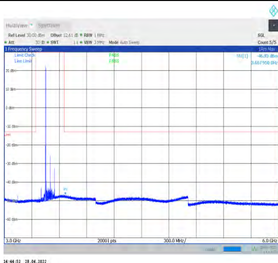
1-N77-3450-3550--30-100-H-1-DFT-QPSK-Edge_1R B_Left-1@0-3000-6000-Ant1--46.93--13-PASS
