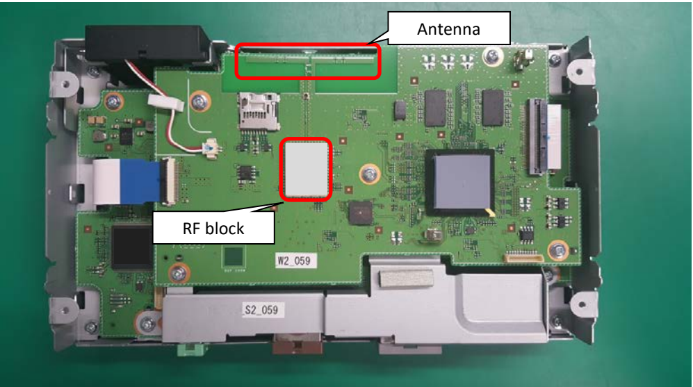
Fig.3 SB-ECU appearance without "TOP Cover"
