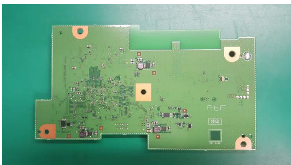
Fig.5 WiFi PCB (Back side)
