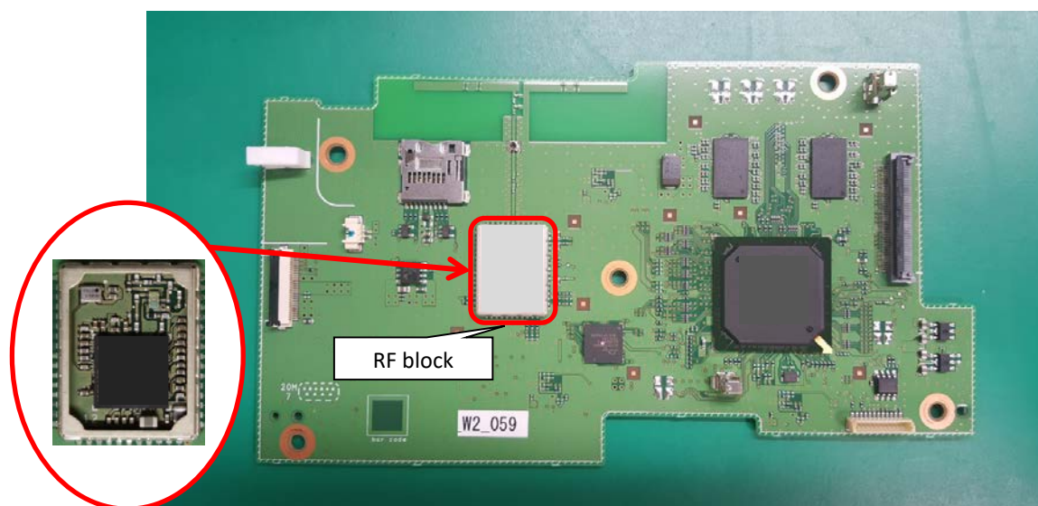
Fig.4 WiFi PCB (Surface side)
