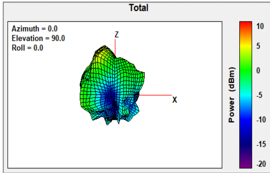
Band 4-5.800GHz X-Z plane View
