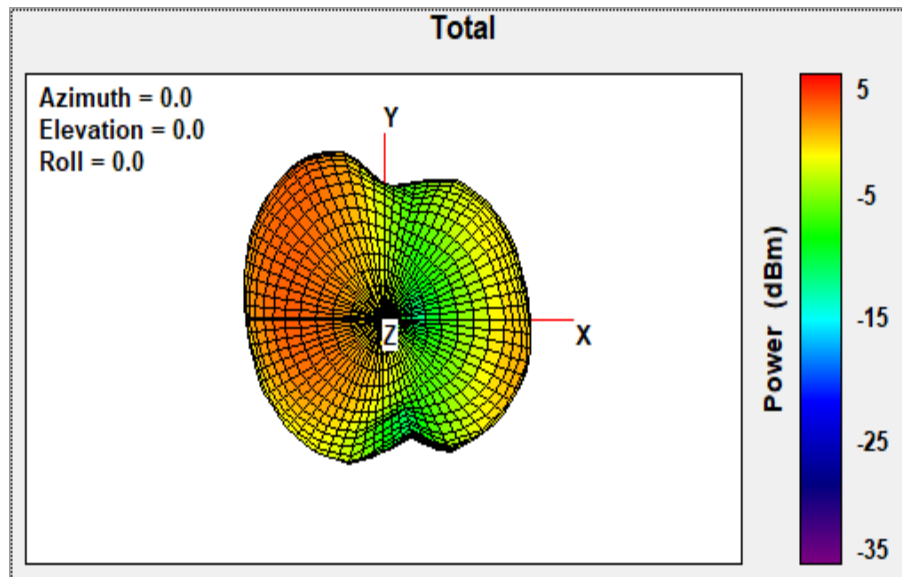
2.44GHz X-Y plane View
