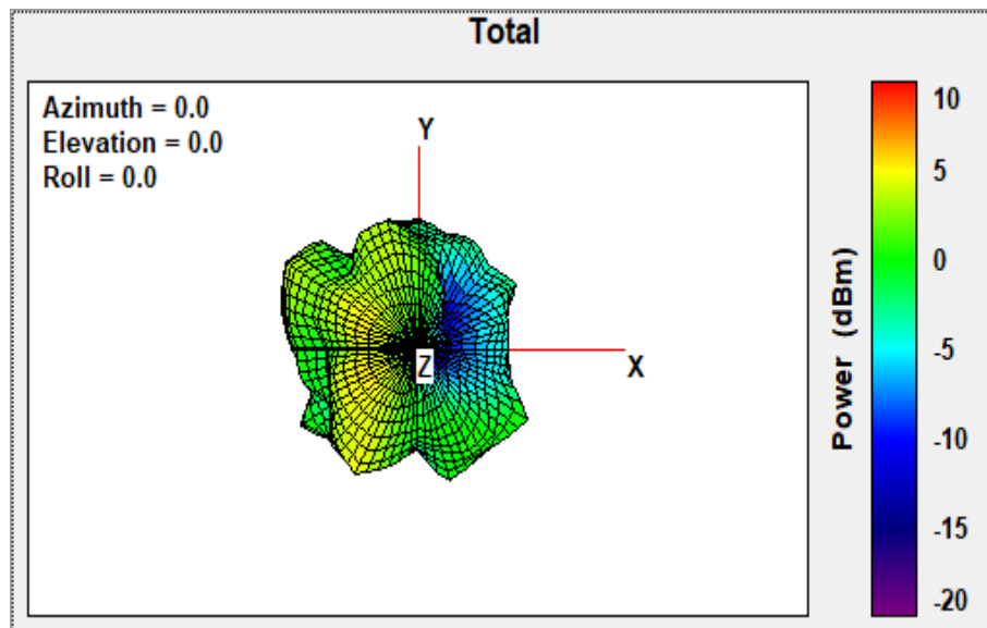
Band 4-5.800GHz X-Y plane View
