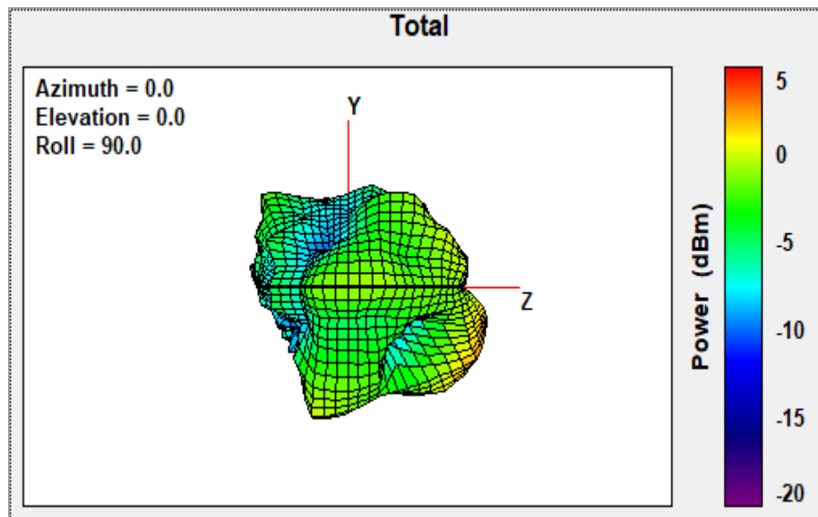
Band 1-5.200GHz Y-Z plane View
