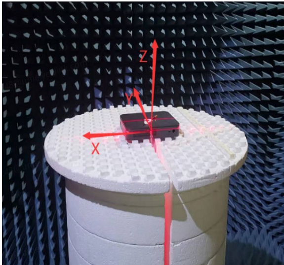
Physical object layout (with coordinate axis)
