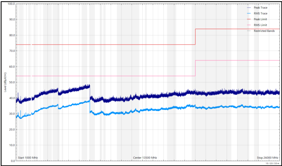
Figure 60 - 2475 MHz (CH25), Thread, iPA, Core 0, 1 GHz to 26 GHz, Horizontal
