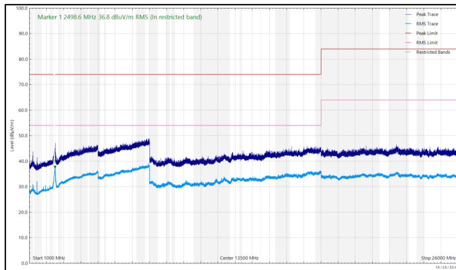
Figure 44 - 2475 MHz (CH25), Thread, ePA, Core 0, 1 GHz to 26 GHz, Horizontal
