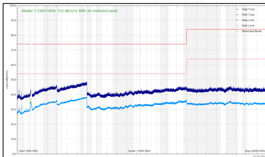
Figure 38 - 2405 MHz (CH11), Thread, ePA, Core 0, 1 GHz to 26 GHz, Horizontal
