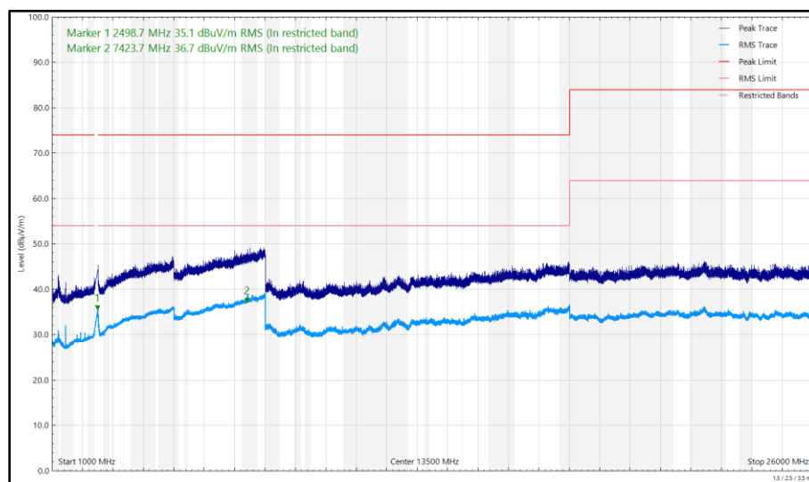
Figure 52 - 2475 MHz (CH25), Thread, ePA, Core 1, 1 GHz to 26 GHz, Horizontal
