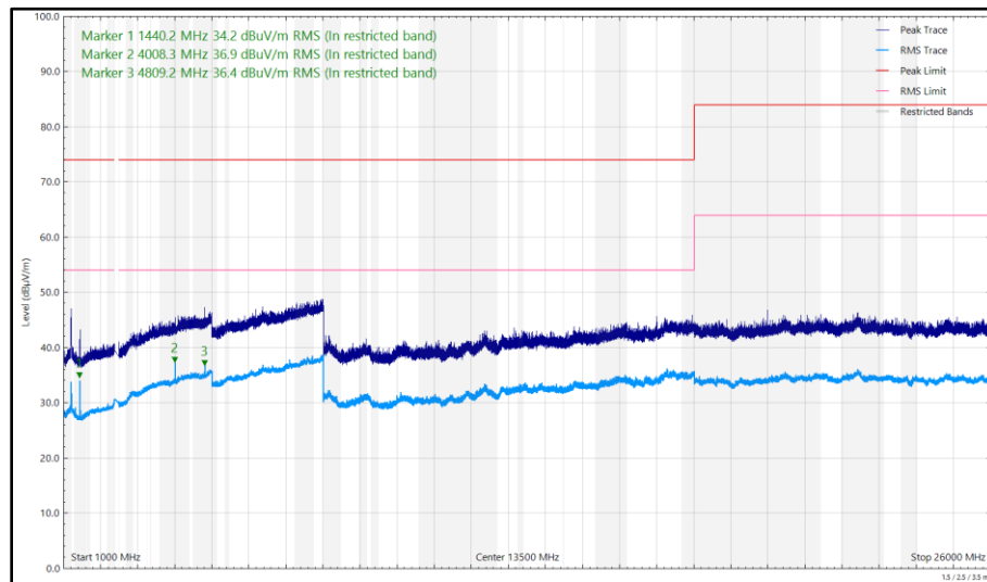
Figure 63 - 2405 MHz (CH11), Thread, iPA, Core 1, 1 GHz to 26 GHz, Vertical
