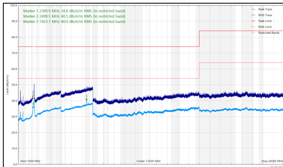
Figure 53 - 2475 MHz (CH25), Thread, ePA, Core 1, 1 GHz to 26 GHz, Vertical
