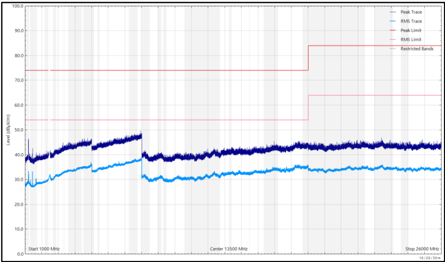
Figure 61 - 2475 MHz (CH25), Thread, iPA, Core 0, 1 GHz to 26 GHz, Vertical
