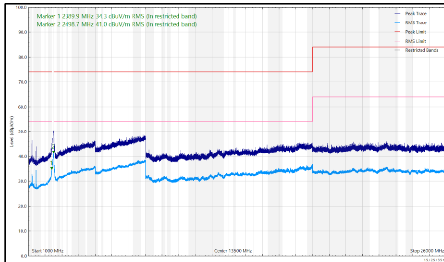
Figure 45 - 2475 MHz (CH25), Thread, ePA, Core 0, 1 GHz to 26 GHz, Vertical
