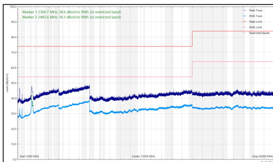
Figure 39 - 2405 MHz (CH11), Thread, ePA, Core 0, 1 GHz to 26 GHz, Vertical
