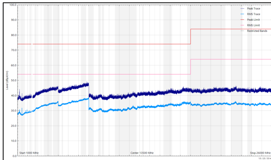
Figure 62 - 2405 MHz (CH11), Thread, iPA, Core 1, 1 GHz to 26 GHz, Horizontal
