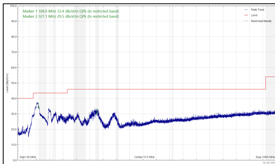
Figure 64 - 2440 MHz (CH18), Thread, iPA, Core 1, 30 MHz to 1 GHz, Horizontal (Peak)
