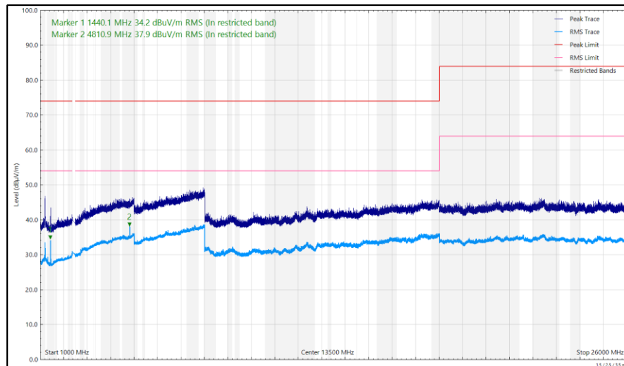
Figure 55 - 2405 MHz (CH11), Thread, iPA, Core 0, 1 GHz to 26 GHz, Vertical
