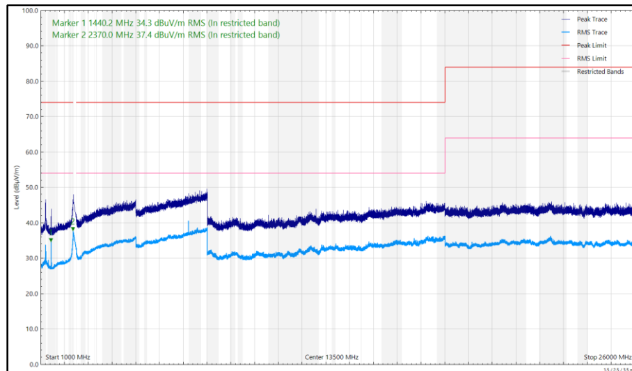
Figure 47 - 2405 MHz (CH11), Thread, ePA, Core 1, 1 GHz to 26 GHz, Vertical
