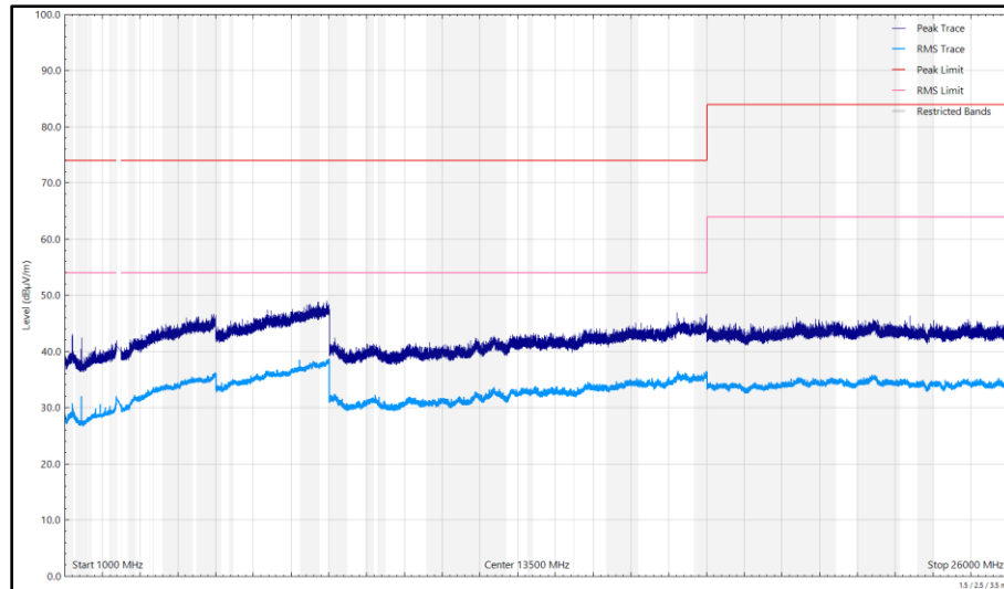
Figure 46 - 2405 MHz (CH11), Thread, ePA, Core 1, 1 GHz to 26 GHz, Horizontal
