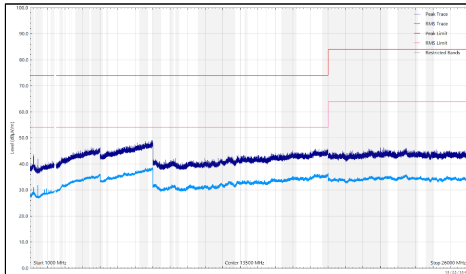
Figure 54 - 2405 MHz (CH11), Thread, iPA, Core 0, 1 GHz to 26 GHz, Horizontal
