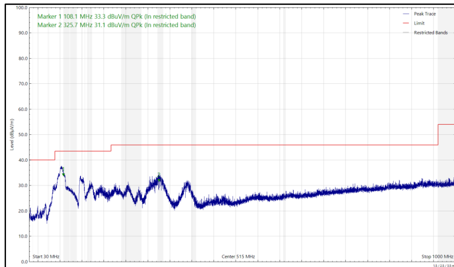
Figure 40 - 2440 MHz (CH18), Thread, ePA, Core 0, 30 MHz to 1 GHz, Horizontal (Peak)
