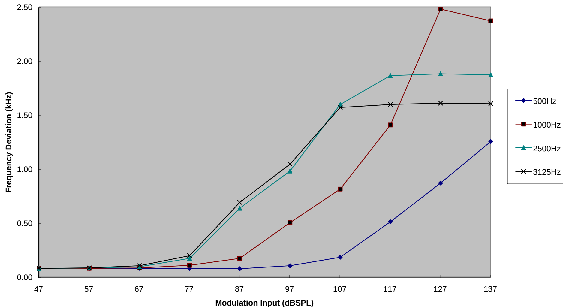
Modulation Limiting Characteristic (T5950)
