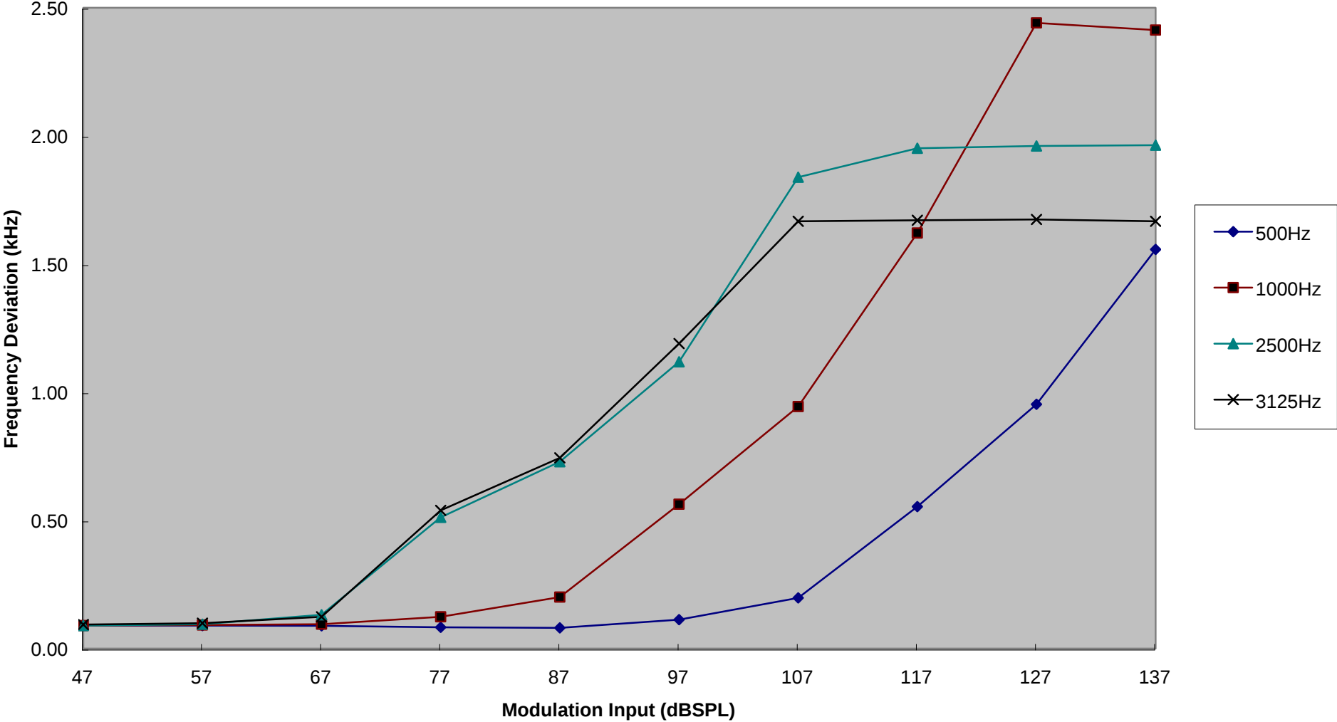
Modulation Limiting Characteristic (T5900)
