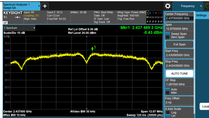
11B-SISO Ant2 2437
