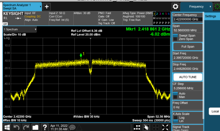
11N40MIMO Ant2 2422
