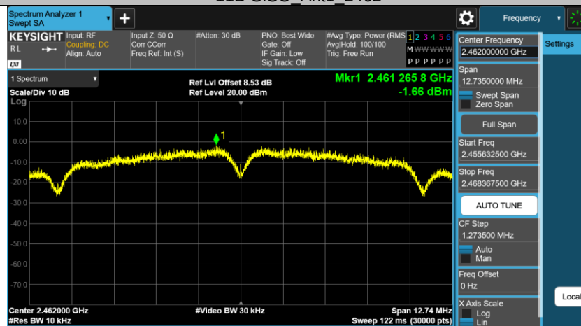
11B-SISO Ant2 2462
