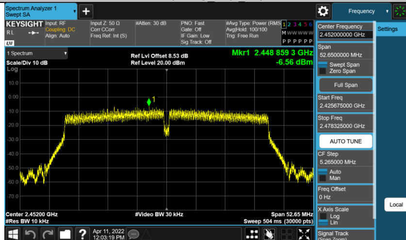
11N40MIMO Ant2 2452
