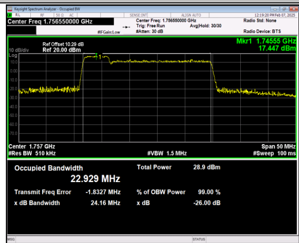
66-66-5MHz-20MHz-16QAM-16QAM-132328-132472-25R B#0-100RB#0-PASS
