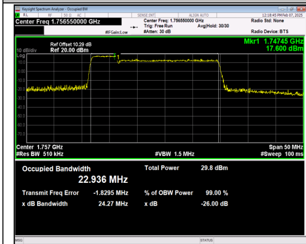
66-66-5MHz-20MHz-QPSK-QPSK-132328-132472-25RB #0-100RB#0-PASS
