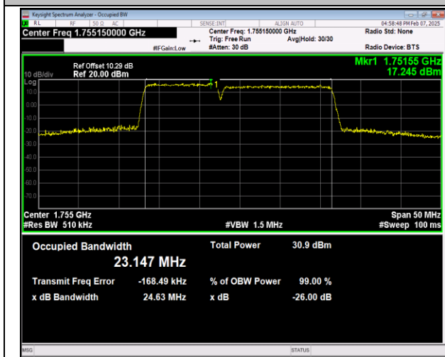
66-66-10MHz-15MHz-QPSK-QPSK-132351-132471-50R B#0-75RB#0-PASS
