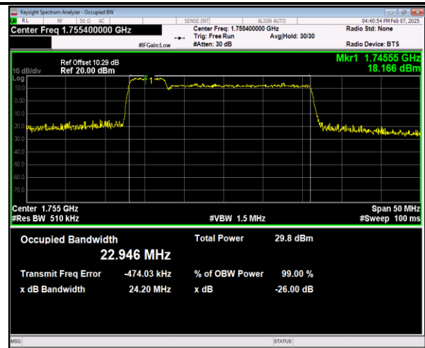
66-66-5MHz-20MHz-16QAM-16QAM-132330-132447-25R B#0-100RB#0-PASS
