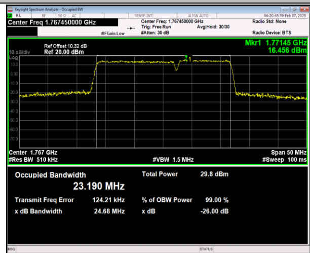
66-66-15MHz-10MHz-16QAM-16QAM-132499-132619-75R B#0-50RB#0-PASS
