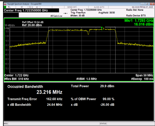
66-66-15MHz-10MHz-16QAM-16QAM-132047-132167-75R B#0-50RB#0-PASS
