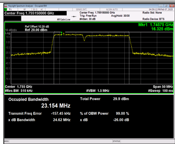
66-66-10MHz-15MHz-16QAM-16QAM-132351-132471-50R B#0-75RB#0-PASS
