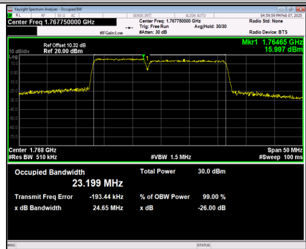
66-66-10MHz-15MHz-16QAM-16QAM-132477-132597-50R B#0-75RB#0-PASS
