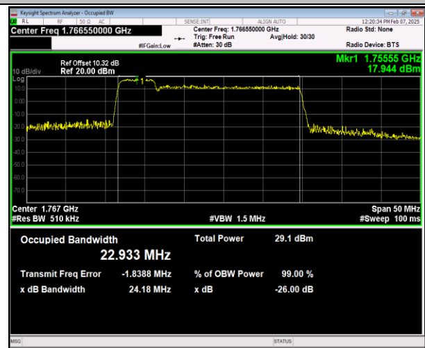
66-66-5MHz-20MHz-16QAM-16QAM-132428-132572-25R B#0-100RB#0-PASS
