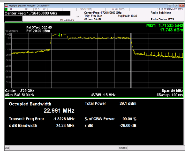
66-66-5MHz-20MHz-16QAM-16QAM-132027-132171-25R B#0-100RB#0-PASS
