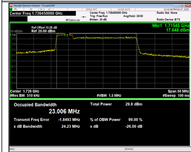
66-66-5MHz-20MHz-QPSK-QPSK-132027-132171-25RB #0-100RB#0-PASS
