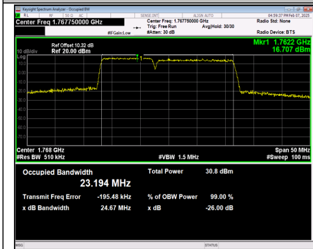
66-66-10MHz-15MHz-QPSK-QPSK-132477-132597-50R B#0-75RB#0-PASS
