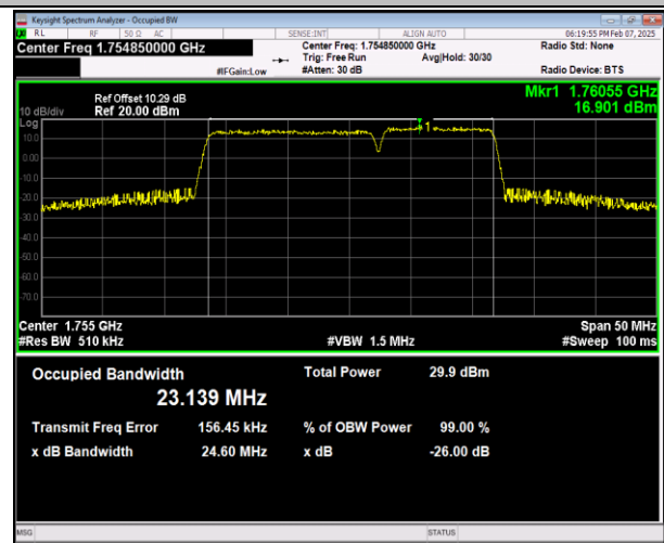
66-66-15MHz-10MHz-16QAM-16QAM-132373-132493-75R B#0-50RB#0-PASS
