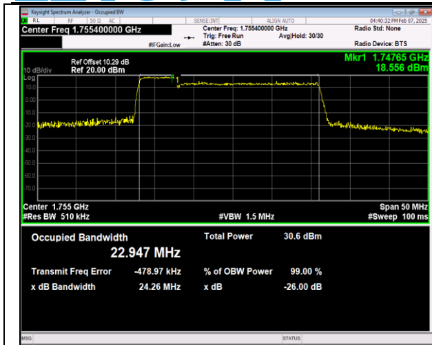
66-66-5MHz-20MHz-QPSK-QPSK-132330-132447-25RB #0-100RB#0-PASS
