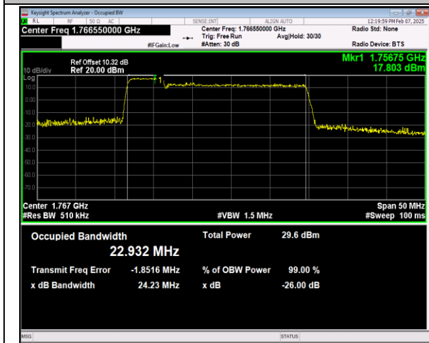
66-66-5MHz-20MHz-QPSK-QPSK-132428-132572-25RB #0-100RB#0-PASS
