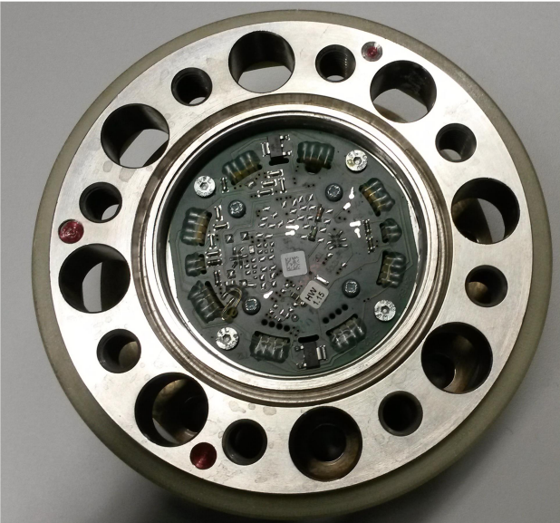
The rotor includes 4 PCB
