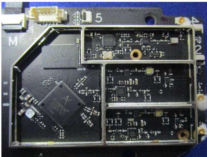
EUT –RF Circuit View
