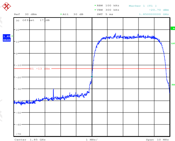
Lower Band Edge Plot on Channel 9262
