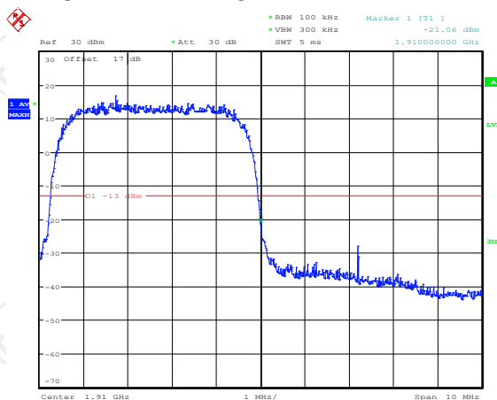
Higher Band Edge Plot on Channel 9538
