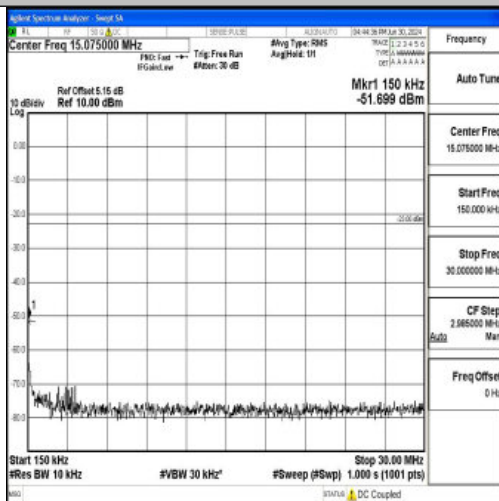
Band12_5MHz_QPSK_23095_1RB#0_0.15~30_0.15~30
