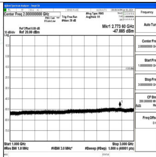
Band12_10MHz_QPSK_23060_1RB#0_1000~3000_1000~3000
