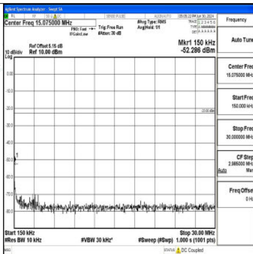
Band12_10MHz_16QAM_23060_1RB#0_0.15~30_0.15~30
