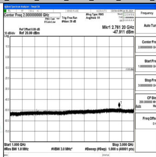
Band12_1.4MHz_16QAM_23173_1RB#0_1000~3000_1000~3000
