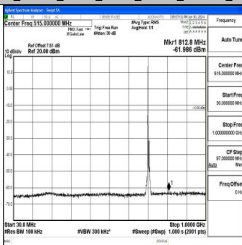
Band12_10MHz_QPSK_23130_1RB#0_30~1000_30~1000
