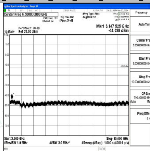
Band12_3MHz_QPSK_23025_1RB#0_3000~10000_3000~10000
