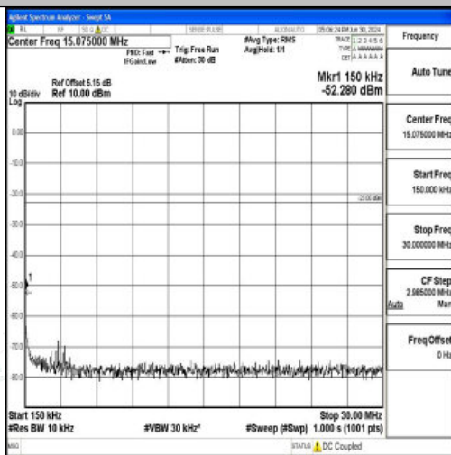
Band12_10MHz_16QAM_23095_1RB#0_0.15~30_0.15~30
