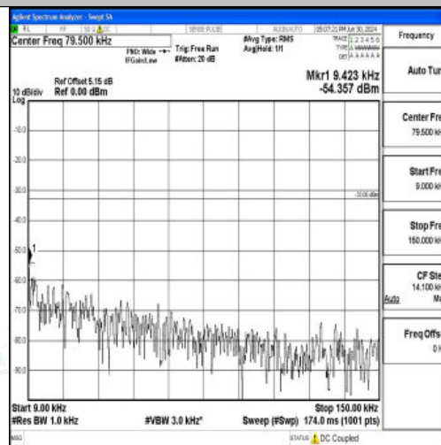
Band12_10MHz_16QAM_23130_1RB#0_0.009~0.15_0.009~0.15
