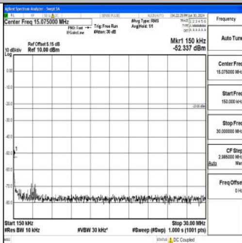
Band12_3MHz_QPSK_23095_1RB#0_0.15~30_0.15~30
