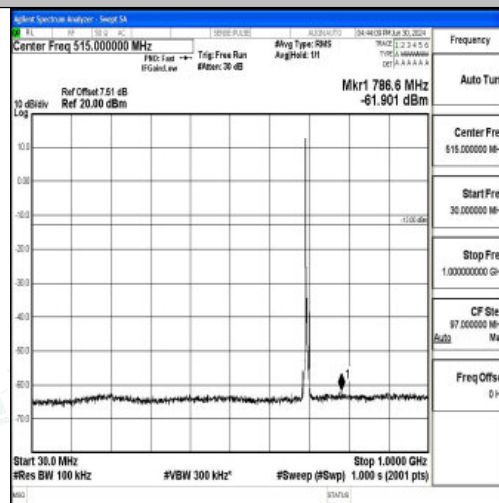
Band12_5MHz_16QAM_23035_1RB#0_30~1000_30~1000
