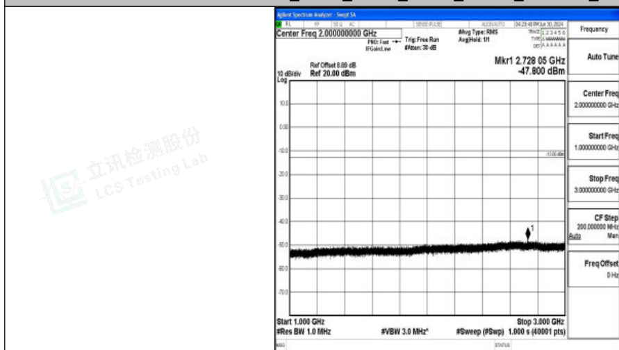
Band12_3MHz_QPSK_23165_1RB#0_1000~3000_1000~3000
