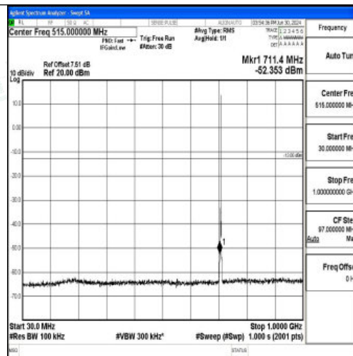
Band12_1.4MHz_16QAM_23173_1RB#0_30~1000_30~1000
