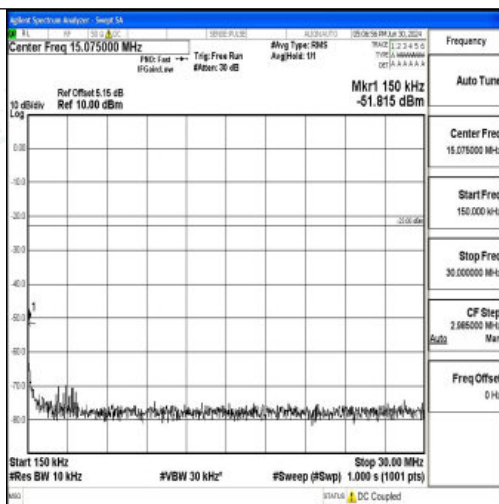
Band12_10MHz_QPSK_23130_1RB#0_0.15~30_0.15~30
