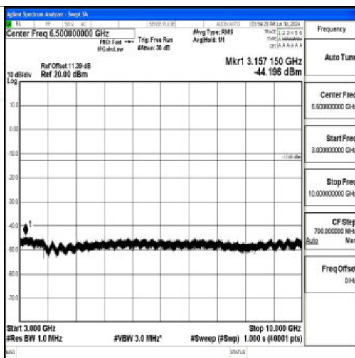
Band12_1.4MHz_QPSK_23173_1RB#0_3000~10000_3000~10000
