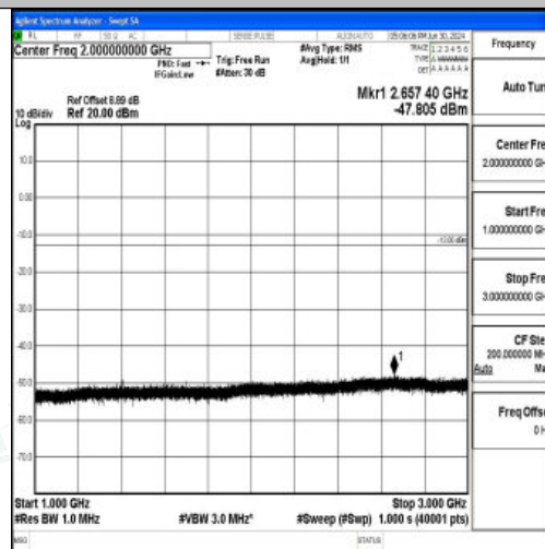
Band12_10MHz_QPSK_23095_1RB#0_1000~3000_1000~3000
