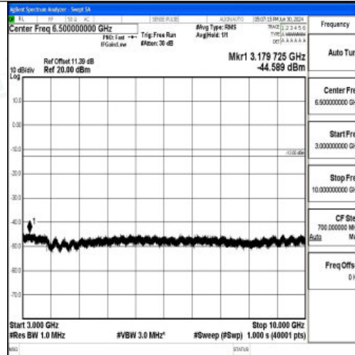
Band12_10MHz_QPSK_23130_1RB#0_3000~10000_3000~10000
