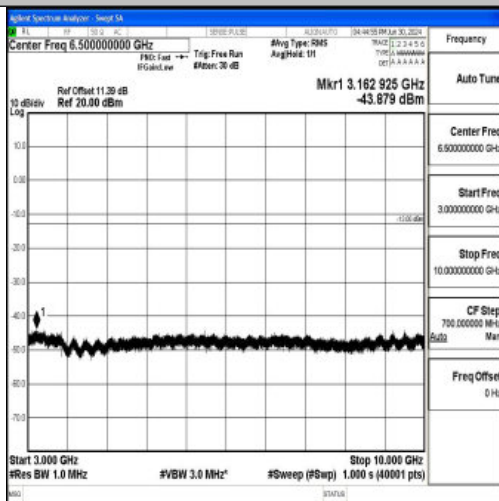
Band12_5MHz_QPSK_23095_1RB#0_3000~10000_3000~10000
