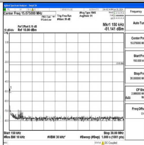
Band12_5MHz_QPSK_23035_1RB#0_0.15~30_0.15~30
