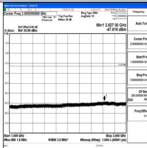
Band12_10MHz_16QAM_23130_1RB#0_1000~3000_1000~3000
