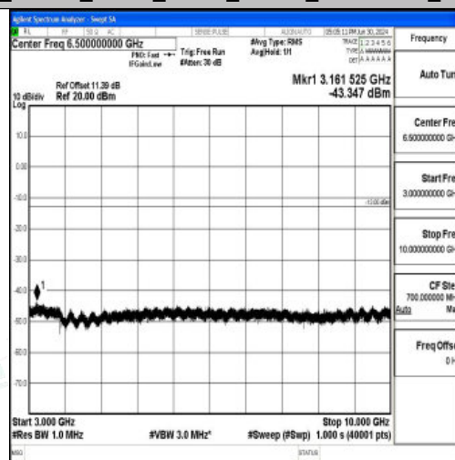
Band12_10MHz_QPSK_23060_1RB#0_3000~10000_3000~10000
