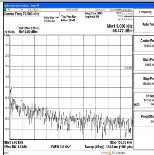
Band12_5MHz_16QAM_23035_1RB#0_0.009~0.15_0.009~0.15
