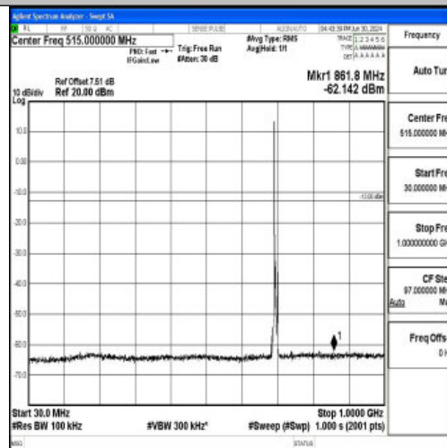
Band12_5MHz_QPSK_23035_1RB#0_30~1000_30~1000
