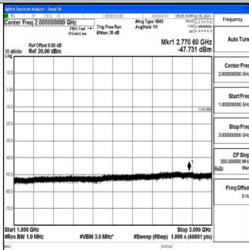
Band12_10MHz_16QAM_23060_1RB#0_1000~3000_1000~3000
