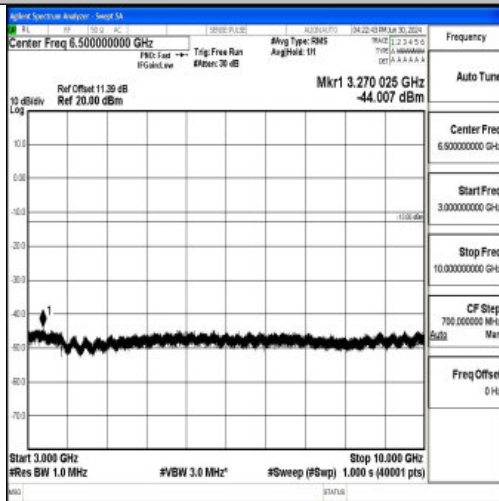
Band12_3MHz_QPSK_23095_1RB#0_3000~10000_3000~10000
