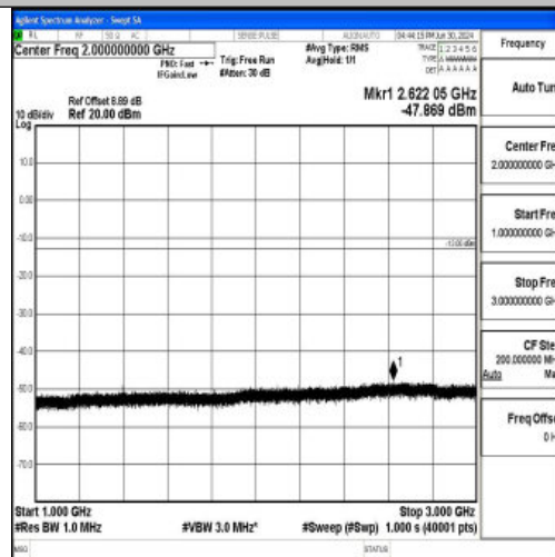
Band12_5MHz_16QAM_23035_1RB#0_1000~3000_1000~3000
