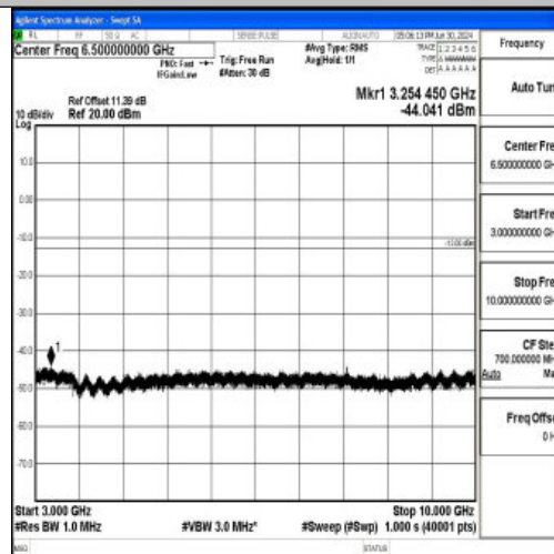
Band12_10MHz_QPSK_23095_1RB#0_3000~10000_3000~10000
