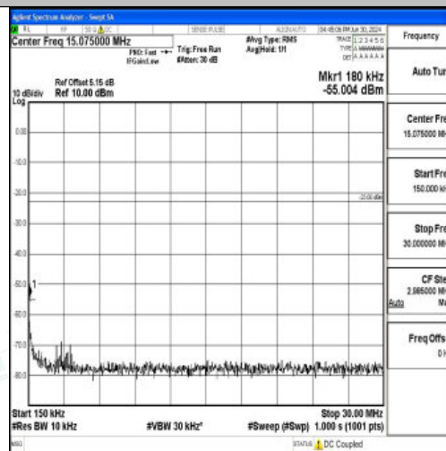
Band12_5MHz_16QAM_23095_1RB#0_0.15~30_0.15~30
