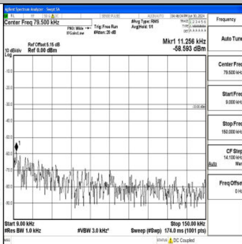
Band12_5MHz_16QAM_23155_1RB#0_0.009~0.15_0.009~0.15
