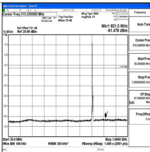
Band12_3MHz_16QAM_23165_1RB#0_30~1000_30~1000
