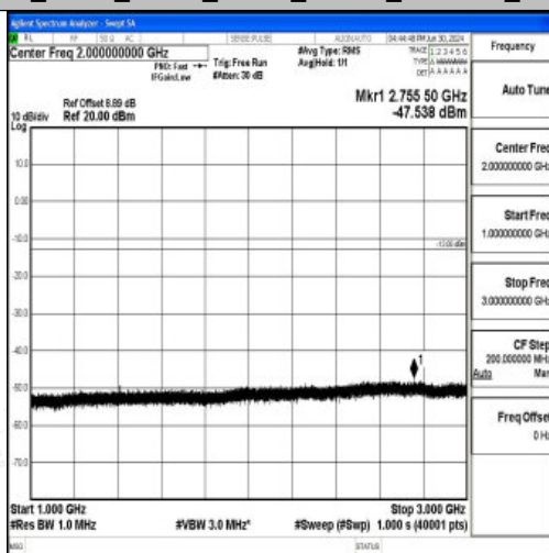
Band12_5MHz_QPSK_23095_1RB#0_1000~3000_1000~3000
