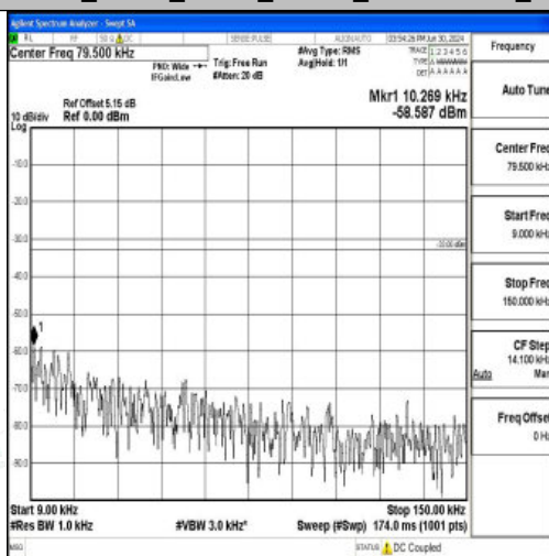
Band12_1.4MHz_16QAM_23173_1RB#0_0.009~0.15_0.009~0.15
