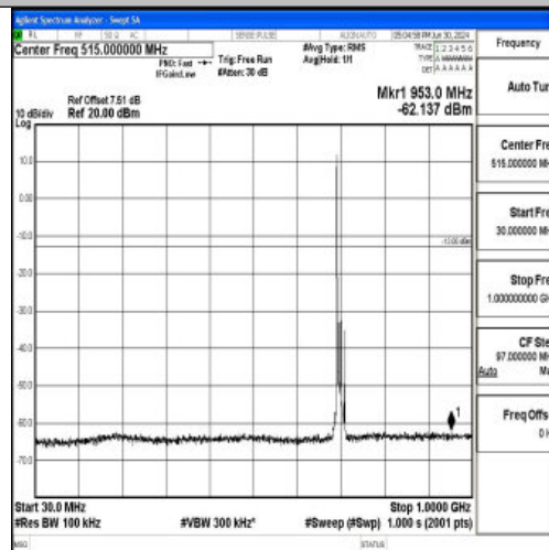
Band12_10MHz_QPSK_23060_1RB#0_30~1000_30~1000
