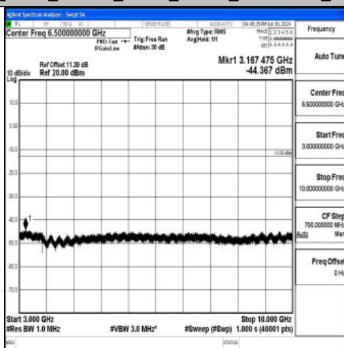
Band12_5MHz_16QAM_23095_1RB#0_3000~10000_3000~10000
