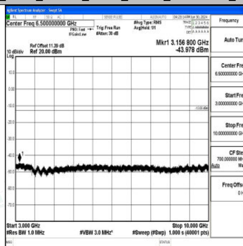
Band12_3MHz_16QAM_23095_1RB#0_3000~10000_3000~10000
