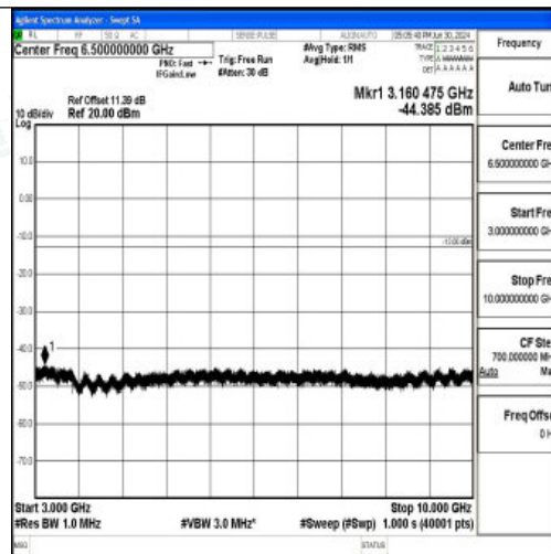
Band12_10MHz_16QAM_23060_1RB#0_3000~10000_3000~10000
