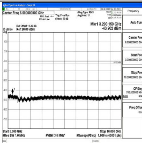
Band12_5MHz_16QAM_23155_1RB#0_3000~10000_3000~10000
