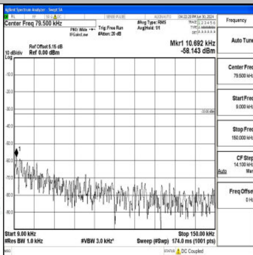
Band12_3MHz_QPSK_23095_1RB#0_0.009~0.15_0.009~0.15
