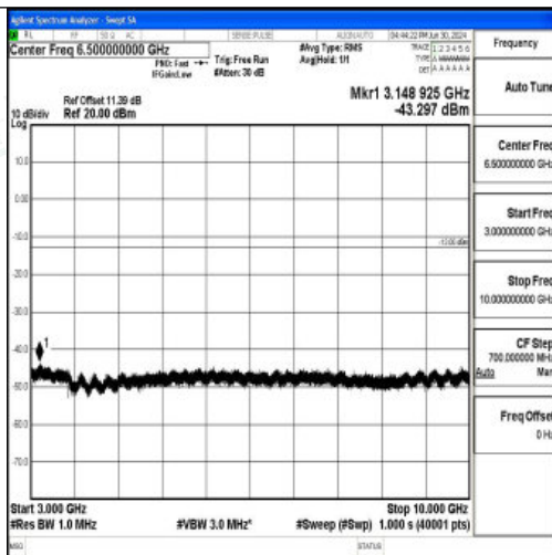
Band12_5MHz_16QAM_23035_1RB#0_3000~10000_3000~10000
