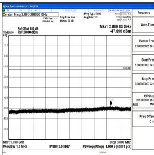
Band12_5MHz_16QAM_23095_1RB#0_1000~3000_1000~3000
