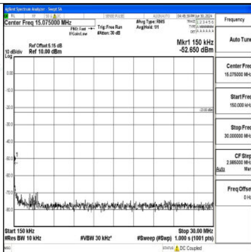
Band12_5MHz_QPSK_23155_1RB#0_0.15~30_0.15~30
