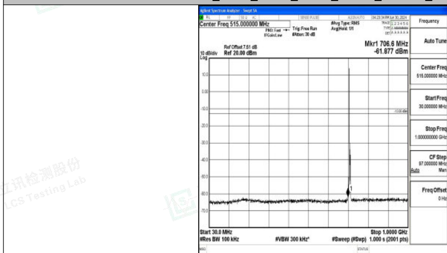
Band12_3MHz_QPSK_23165_1RB#0_30~1000_30~1000
