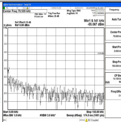
Band12_3MHz_16QAM_23165_1RB#0_0.009~0.15_0.009~0.15
