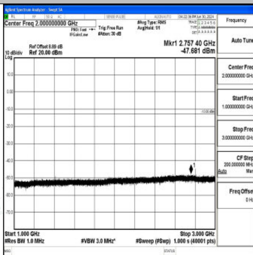
Band12_3MHz_QPSK_23095_1RB#0_1000~3000_1000~3000
