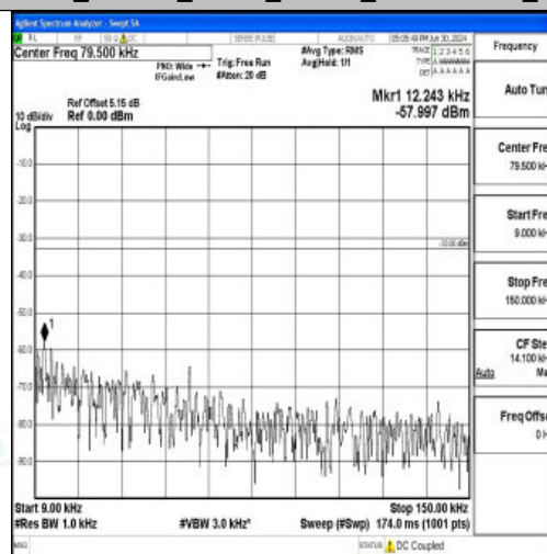
Band12_10MHz_QPSK_23095_1RB#0_0.009~0.15_0.009~0.15
