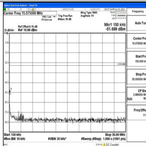
Band12_10MHz_16QAM_23130_1RB#0_0.15~30_0.15~30
