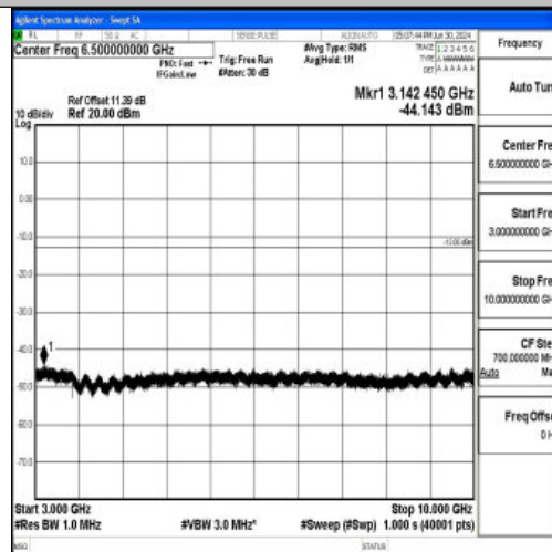
Band12_10MHz_16QAM_23130_1RB#0_3000~10000_3000~10000
