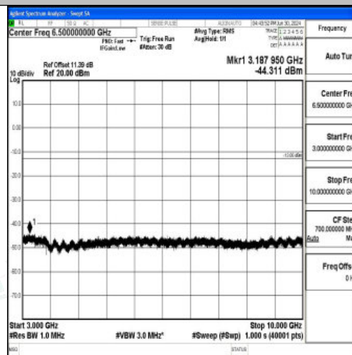
Band12_5MHz_QPSK_23035_1RB#0_3000~10000_3000~10000
