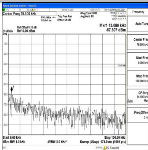
Band12_5MHz_QPSK_23095_1RB#0_0.009~0.15_0.009~0.15
