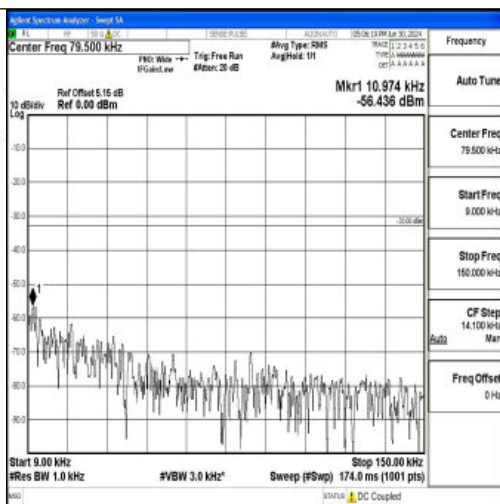
Band12_10MHz_16QAM_23095_1RB#0_0.009~0.15_0.009~0.15
