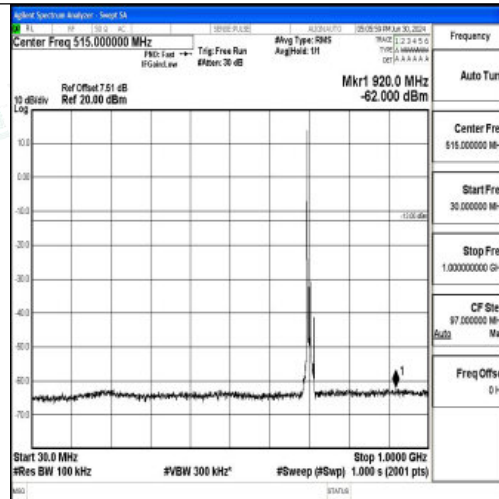
Band12_10MHz_QPSK_23095_1RB#0_30~1000_30~1000
