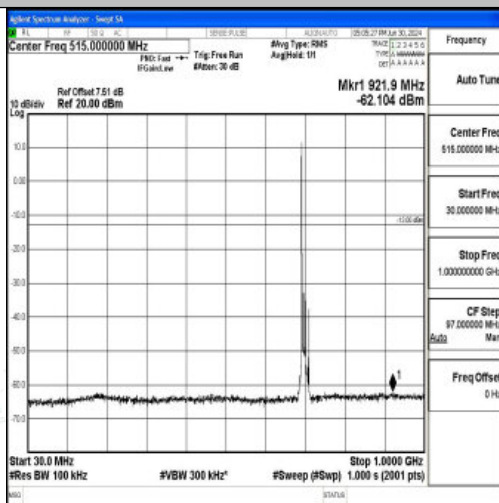
Band12_10MHz_16QAM_23060_1RB#0_30~1000_30~1000
