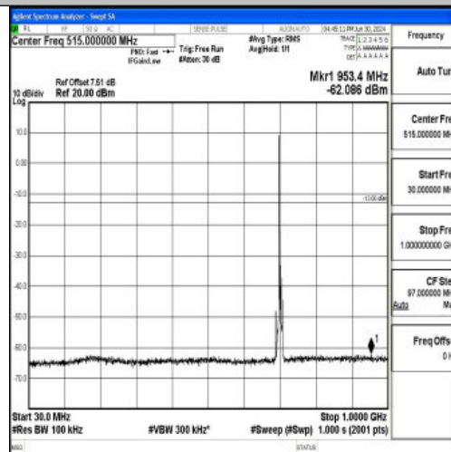
Band12_5MHz_16QAM_23095_1RB#0_30~1000_30~1000
