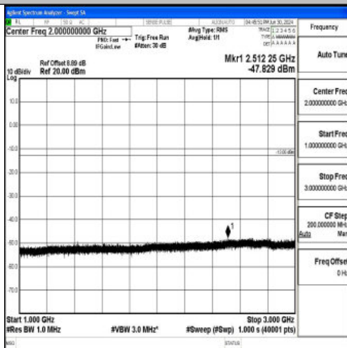
Band12_5MHz_QPSK_23155_1RB#0_1000~3000_1000~3000
