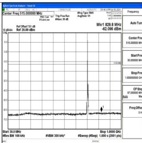
Band12_5MHz_16QAM_23155_1RB#0_30~1000_30~1000
