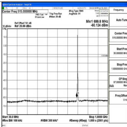
Band12_3MHz_QPSK_23095_1RB#0_30~1000_30~1000
