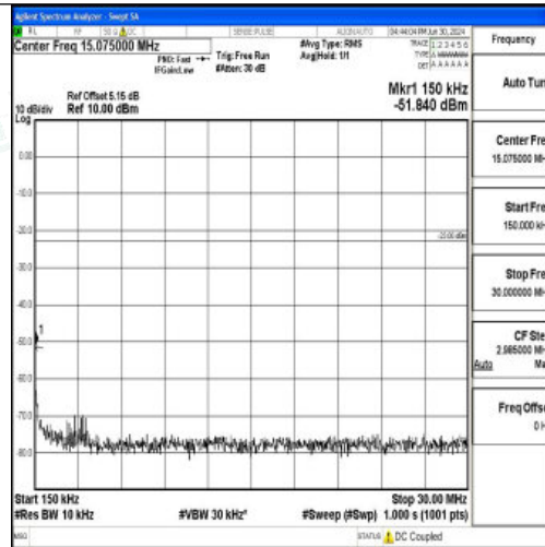
Band12_5MHz_16QAM_23035_1RB#0_0.15~30_0.15~30
