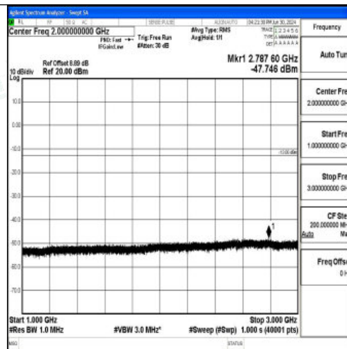
Band12_3MHz_QPSK_23025_1RB#0_1000~3000_1000~3000
