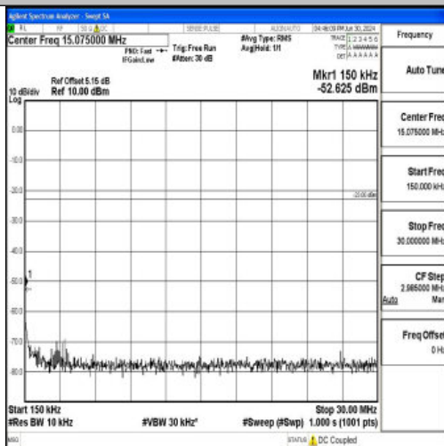
Band12_5MHz_16QAM_23155_1RB#0_0.15~30_0.15~30
