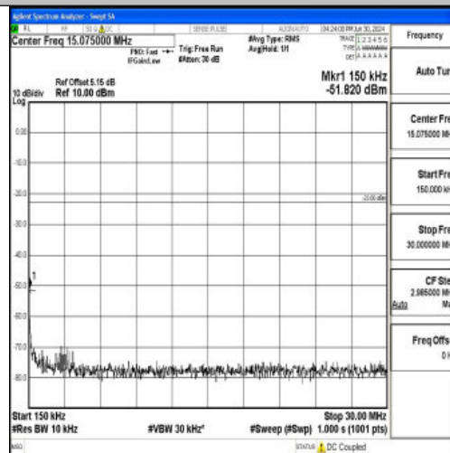
Band12_3MHz_16QAM_23165_1RB#0_0.15~30_0.15~30
