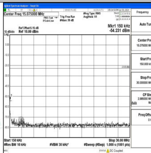
Band12_10MHz_QPSK_23060_1RB#0_0.15~30_0.15~30
