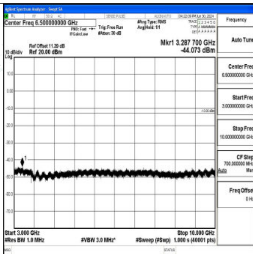
Band12_3MHz_16QAM_23025_1RB#0_3000~10000_3000~10000
