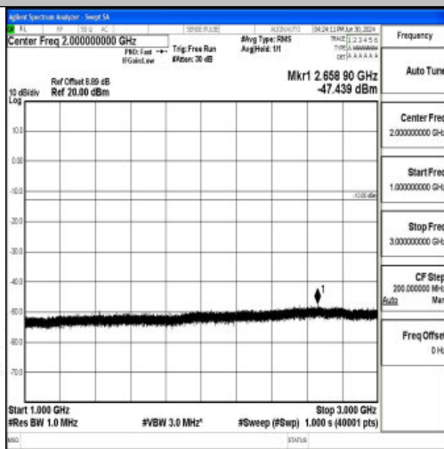
Band12_3MHz_16QAM_23165_1RB#0_1000~3000_1000~3000
