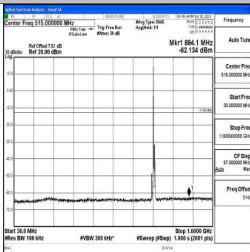
Band12_5MHz_QPSK_23155_1RB#0_30~1000_30~1000
