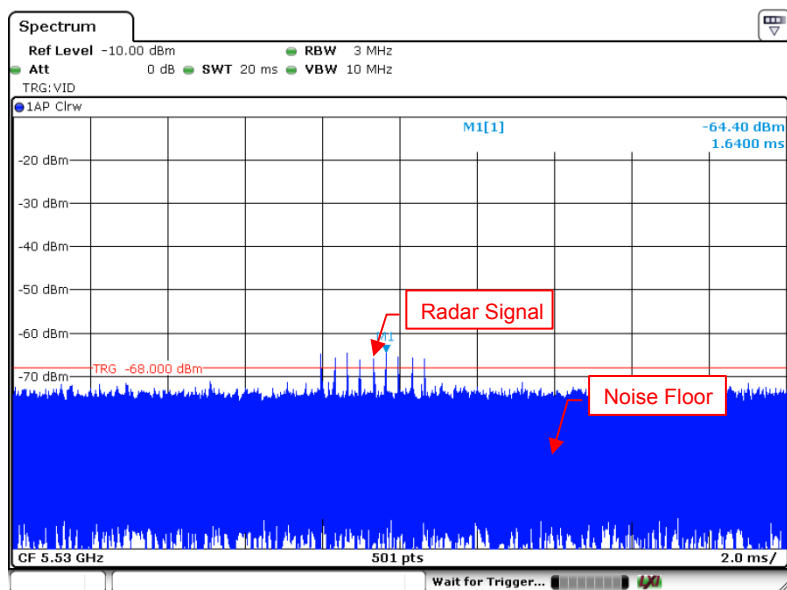
Radar Signal 6
