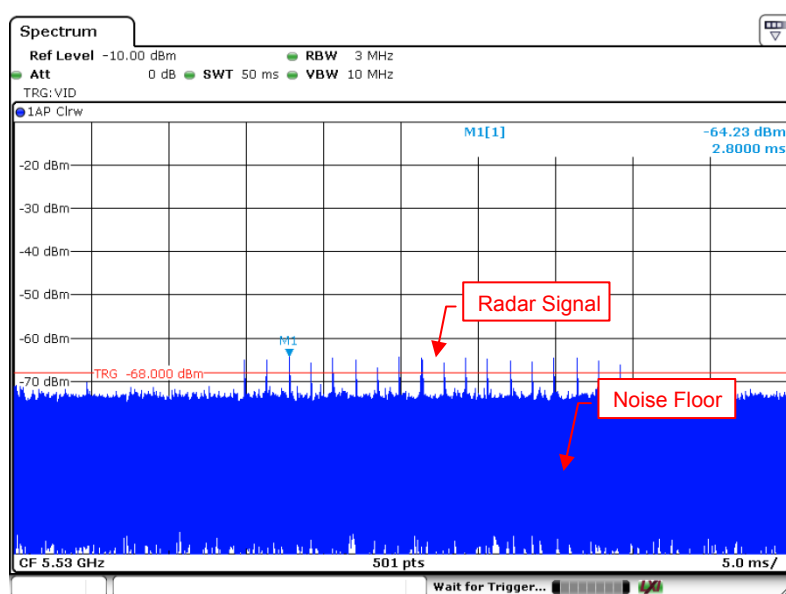
Radar Signal 0
