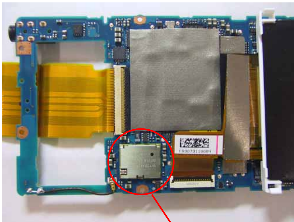
WLAN Module "WY5BAKSX2-A" manufactured by Taiyo Yuden
