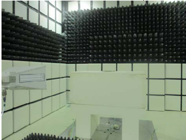
Part_22_24_GSM_Radiated_E2_Setup
