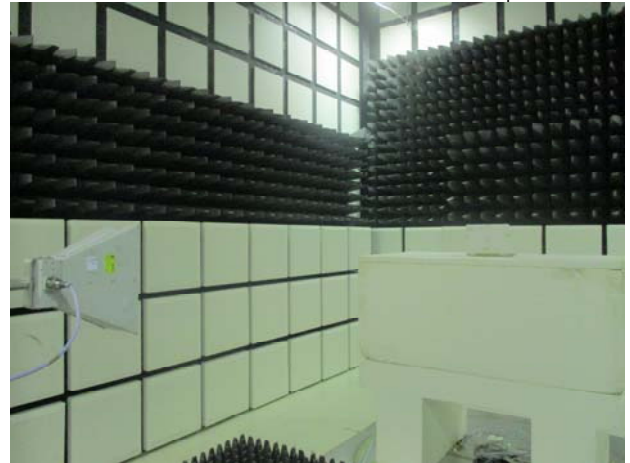
Part_22_24_27_Cat M1_Radiated_NB_Setup
