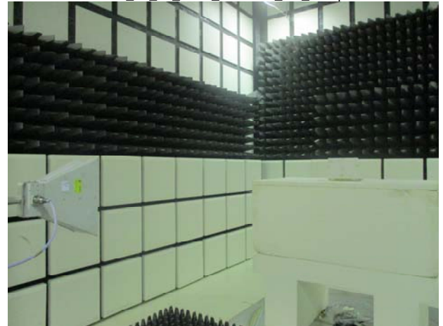
Part_22_24_GSM_Radiated_NB_Setup
