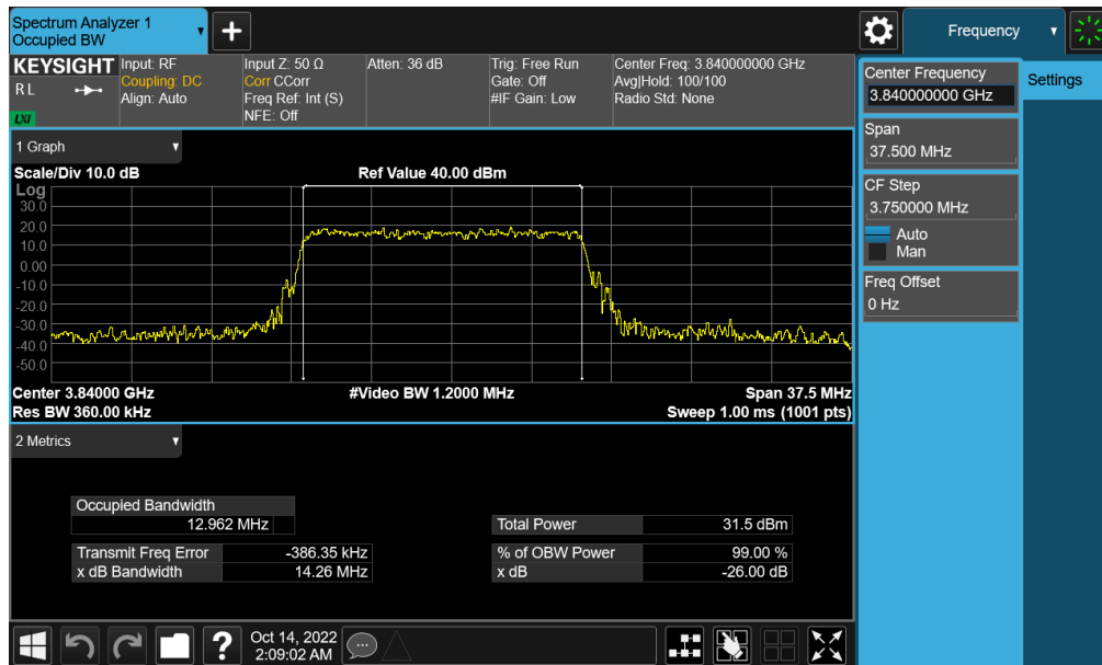
Plot 7-67. Occupied Bandwidth Plot (NR Band n77 - C-Band – 15MHz – \pi/2 BPSK - Full RB)
