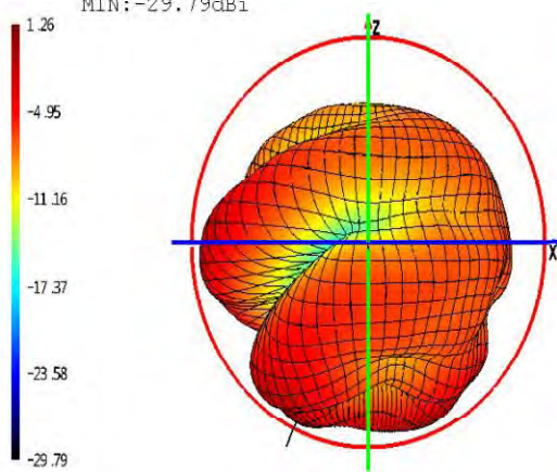
Phi=0 freq=2480MHz
