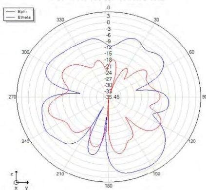
Phi=90 freq=2402MHz
