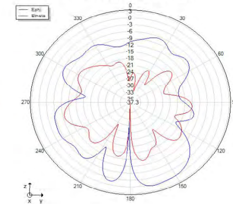
Phi=90 freq=2480MHz
