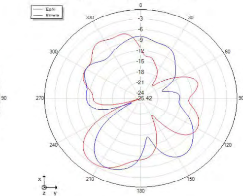
Theta=90 freq=2480MHz
