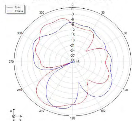
Theta=90 freq=2402MHz
