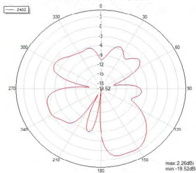
Phi=90 freq=2402MHz
