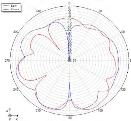
Phi=0 freq=2480MHz
