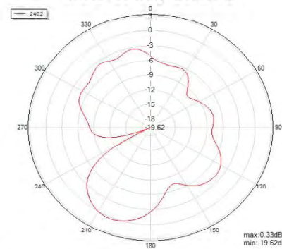
Theta=90 freq=2402MHz
