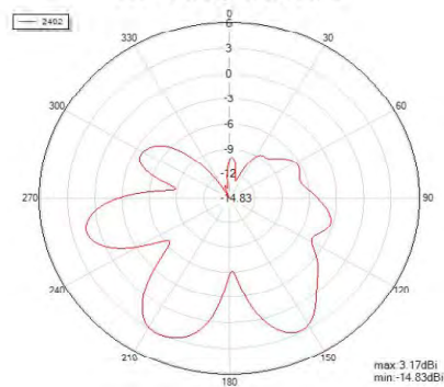
Phi=0 freq=2402MHz
