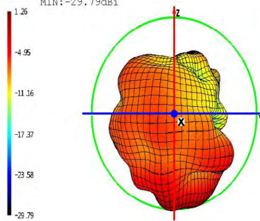
Phi=90 freq=2480MHz
