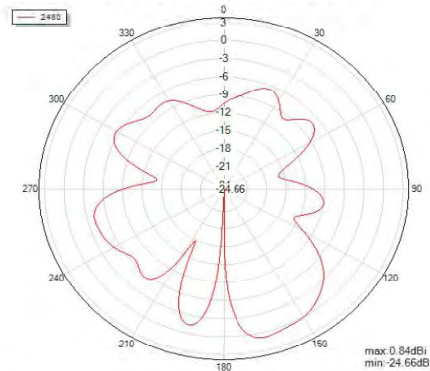
Phi=90 freq=2480MHz
