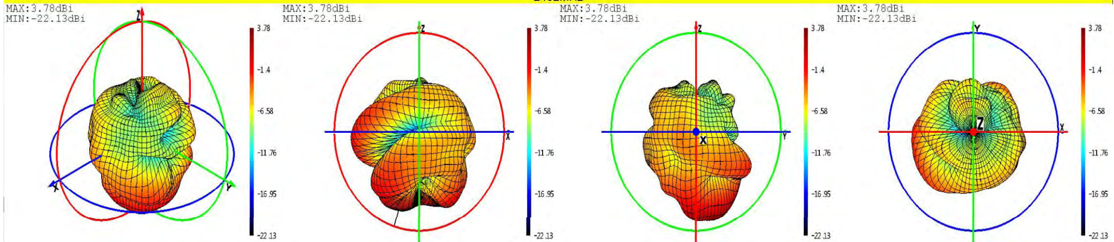
Phi=0 freq=2402MHz
