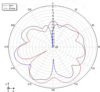
Phi=0 freq=2402MHz
