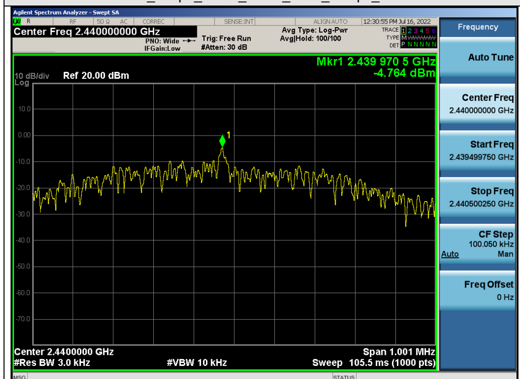
Test_Graph_LE1M_ANT1_2440_1Mbps_PSD
