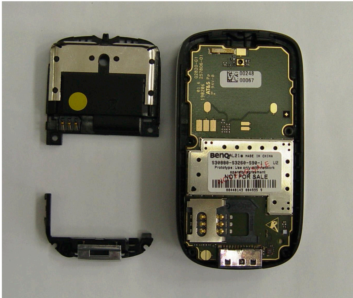
AL21a Disassembly Step 1
