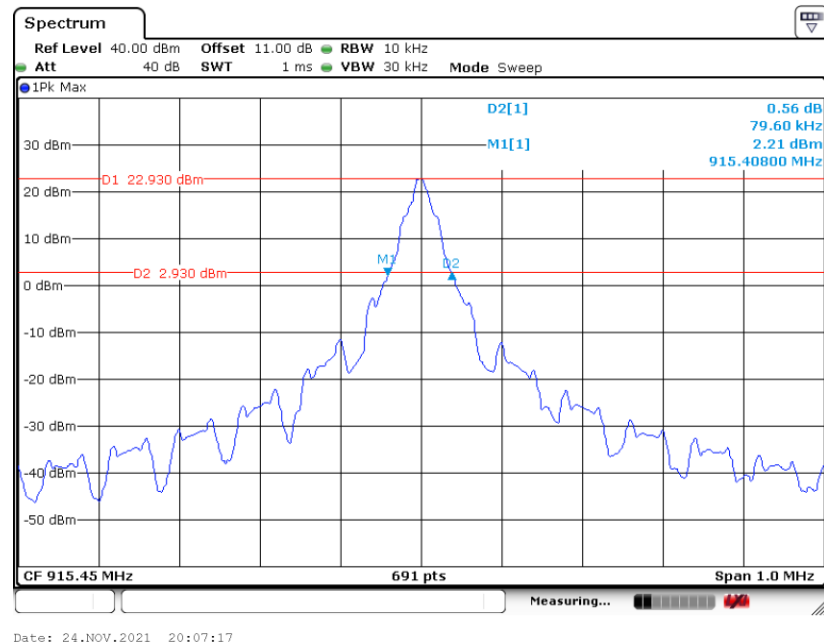
20 dB Bandwidth Plot on 915.45MHz
