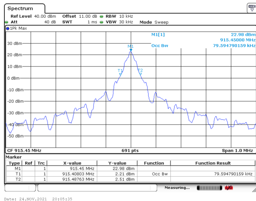
99% Occupied Bandwidth Plot on 915.45MHz
