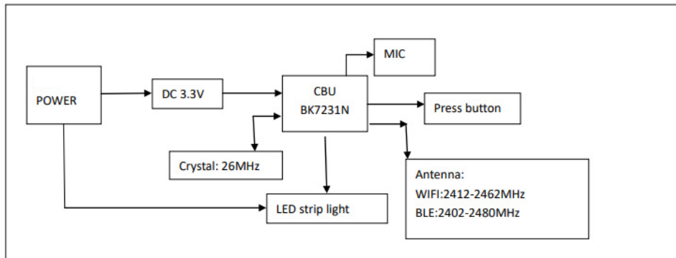
BLOCK DIAGRAM
