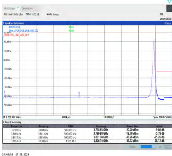
1-N78-3700-3800-PC2-30-90-H-5-CP-QPSK-Edge_1RB_Right-1@244-Ant7-1--PASS-see graph
