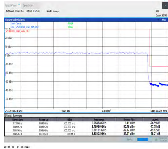
1-N78-3700-3800-PC2-30-80-H-3-DFT-PI2BPSK-Outer_Full-216@0-Ant7-1--PASS-see graph
