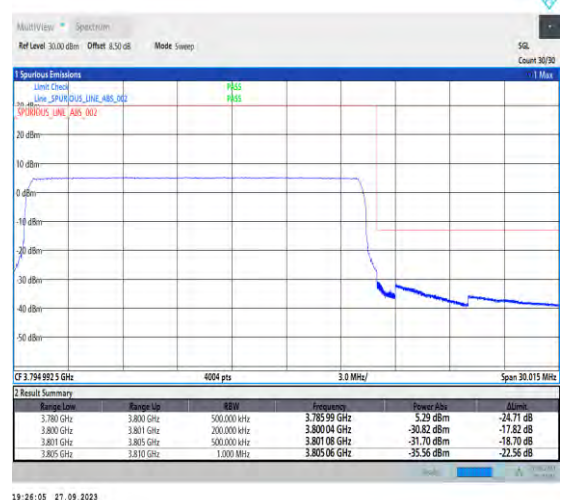
1-N78-3700-3800-PC2-30-20-H-6-CP-QPSK-Outer_Full-51@0-Ant7-1--PASS-see graph
