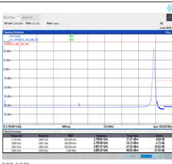
1-N78-3700-3800-PC2-30-90-H-2-DFT-PI2BPSK-Edge_1RB_Right-1@244-Ant7-1--PASS-see graph
