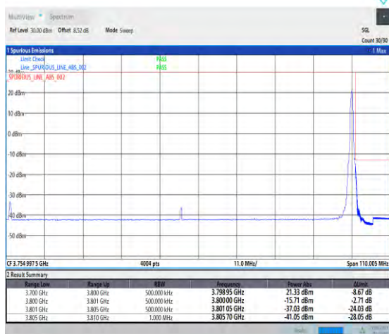
1-N78-3700-3800-PC2-30-100-H-2-DFT-PI2BPSK-Edge_1RB_Right-1@272-Ant7-1--PASS-see graph
