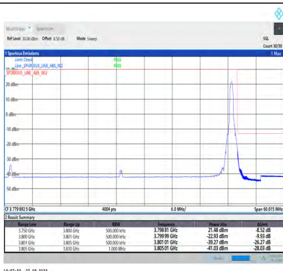
1-N78-3700-3800-PC2-30-50-H-2-DFT-PI2BPSK-Edge_1RB_Right-1@132-Ant7-1--PASS-see graph
