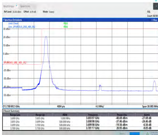
1-N78-3700-3800-PC2-30-30-L-4-CP-QPSK-Edge_1RB_Left-1@0-Ant7-1--PASS-see graph
