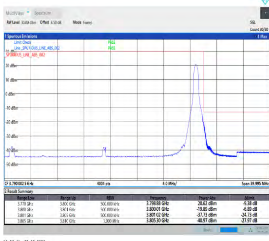
1-N78-3700-3800-PC2-30-30-H-5-CP-QPSK-Edge_1RB_Right-1@77-Ant7-1--PASS-see graph
