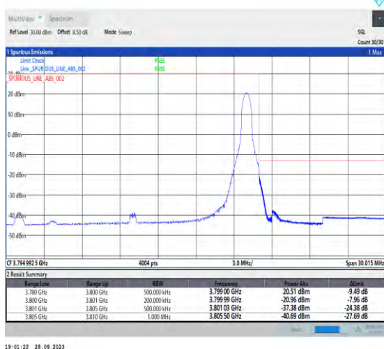
1-N78-3700-3800-PC2-30-20-H-5-CP-QPSK-Edge_1RB_Right-1@50-Ant7-1--PASS-see graph
