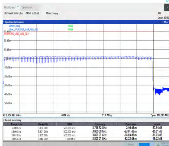
1-N78-3700-3800-PC2-30-100-H-3-DFT-PI2BPSK-Outer_Full-270@0-Ant7-1--PASS-see graph
