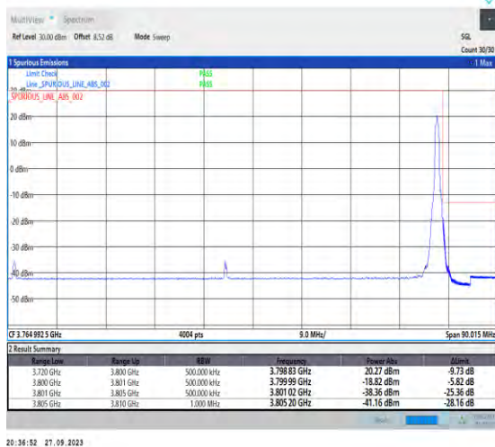
1-N78-3700-3800-PC2-30-80-H-5-CP-QPSK-Edge_1RB_Right-1@216-Ant7-1--PASS-see graph
