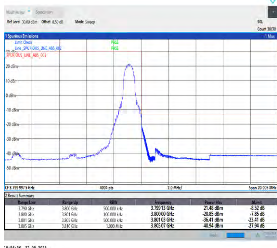
1-N78-3700-3800-PC2-30-10-H-2-DFT-PI2BPSK-Edge_1RB_Right-1@23-Ant7-1--PASS-see graph
