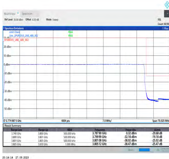
1-N78-3700-3800-PC2-30-60-H-6-CP-QPSK-Outer_Full-162@0-Ant7-1--PASS-see graph
