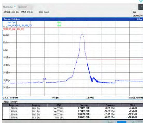
1-N78-3700-3800-PC2-30-15-H-5-CP-QPSK-Edge_1RB_Right-1@37-Ant7-1--PASS-see graph
