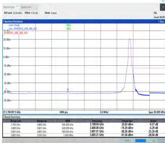
1-N78-3700-3800-PC2-30-40-H-5-CP-QPSK-Edge_1RB_Right-1@105-Ant7-1--PASS-see graph
