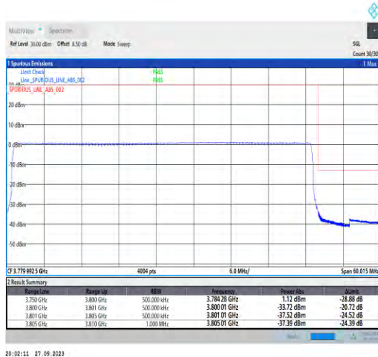
1-N78-3700-3800-PC2-30-50-H-6-CP-QPSK-Outer_Full-133@0-Ant7-1--PASS-see graph
