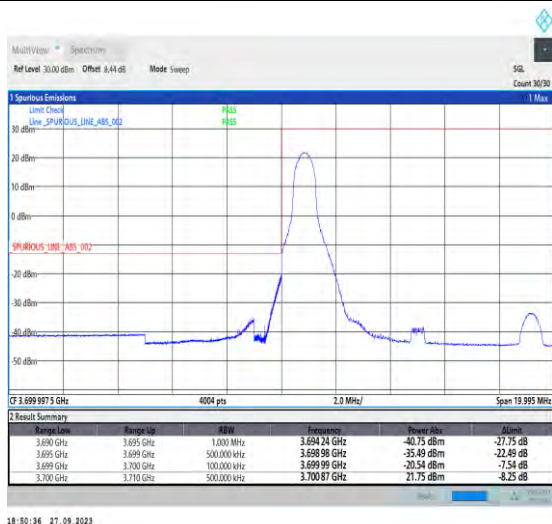
1-N78-3700-3800-PC2-30-10-L-1-DFT-PI2BPSK-Edge_1RB_Left-1@0-Ant7-1--PASS-see graph
