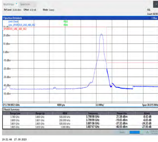
1-N78-3700-3800-PC2-30-20-H-2-DFT-PI2BPSK-Edge_1RB_Right-1@50-Ant7-1--PASS-see graph
