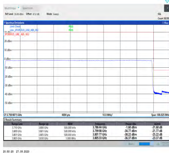
1-N78-3700-3800-PC2-30-90-H-6-CP-QPSK-Outer_Full-245@0-Ant7-1--PASS-see graph
