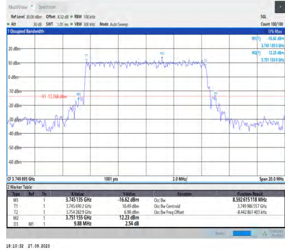
1-N78-3700-3800-PC2-30-10-M-2-DFT-PI2BPSK-Ou ter_Full-24@0-Ant7-8.593-9.880-≤10-PASS
