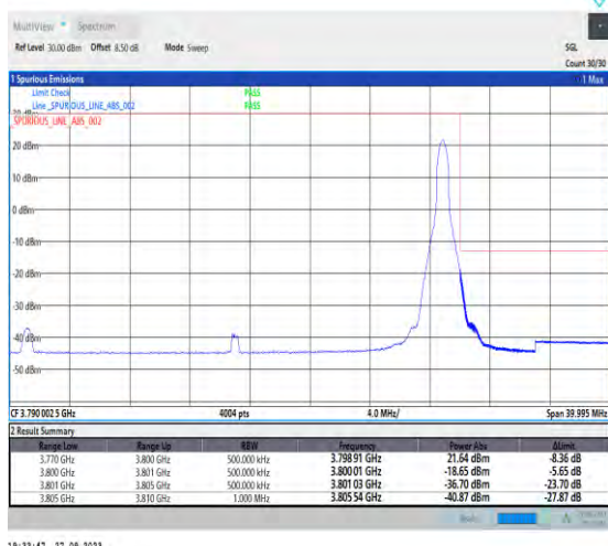
1-N78-3700-3800-PC2-30-30-H-2-DFT-PI2BPSK-Edge_1RB_Right-1@77-Ant7-1--PASS-see graph
