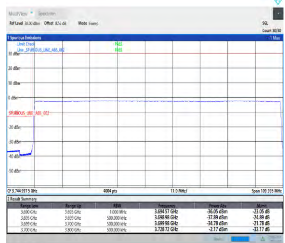
1-N78-3700-3800-PC2-30-100-L-6-CP-QPSK-Outer_Full-273@0-Ant7-1--PASS-see graph
