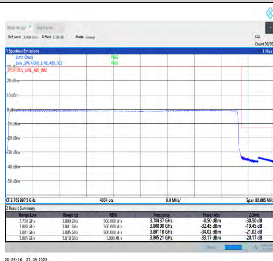
1-N78-3700-3800-PC2-30-70-H-6-CP-QPSK-Outer_Full-189@0-Ant7-1--PASS-see graph
