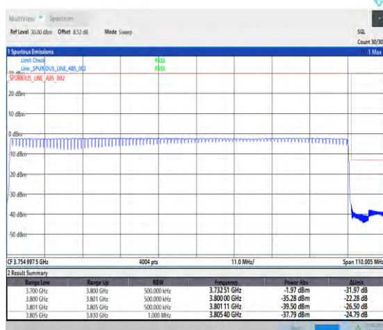
1-N78-3700-3800-PC2-30-100-H-6-CP-QPSK-Outer_Full-273@0-Ant7-1--PASS-see graph
