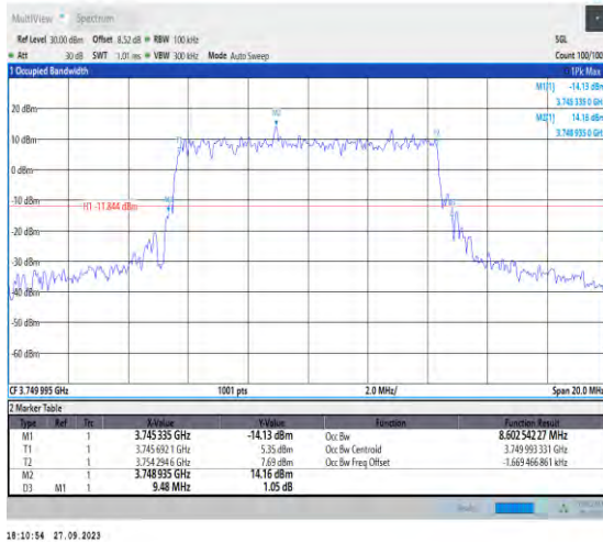
1-N78-3700-3800-PC2-30-10-M-3-DFT-16QAM-Oute r_Full-24@0-Ant7-8.603-9.480-≤10-PASS
