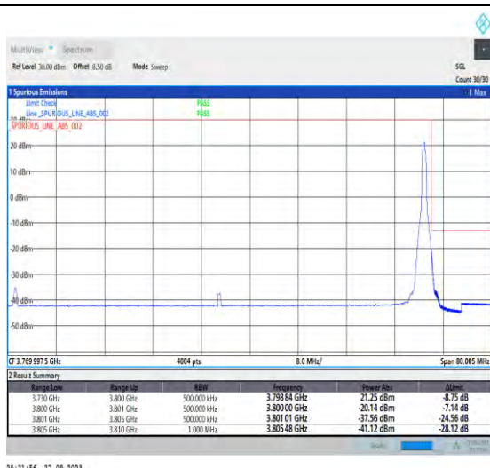
1-N78-3700-3800-PC2-30-70-H-2-DFT-PI2BPSK-Edge_1RB_Right-1@188-Ant7-1--PASS-see graph
