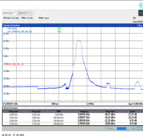
1-N78-3700-3800-PC2-30-10-L-4-CP-QPSK-Edge_1RB_Left-1@0-Ant7-1--PASS-see graph
