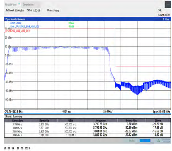
1-N78-3700-3800-PC2-30-20-H-3-DFT-PI2BPSK-Outer_Full-50@0-Ant7-1--PASS-see graph
