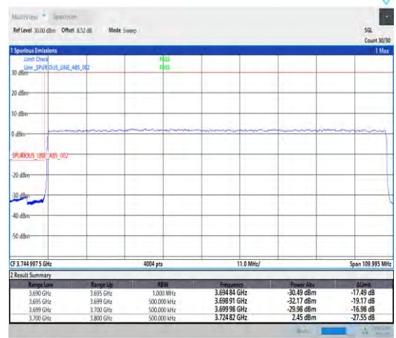
1-N78-3700-3800-PC2-30-100-L-3-DFT-PI2BPSK-Outer_Full-270@0-Ant7-1--PASS-see graph
