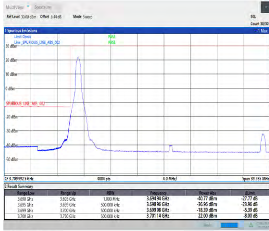
1-N78-3700-3800-PC2-30-30-L-1-DFT-PI2BPSK-Edge_1RB_Left-1@0-Ant7-1--PASS-see graph
