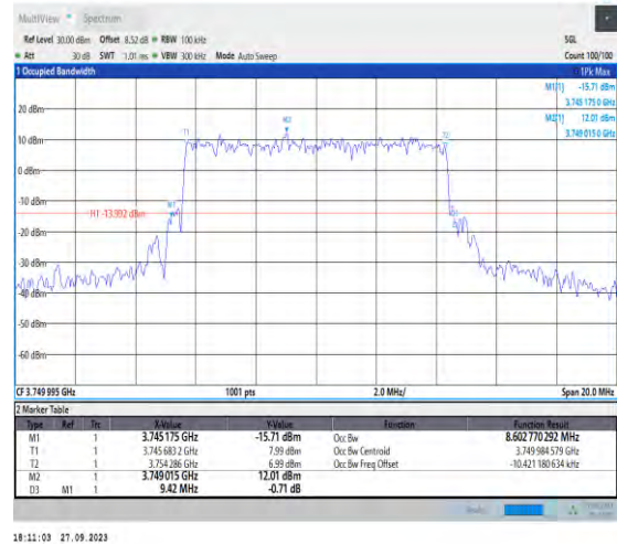
1-N78-3700-3800-PC2-30-10-M-4-DFT-64QAM-Oute r_Full-24@0-Ant7-8.603-9.420-≤10-PASS
