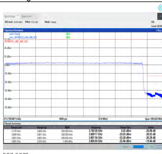
1-N78-3700-3800-PC2-30-90-H-3-DFT-PI2BPSK-Outer_Full-240@0-Ant7-1--PASS-see graph
