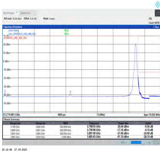
1-N78-3700-3800-PC2-30-60-H-5-CP-QPSK-Edge_1RB_Right-1@161-Ant7-1--PASS-see graph
