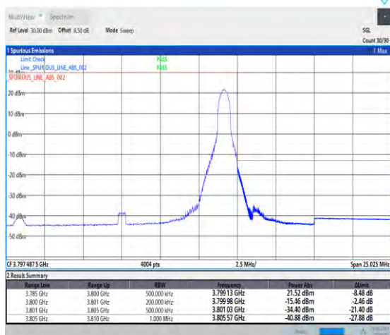
1-N78-3700-3800-PC2-30-15-H-2-DFT-PI2BPSK-Edge_1RB_Right-1@37-Ant7-1--PASS-see graph
