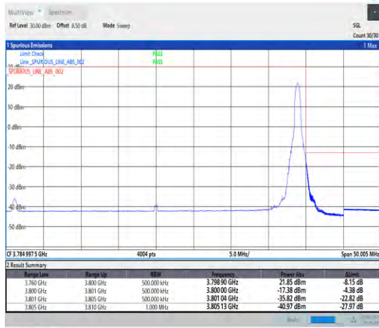
1-N78-3700-3800-PC2-30-40-H-2-DFT-PI2BPSK-Edge_1RB_Right-1@105-Ant7-1--PASS-see graph
