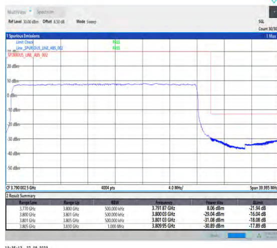
1-N78-3700-3800-PC2-30-30-H-3-DFT-PI2BPSK-Outer_Full-75@0-Ant7-1--PASS-see graph
