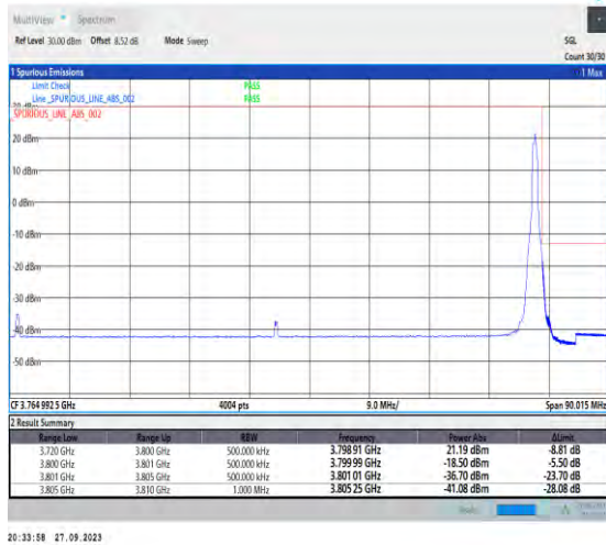
1-N78-3700-3800-PC2-30-80-H-2-DFT-PI2BPSK-Edge_1RB_Right-1@216-Ant7-1--PASS-see graph
