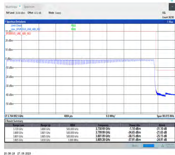
1-N78-3700-3800-PC2-30-80-H-6-CP-QPSK-Outer_Full-217@0-Ant7-1--PASS-see graph
