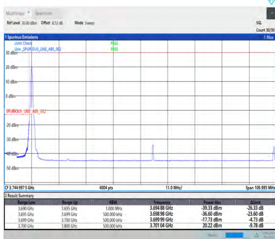
1-N78-3700-3800-PC2-30-100-L-4-CP-QPSK-Edge_1RB_Left-1@0-Ant7-1--PASS-see graph
