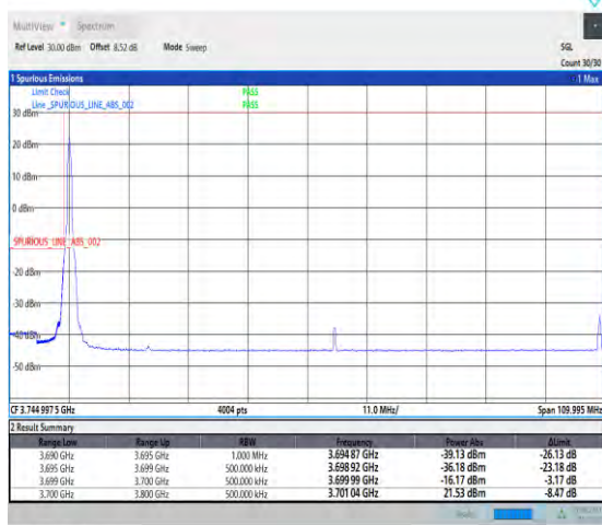
1-N78-3700-3800-PC2-30-100-L-1-DFT-PI2BPSK-Edge_1RB_Left-1@0-Ant7-1--PASS-see graph
