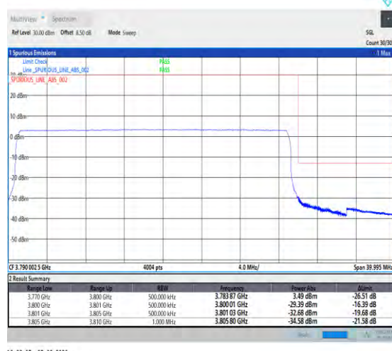
1-N78-3700-3800-PC2-30-30-H-6-CP-QPSK-Outer_Full-78@0-Ant7-1--PASS-see graph
