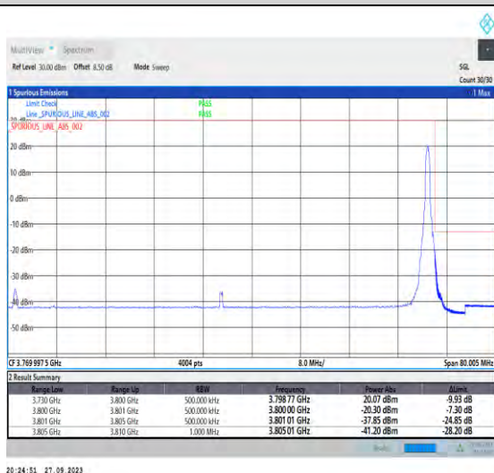
1-N78-3700-3800-PC2-30-70-H-5-CP-QPSK-Edge_1RB_Right-1@188-Ant7-1--PASS-see graph
