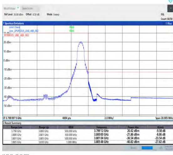
1-N78-3700-3800-PC2-30-10-H-5-CP-QPSK-Edge_1RB_Right-1@23-Ant7-1--PASS-see graph
