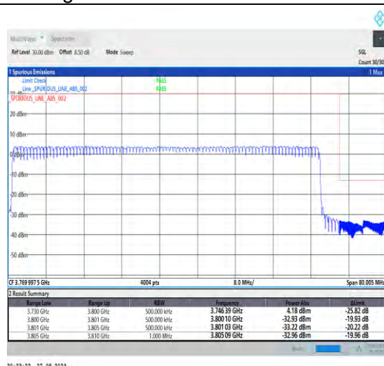
1-N78-3700-3800-PC2-30-70-H-3-DFT-PI2BPSK-Outer_Full-180@0-Ant7-1--PASS-see graph
