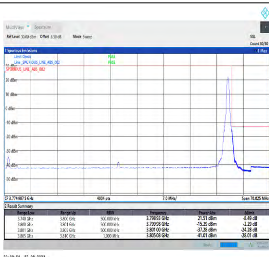
1-N78-3700-3800-PC2-30-60-H-2-DFT-PI2BPSK-Edge_1RB_Right-1@161-Ant7-1--PASS-see graph
