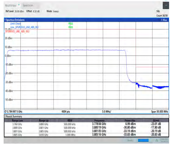
1-N78-3700-3800-PC2-30-40-H-3-DFT-PI2BPSK-Outer_Full-100@0-Ant7-1--PASS-see graph
