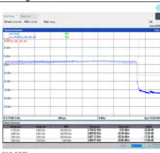
1-N78-3700-3800-PC2-30-60-H-3-DFT-PI2BPSK-Outer_Full-162@0-Ant7-1--PASS-see graph
