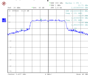
99 % Occupied Bandwidth
