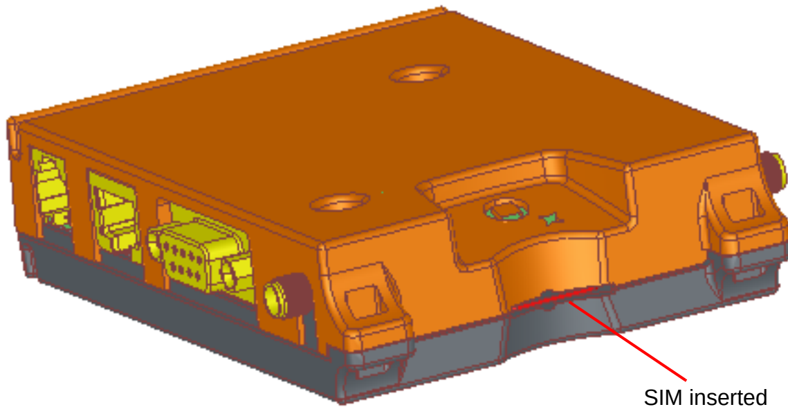
Figure 7: SIM interface
