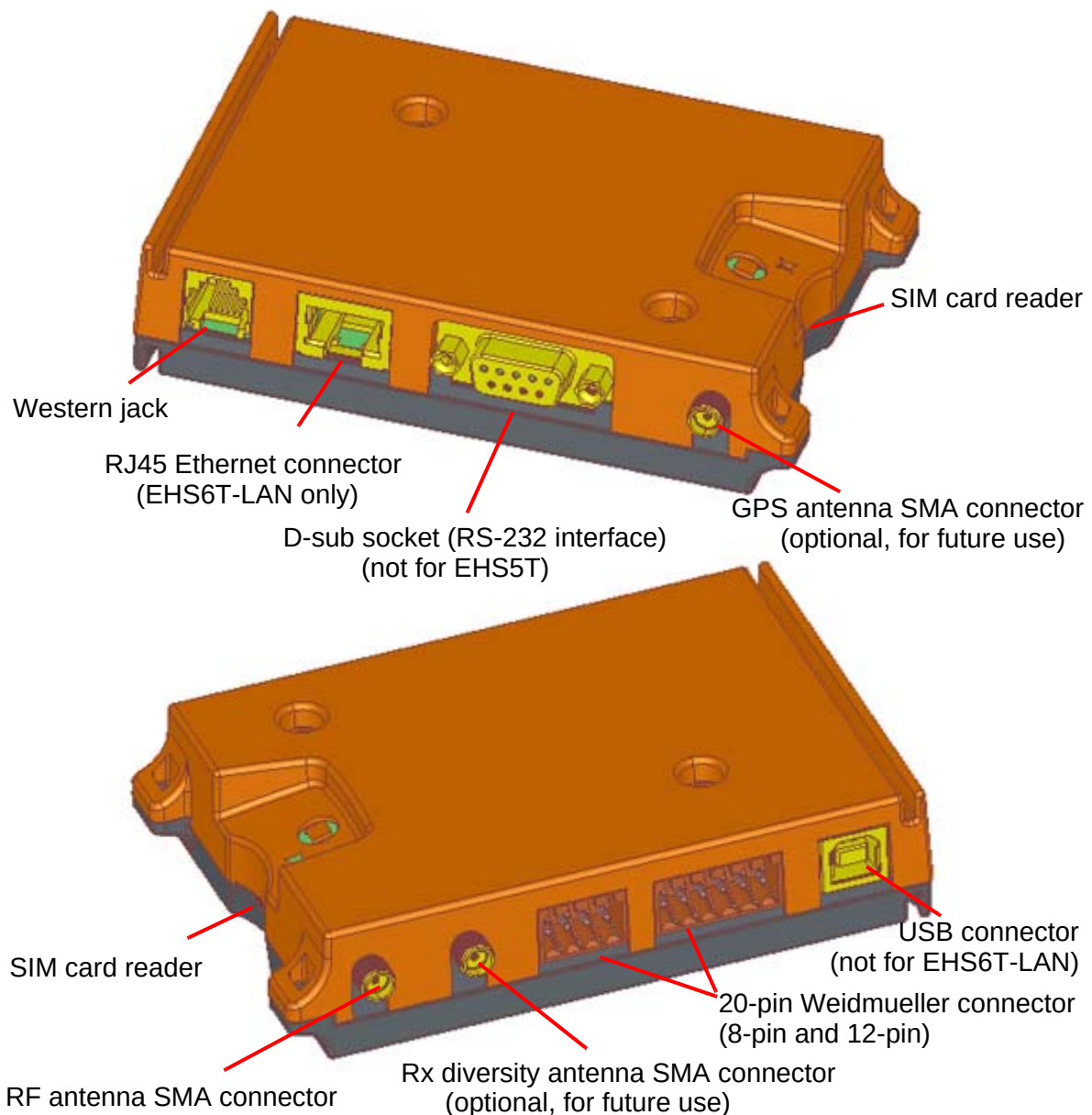
Figure 2: Java Terminals 3D view
