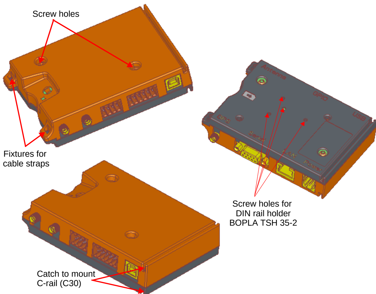
Figure 12: Mounting the Java Terminals
