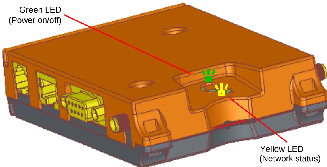
Figure 8: Status LED
