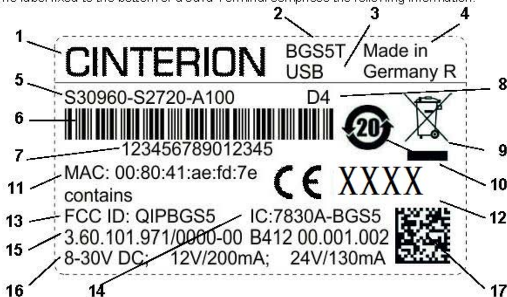
Figure 1: Sample Java Terminal label (BGS5T)
