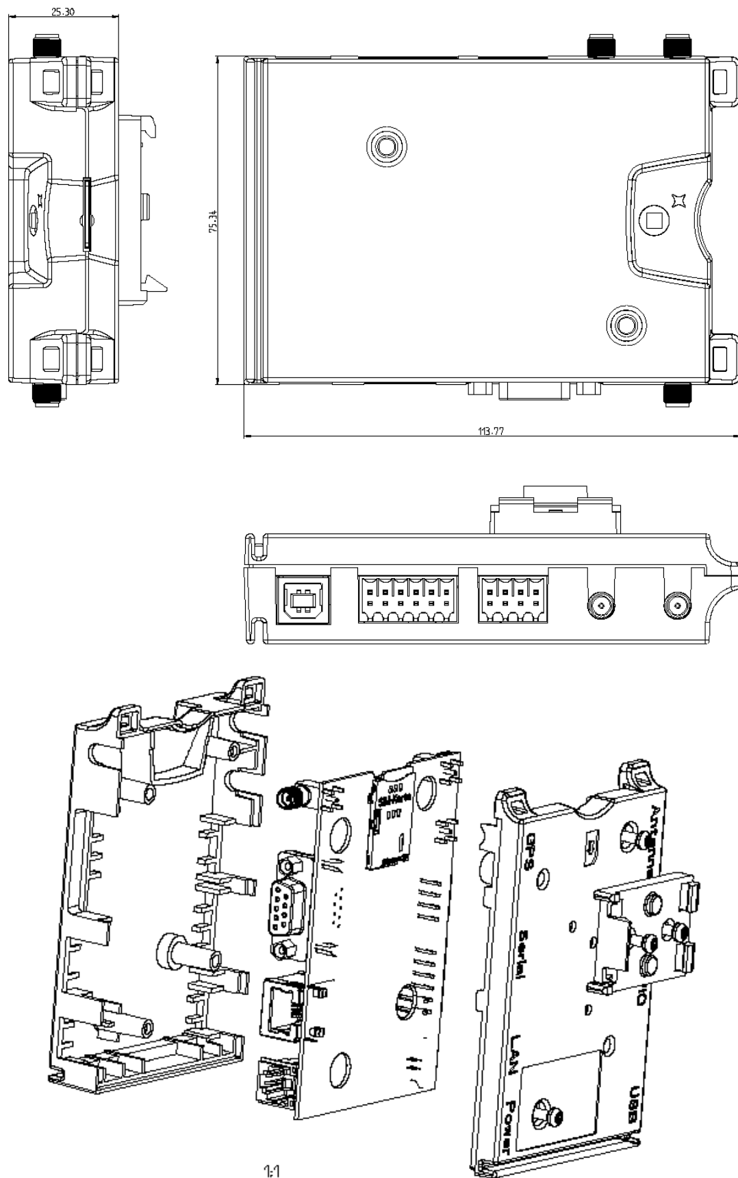
Figure 11: Java Terminals mechanical dimensions
