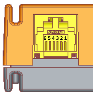
Figure 6: 6-pole Western jack for power supply, ignition, reset, typical connection
