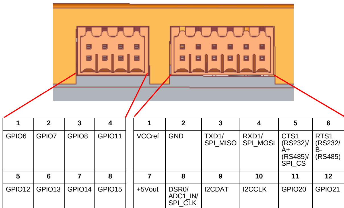
Figure 5: Weidmueller connectors (8-pin and 12-pin)
