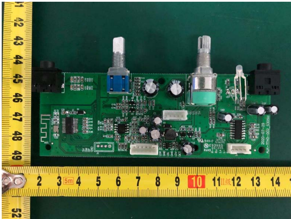
Internal photos M/N: VSC-550BT
