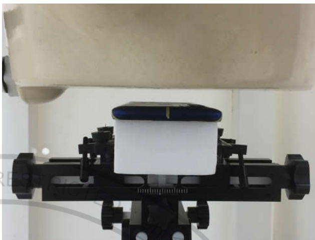
Back, Test Separation 14 mm(sensor on)
