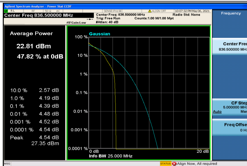
Band5-3MHz-QPSK-20525-1RB#0
