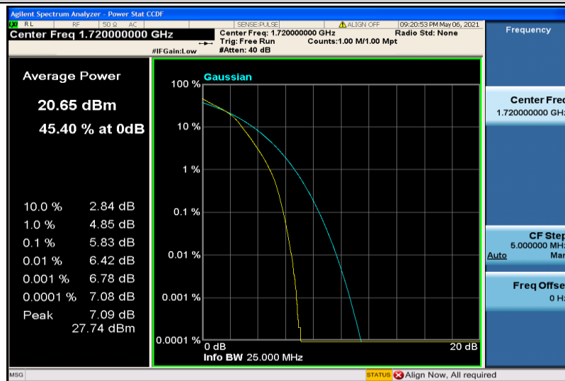
Band4-20MHz-16QAM-20050-100RB#0
