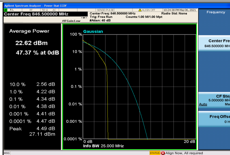
Band5-5MHz-QPSK-20625-1RB#0
