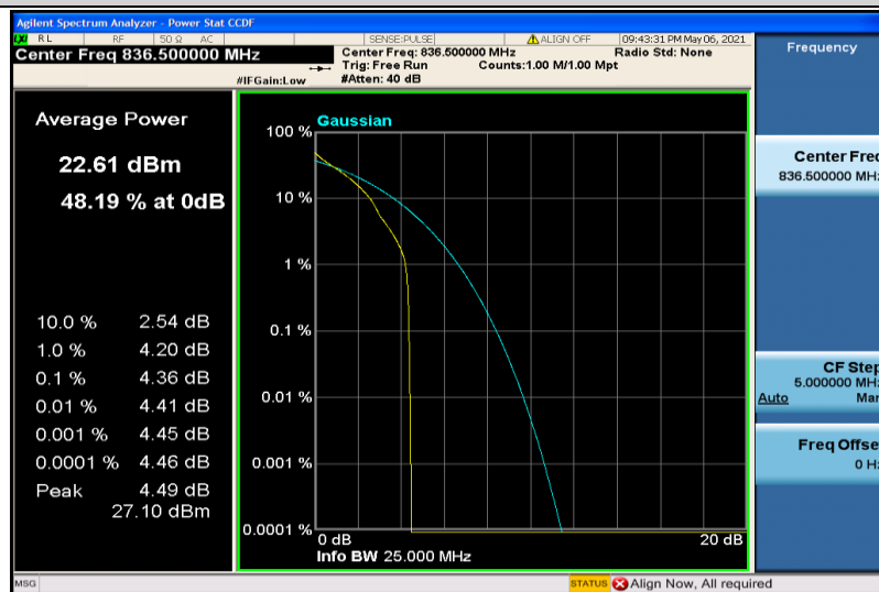
Band5-1.4MHz-QPSK-20525-1RB#0
