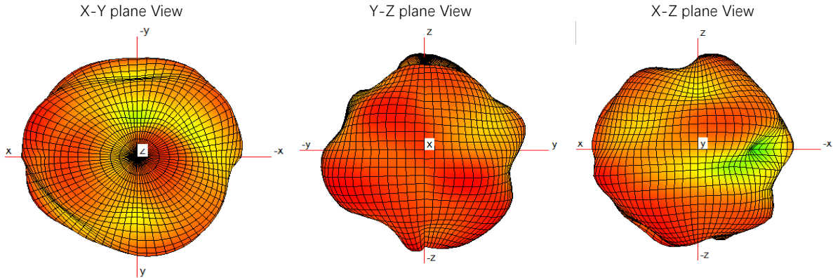
3D Radiation Pattern for 2440MHz
