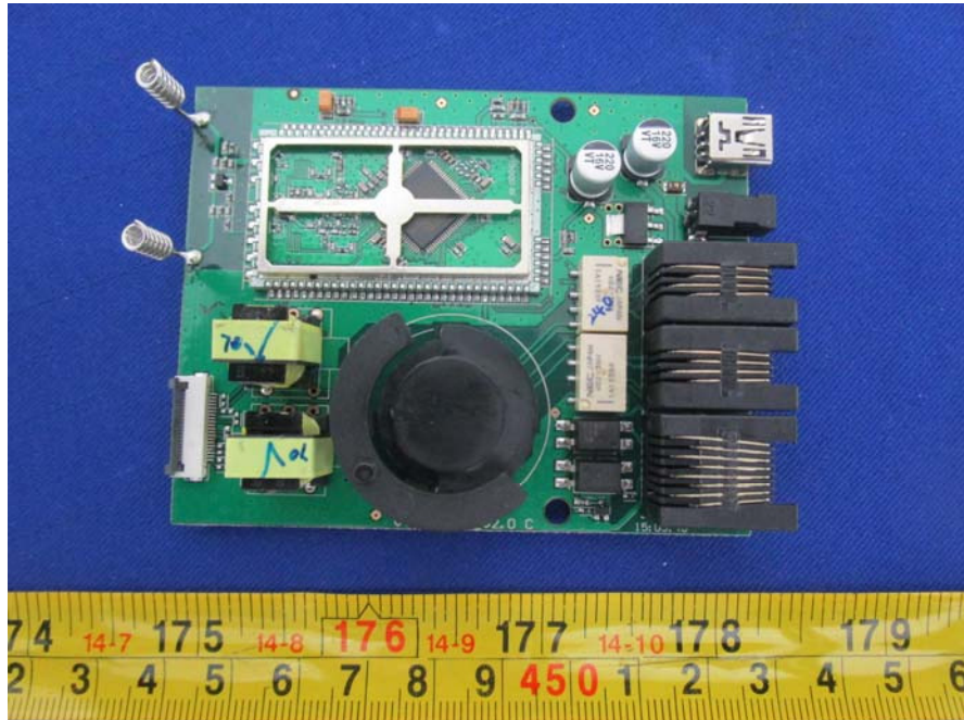
EUT – Main Board Unshielded View
