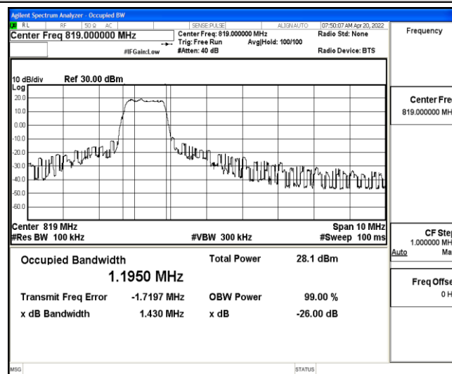
Band26-5MHz-QPSK-26740-6-0-Low-1.1950-1.430-PASS
