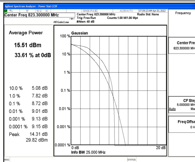
Band26-1.4MHz-QPSK-26783-6-0-Low-8.72-&lt;=13-PASS
