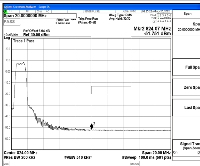
Band26-10MHz-16QAM-26740-6-0-Low--52.06,-51.75-PASS
