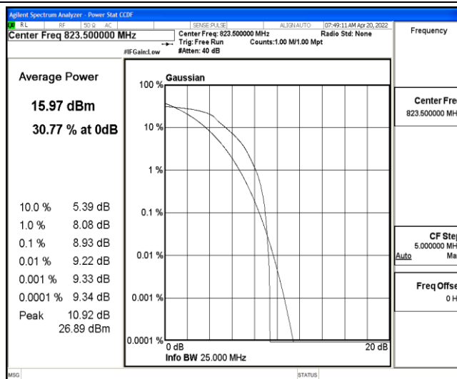
Band26-5MHz-16QAM-26785-6-0-Low-8.93-&lt;=13-PASS
