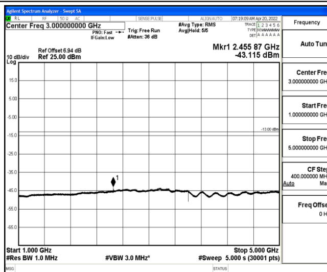
Band26-1.4MHz-16QAM-26740-1-0-Low-1000-5000--43.12-PASS
