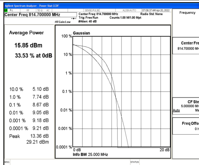
Band26-1.4MHz-QPSK-26697-6-0-Low-8.67-<=13-PASS
