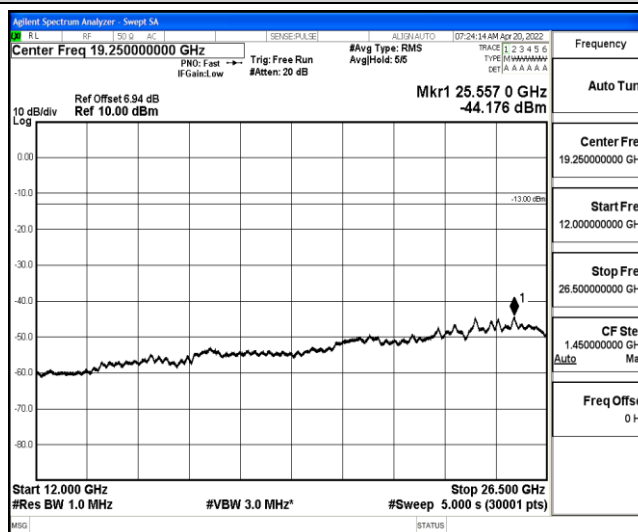
Band26-1.4MHz-16QAM-26783-1-0-High-12000-26500--44.18-PASS
