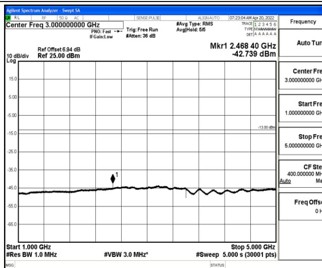
Band26-1.4MHz-16QAM-26783-1-0-High-1000-5000--42.74-PASS
