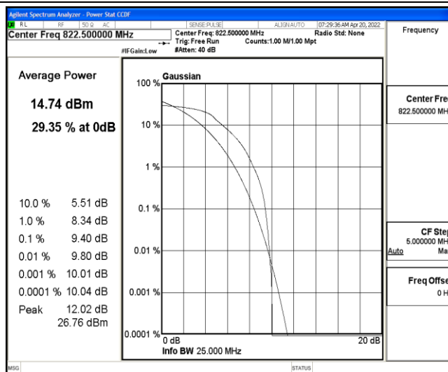
Band26-3MHz-16QAM-26775-6-0-Low-9.40-&lt;=13-PASS
