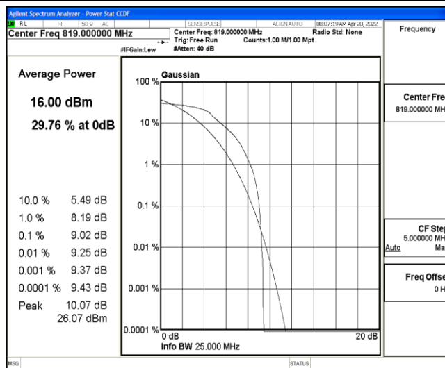
Band26-10MHz-QPSK-26740-6-0-Low-9.02-&lt;=13-PASS
