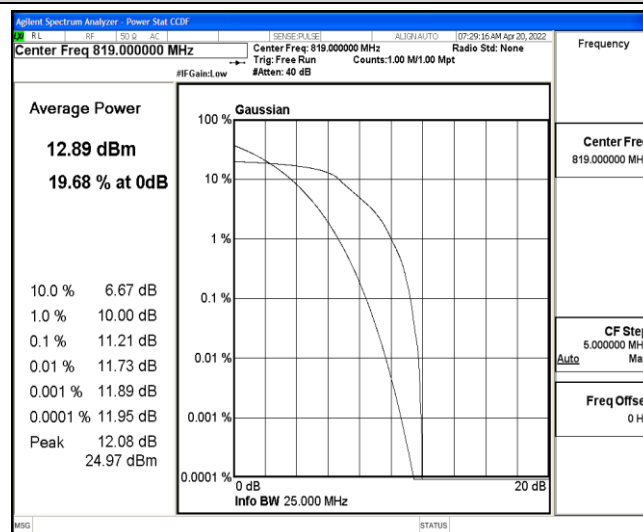
Band26-3MHz-16QAM-26740-6-0-Low-11.21-&lt;=13-PASS
