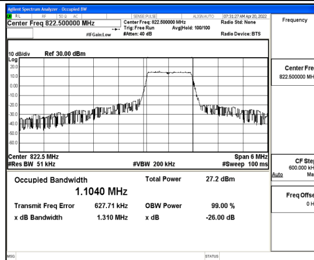
Band26-3MHz-16QAM-26775-6-0-High-1.1040-1.310-PASS
