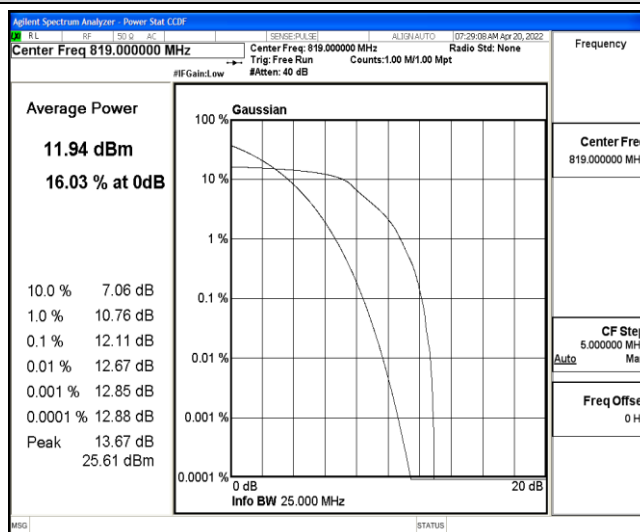
Band26-3MHz-QPSK-26740-6-0-Low-12.11-&lt;=13-PASS
