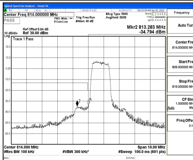
Band26-5MHz-QPSK-26715-6-0-Low--33.90,-34.79-PASS
