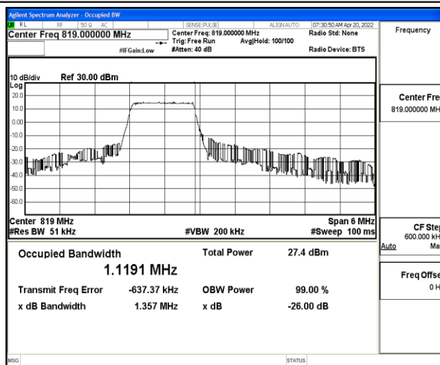
Band26-3MHz-16QAM-26740-6-0-Low-1.1191-1.357-PASS
