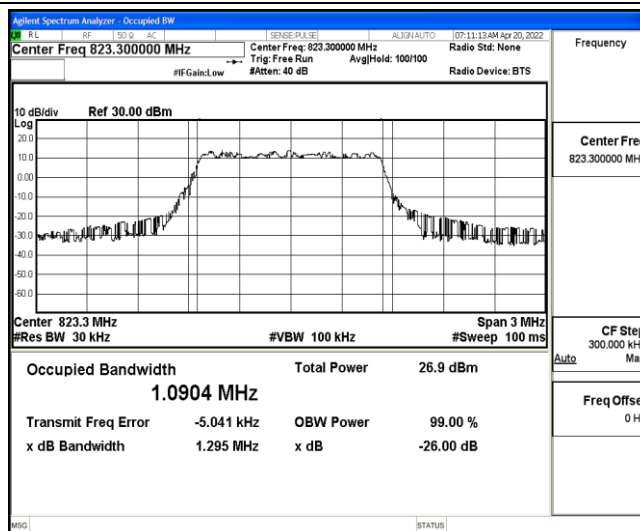
Band26-1.4MHz-QPSK-26783-6-0-High-1.0904-1.295-PASS
