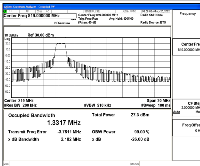
Band26-10MHz-16QAM-26740-6-0-Low-1.3317-2.182-PASS
