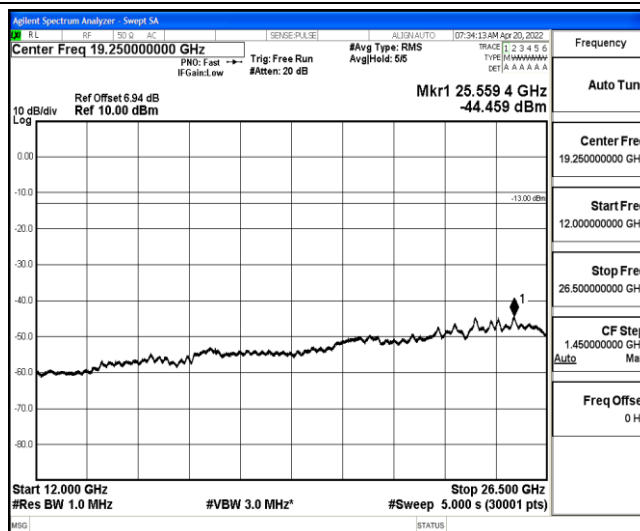
Band26-3MHz-QPSK-26705-1-0-Low-12000-26500--44.46-PASS
