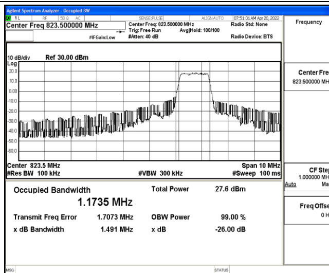
Band26-5MHz-16QAM-26785-6-0-High-1.1735-1.491-PASS
