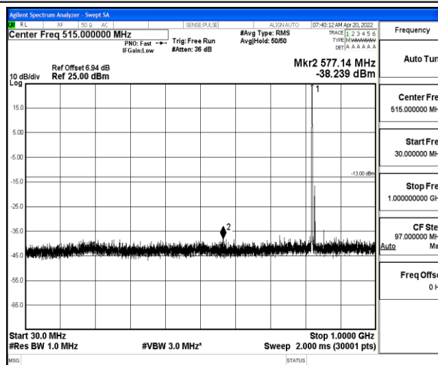
Band26-3MHz-QPSK-26775-1-0-High-30-1000--38.24-PASS
