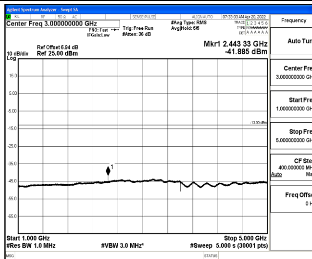
Band26-3MHz-QPSK-26705-1-0-Low-1000-5000--41.89-PASS
