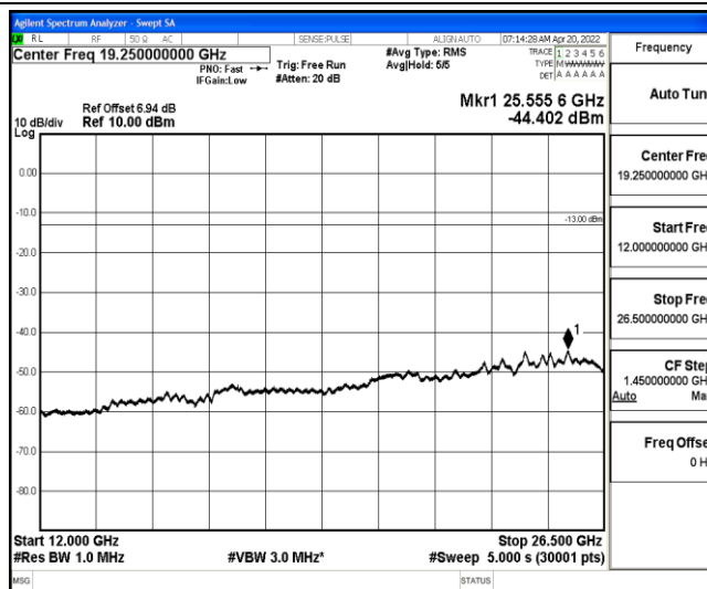
Band26-1.4MHz-QPSK-26697-1-0-Low-12000-26500--44.4-PASS
