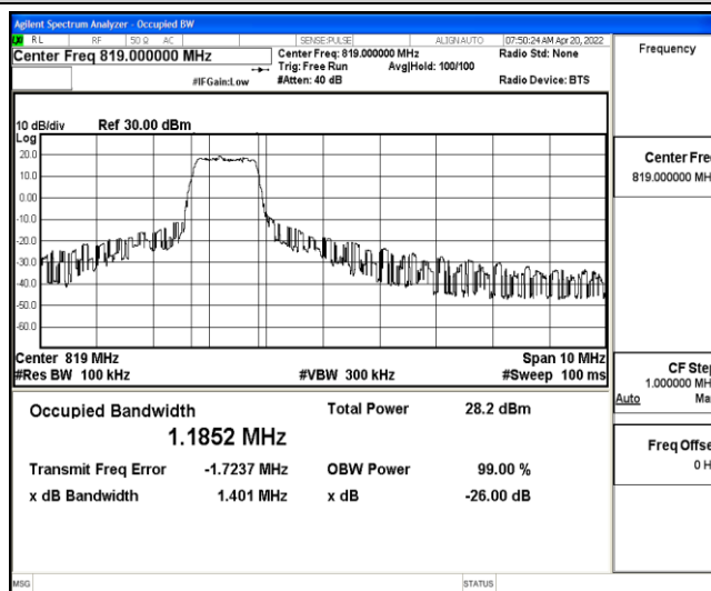
Band26-5MHz-16QAM-26740-6-0-Low-1.1852-1.401-PASS
