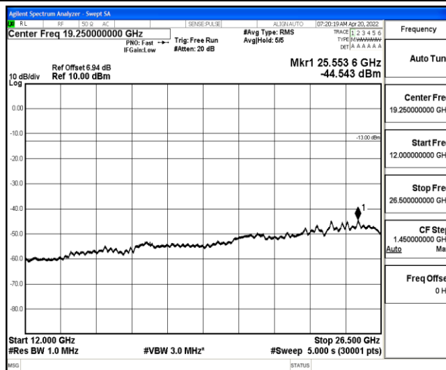
Band26-1.4MHz-16QAM-26740-1-0-Low-12000-26500--44.54-PASS
