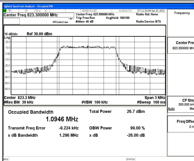
Band26-1.4MHz-16QAM-26783-6-0-High-1.0946-1.296-PASS
