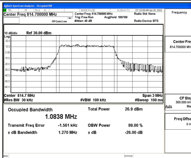
Band26-1.4MHz-16QAM-26697-6-0-Low-1.0838-1.270-PASS
