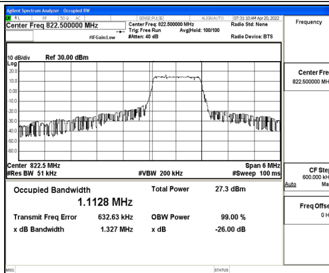
Band26-3MHz-QPSK-26775-6-0-High-1.1128-1.327-PASS
