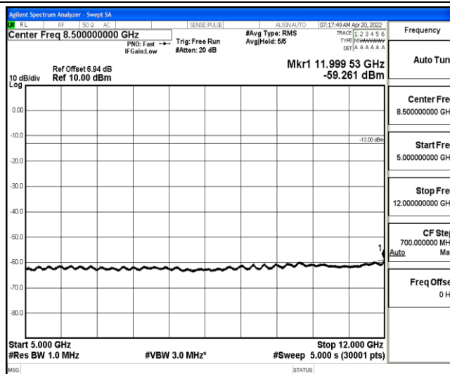
Band26-1.4MHz-QPSK-26740-1-0-Low-5000-12000--59.26-PASS
