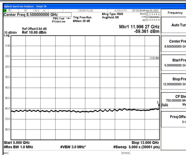
Band26-3MHz-QPSK-26705-1-0-Low-5000-12000--59.36-PASS
