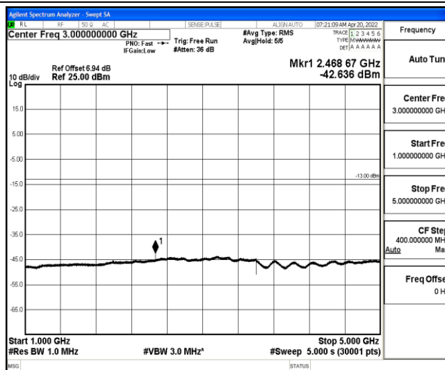
Band26-1.4MHz-QPSK-26783-1-0-High-1000-5000--42.64-PASS
