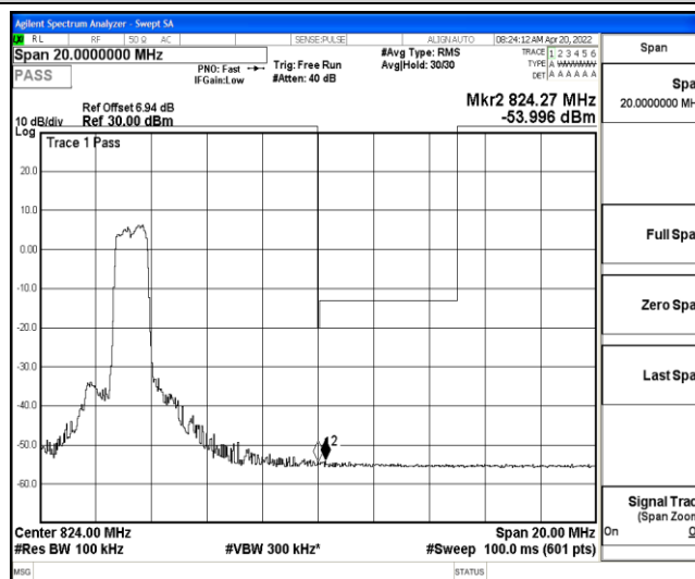
Band26-5MHz-16QAM-26740-6-0-Low--54.21,-53.88-PASS
