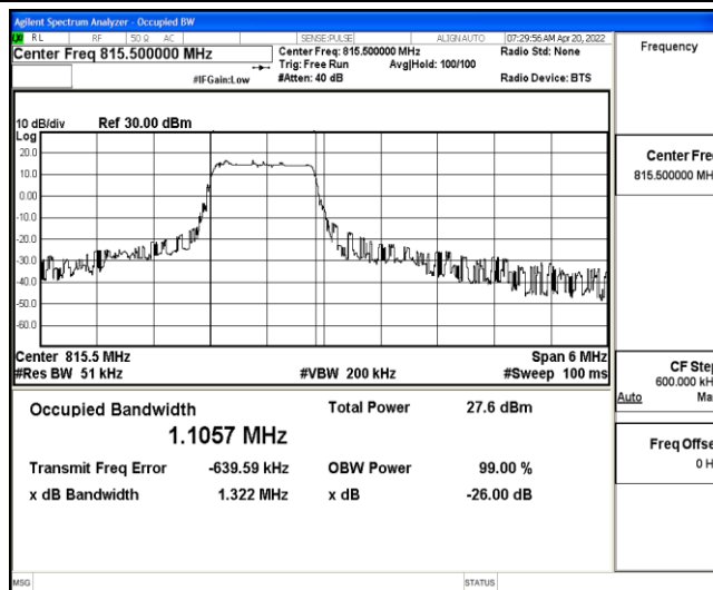
Band26-3MHz-QPSK-26705-6-0-Low-1.1057-1.322-PASS
