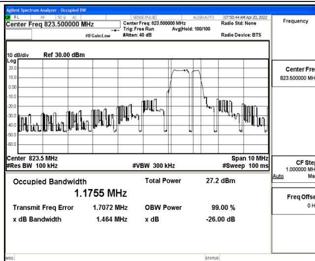
Band26-5MHz-QPSK-26785-6-0-High-1.1755-1.464-PASS
