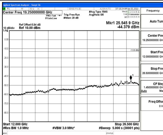
Band26-1.4MHz-QPSK-26740-1-0-Low-12000-26500--44.38-PASS
