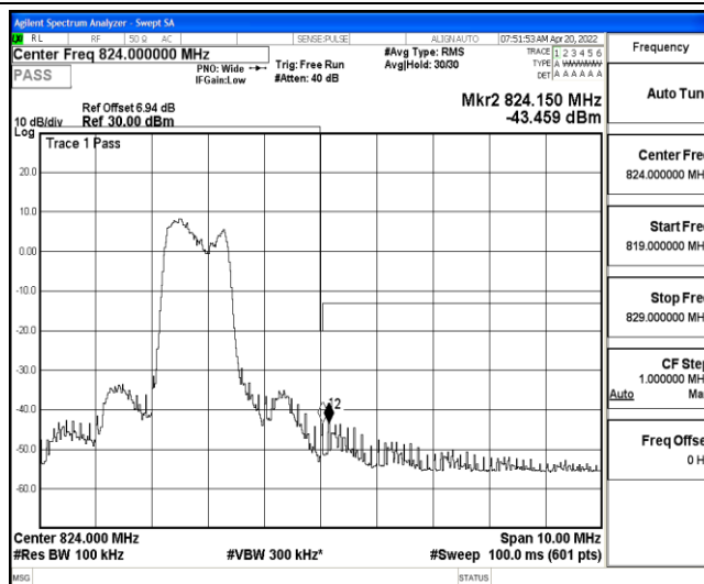
Band26-5MHz-16QAM-26785-6-0-Low--43.38,-43.46-PASS
