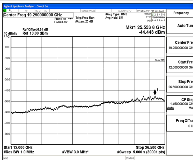
Band26-1.4MHz-16QAM-26697-1-0-Low-12000-26500--44.44-PASS
