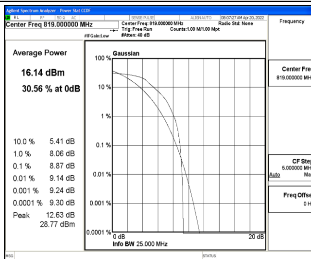
Band26-10MHz-16QAM-26740-6-0-Low-8.87-&lt;=13-PASS
