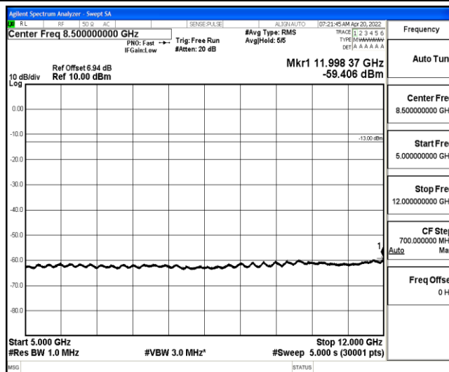
Band26-1.4MHz-QPSK-26783-1-0-High-5000-12000--59.41-PASS
