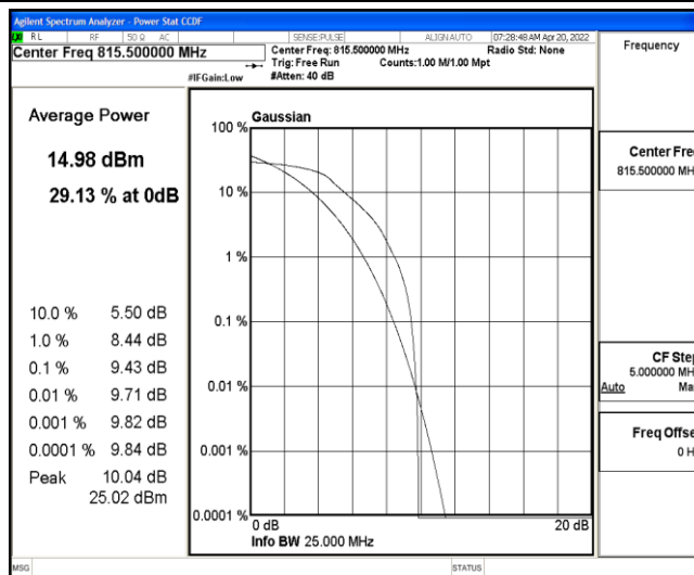
Band26-3MHz-QPSK-26705-6-0-Low-9.43-&lt;=13-PASS
