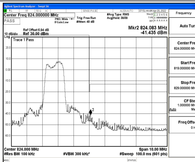
Band26-5MHz-QPSK-26785-6-0-Low--43.12,-41.44-PASS
