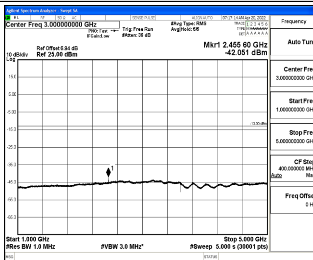
Band26-1.4MHz-QPSK-26740-1-0-Low-1000-5000--42.05-PASS
