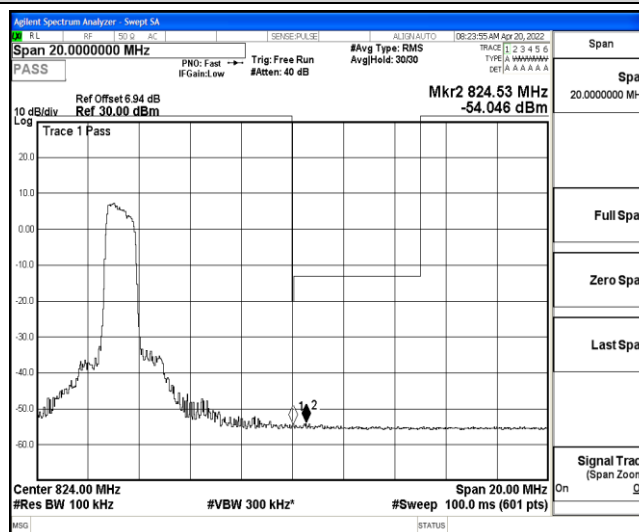
Band26-5MHz-QPSK-26740-6-0-Low--54.31,-54.05-PASS
