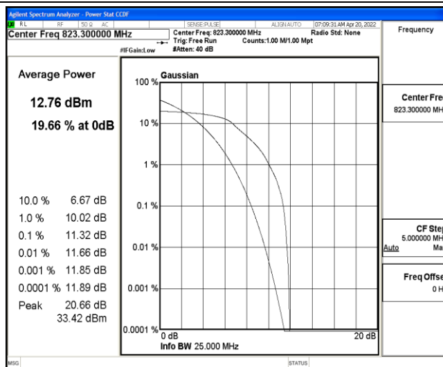
Band26-1.4MHz-16QAM-26783-6-0-Low-11.32-&lt;=13-PASS
