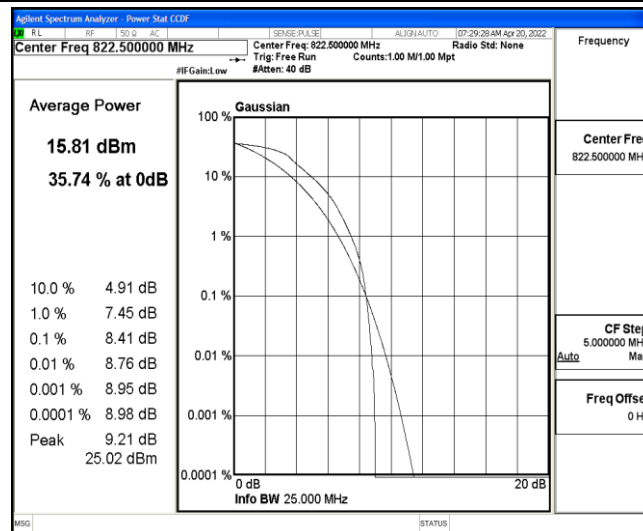
Band26-3MHz-QPSK-26775-6-0-Low-8.41-&lt;=13-PASS
