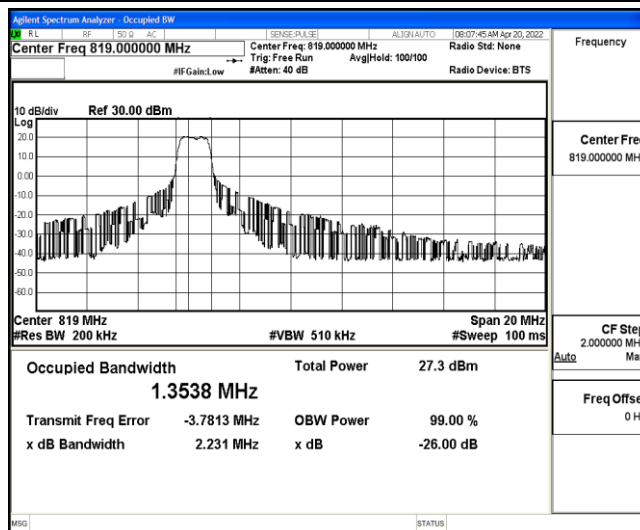
Band26-10MHz-QPSK-26740-6-0-Low-1.3538-2.231-PASS
