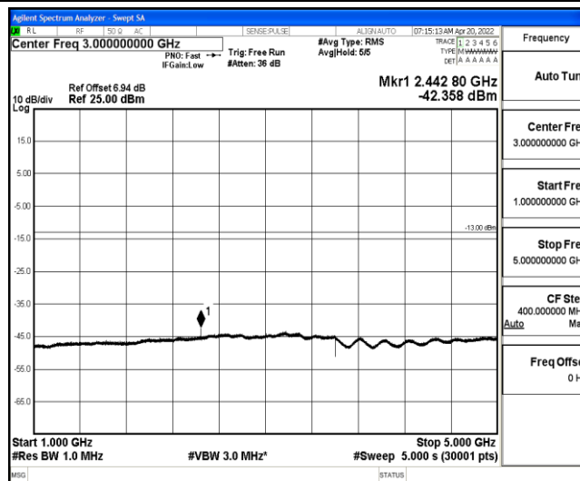
Band26-1.4MHz-16QAM-26697-1-0-Low-1000-5000--42.36-PASS
