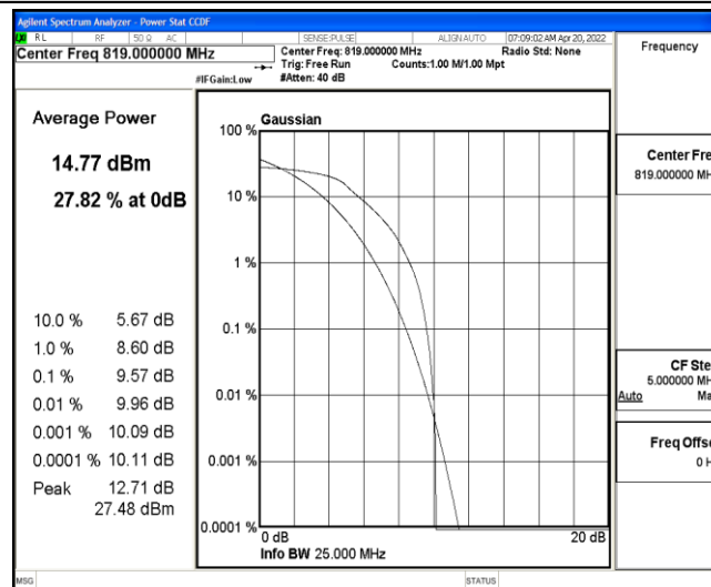
Band26-1.4MHz-QPSK-26740-6-0-Low-9.57-<=13-PASS
