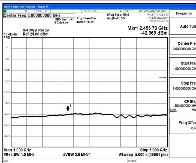
Band26-3MHz-QPSK-26740-1-0-Low-1000-5000--42.37-PASS
