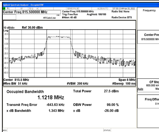
Band26-3MHz-16QAM-26705-6-0-Low-1.1218-1.343-PASS
