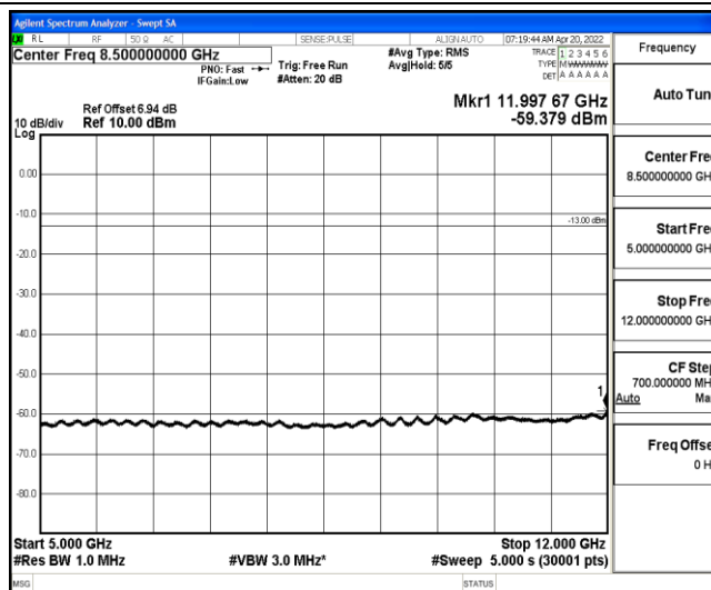
Band26-1.4MHz-16QAM-26740-1-0-Low-5000-12000--59.38-PASS
