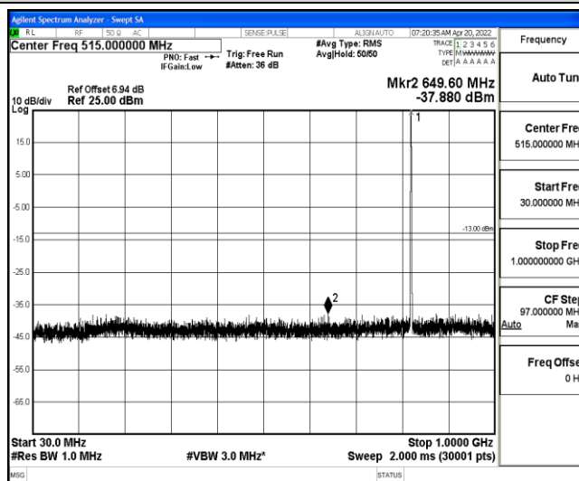
Band26-1.4MHz-QPSK-26783-1-0-High-30-1000--37.88-PASS
