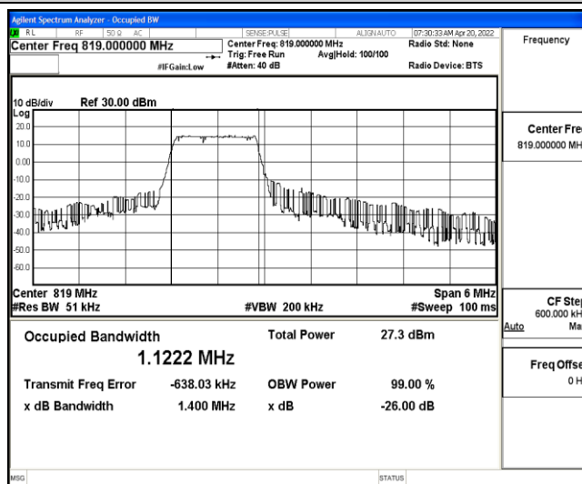
Band26-3MHz-QPSK-26740-6-0-Low-1.1222-1.400-PASS
