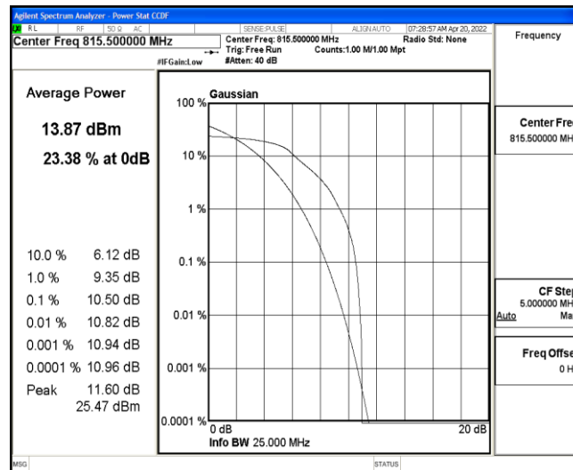
Band26-3MHz-16QAM-26705-6-0-Low-10.50-&lt;=13-PASS
