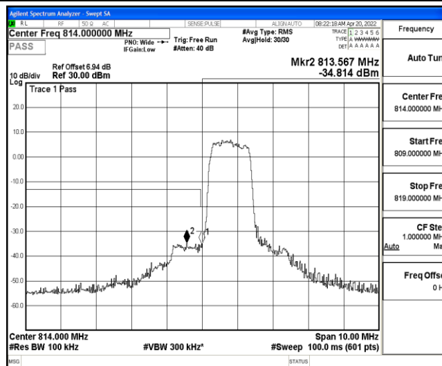
Band26-5MHz-16QAM-26715-6-0-Low--35.16,-34.81-PASS
