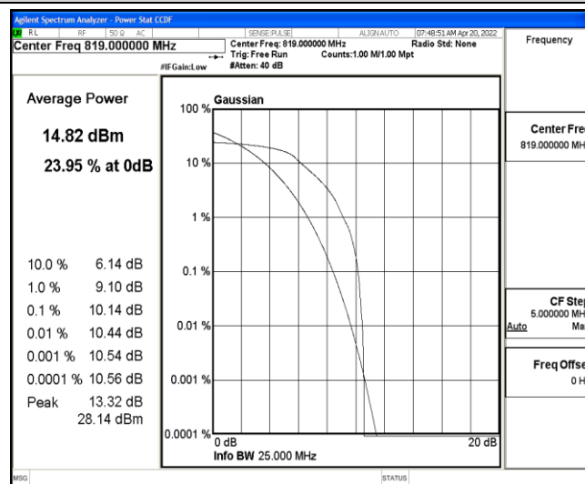
Band26-5MHz-16QAM-26740-6-0-Low-10.14-&lt;=13-PASS
