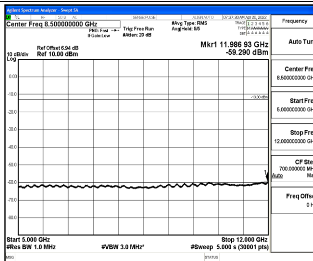
Band26-3MHz-QPSK-26740-1-0-Low-5000-12000--59.29-PASS
