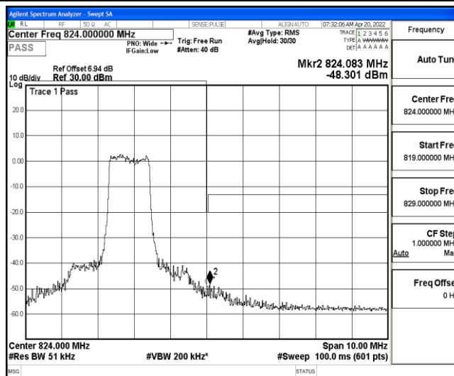
Band26-3MHz-QPSK-26775-6-0-Low--49.81,-48.30-PASS
