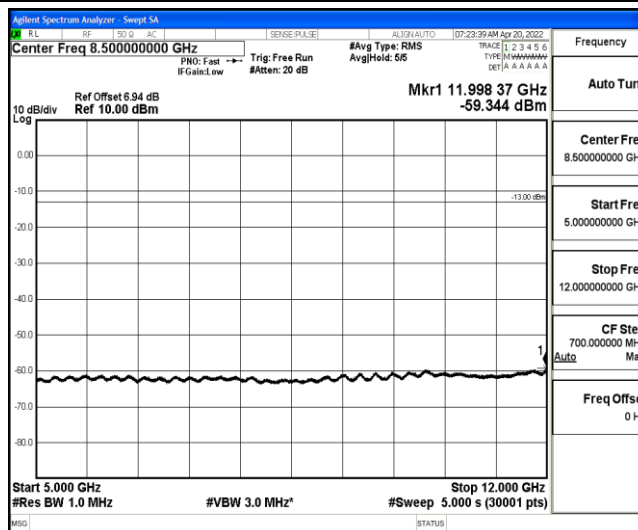
Band26-1.4MHz-16QAM-26783-1-0-High-5000-12000--59.34-PASS
