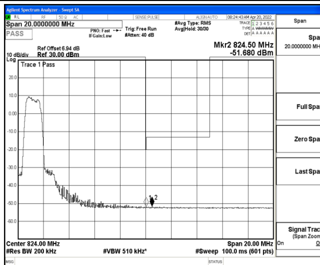
Band26-10MHz-QPSK-26740-6-0-Low--51.93,-51.68-PASS
