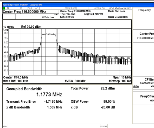
Band26-5MHz-16QAM-26715-6-0-Low-1.1773-1.565-PASS
