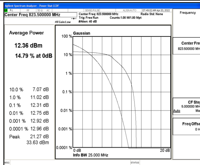
Band26-5MHz-QPSK-26785-6-0-Low-12.31-&lt;=13-PASS
