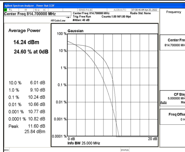
Band26-1.4MHz-16QAM-26697-6-0-Low-10.24-&lt;=13-PASS
