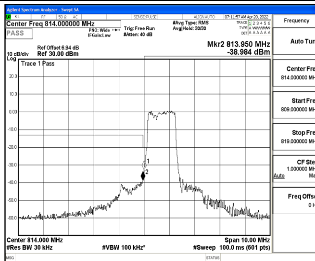
Band26-1.4MHz-16QAM-26697-6-0-Low--32.84,-38.98-PASS
