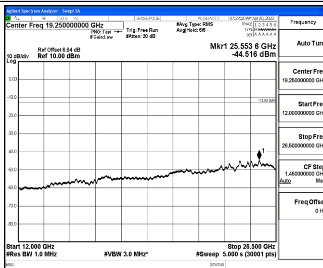
Band26-1.4MHz-QPSK-26783-1-0-High-12000-26500--44.52-PASS
