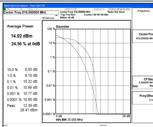
Band26-1.4MHz-16QAM-26740-6-0-Low-10.22-&lt;=13-PASS
