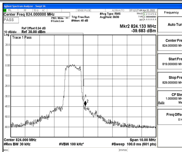
Band26-1.4MHz-16QAM-26783-6-0-Low--34.85,-39.68-PASS
