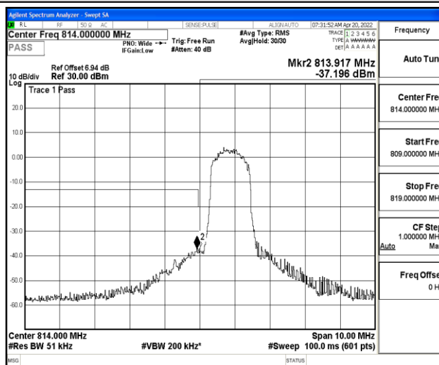
Band26-3MHz-16QAM-26705-6-0-Low--37.82,-37.20-PASS
