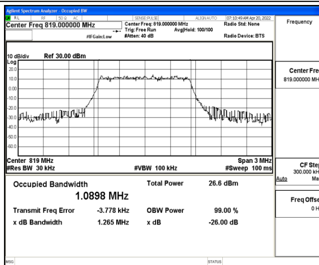
Band26-1.4MHz-16QAM-26740-6-0-Low-1.0898-1.265-PASS
