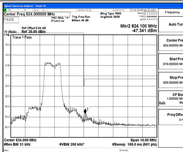
Band26-3MHz-16QAM-26775-6-0-Low--53.43,-47.34-PASS
