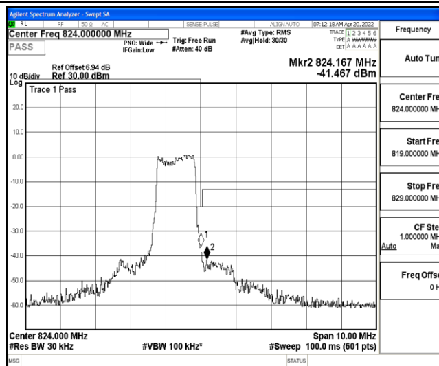
Band26-1.4MHz-QPSK-26783-6-0-Low--36.28,-41.47-PASS
