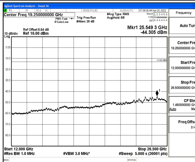
Band26-3MHz-QPSK-26740-1-0-Low-12000-26500--44.31-PASS
