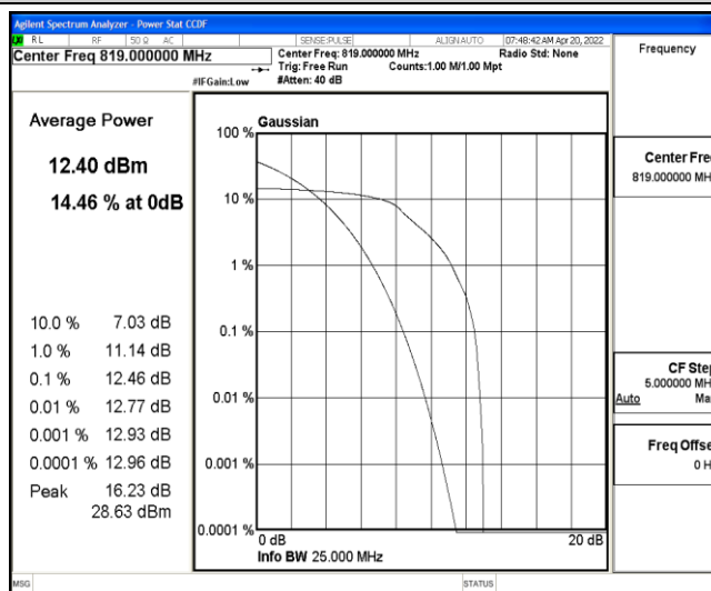
Band26-5MHz-QPSK-26740-6-0-Low-12.46-&lt;=13-PASS
