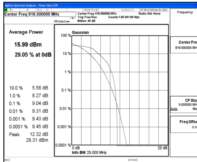
Band26-5MHz-16QAM-26715-6-0-Low-9.04-&lt;=13-PASS
