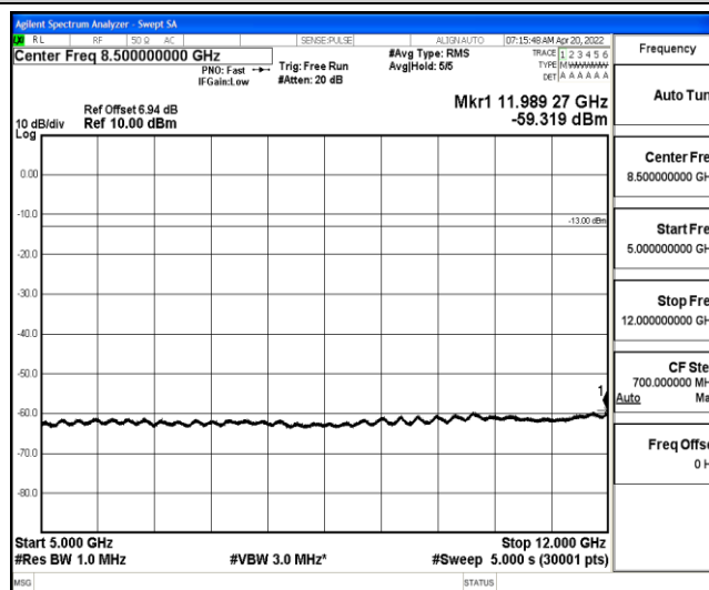
Band26-1.4MHz-16QAM-26697-1-0-Low-5000-12000--59.32-PASS
