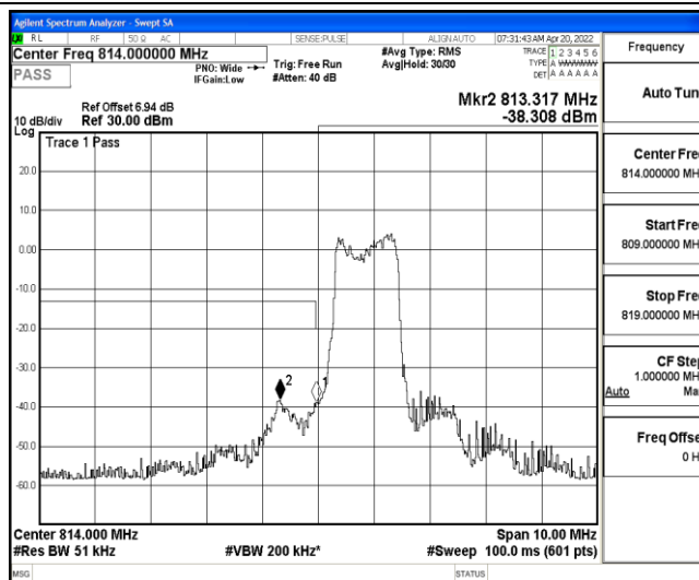
Band26-3MHz-QPSK-26705-6-0-Low--38.83,-38.31-PASS
