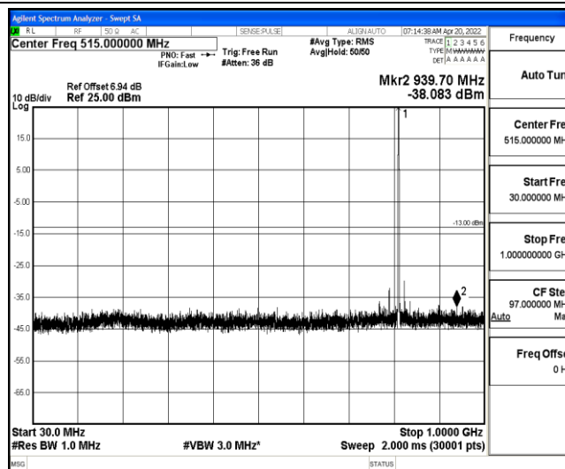
Band26-1.4MHz-16QAM-26697-1-0-Low-30-1000--38.08-PASS
