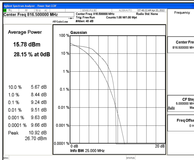
Band26-5MHz-QPSK-26715-6-0-Low-9.24-&lt;=13-PASS
