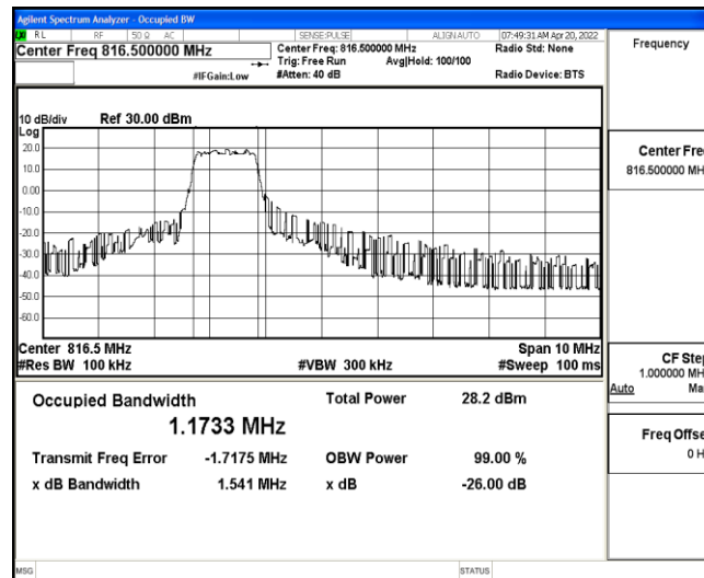
Band26-5MHz-QPSK-26715-6-0-Low-1.1733-1.541-PASS
