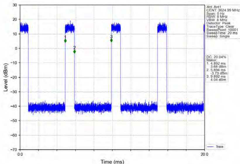
n78d_30kHz_MIMO_NTNV_100MHz_CP-OFDM 64 QAM_3624.99MHz_Inner_Full
