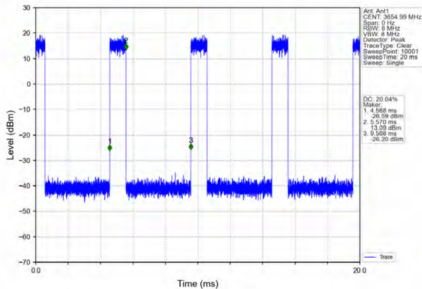
n78d_30kHz_MIMO_NTNV_90MHz_CP-OFDM_16_QAM_3654.99MHz_Inner_Full
