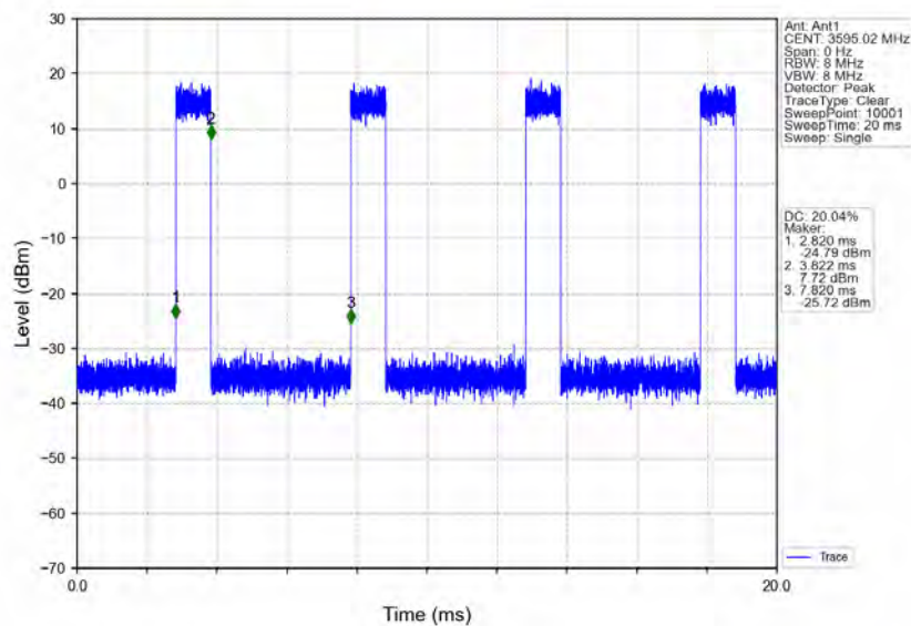
n78d_30kHz_MIMO_NTNV_90MHz_CP-OFDM 64 QAM_3595.02MHz_Inner_Full
