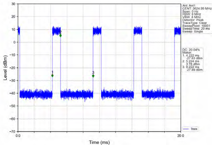
n78d_30kHz_MIMO_NTNV_90MHz_CP-OFDM_256_QAM_3624.99MHz_Inner_Full
