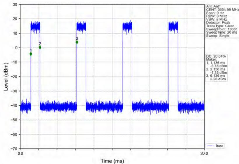
n78d_30kHz_MIMO_NTNV_90MHz_CP-OFDM 64 QAM_3654.99MHz_Inner_Full
