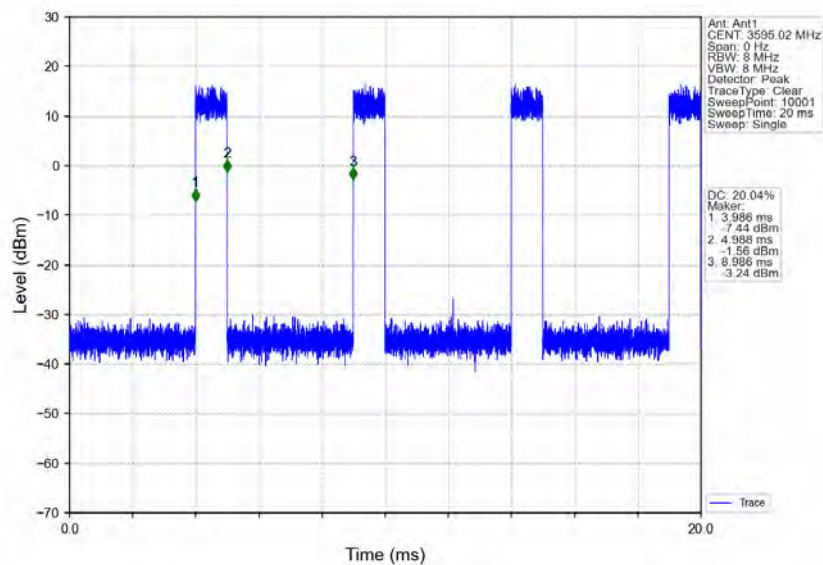
n78d_30kHz_MIMO_NTNV_90MHz_CP-OFDM_16_QAM_3595.02MHz_Inner_Full
