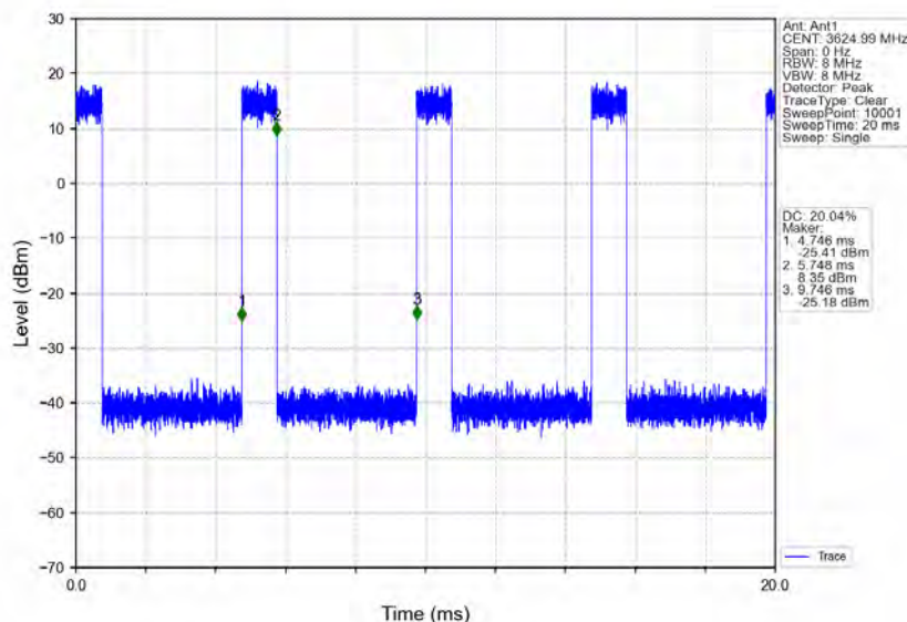
n78d_30kHz_MIMO_NTNV_90MHz_CP-OFDM 64 QAM_3624.99MHz_Inner_Full
