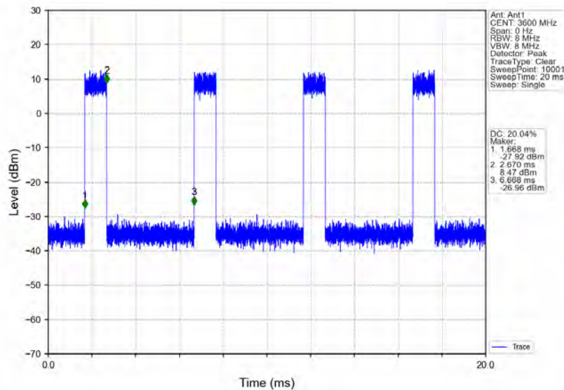
n78d_30kHz_MIMO_NTNV_100MHz_CP-OFDM_256_QAM_3600MHz_Inner_Full
