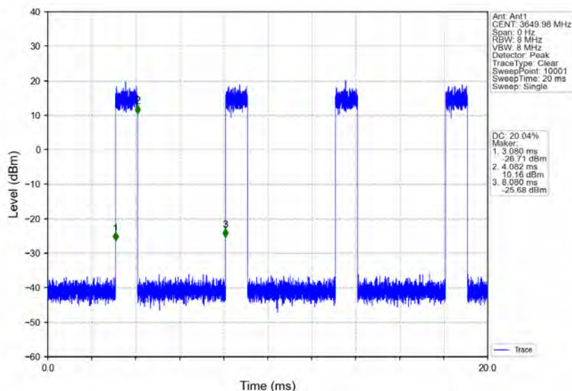
n78d_30kHz_MIMO_NTNV_100MHz_CP-OFDM_QPSK_3649.98MHz_Inner_Full
