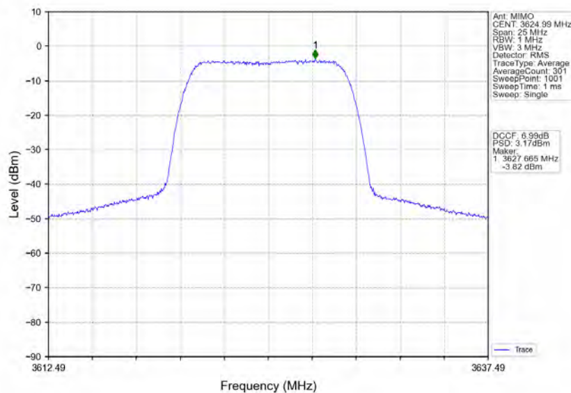
n78d_30kHz_MIMO_NTNV_10MHz_CP-OFDM 64 QAM_3624.99MHz_Inner_Full
