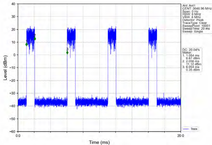
n78d_30kHz_MIMO_NTNV_100MHz_CP-OFDM_256_QAM_3600MHz_Edge_1RB_Right
