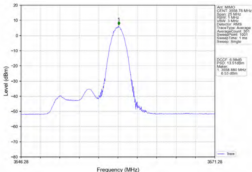
n78d_30kHz_MIMO_NTNV_10MHz_CP-OFDM_256_QAM_3555MHz_Inner_1RB_Right
