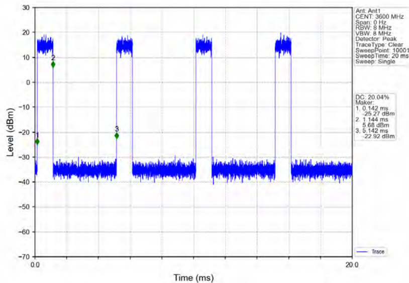
n78d_30kHz_MIMO_NTNV_100MHz_CP-OFDM_16_QAM_3600MHz_Inner_Full
