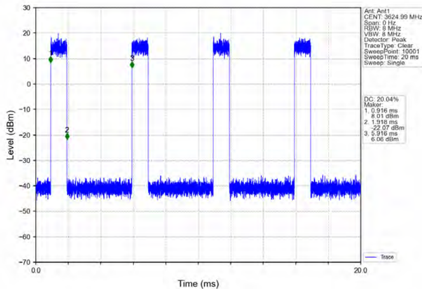
n78d_30kHz_MIMO_NTNV_100MHz_CP-OFDM_QPSK_3624.99MHz_Inner_Full
