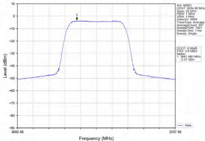
n78d_30kHz_MIMO_NTNV_10MHz_CP-OFDM_16_QAM_3694.98MHz_Inner_Full
