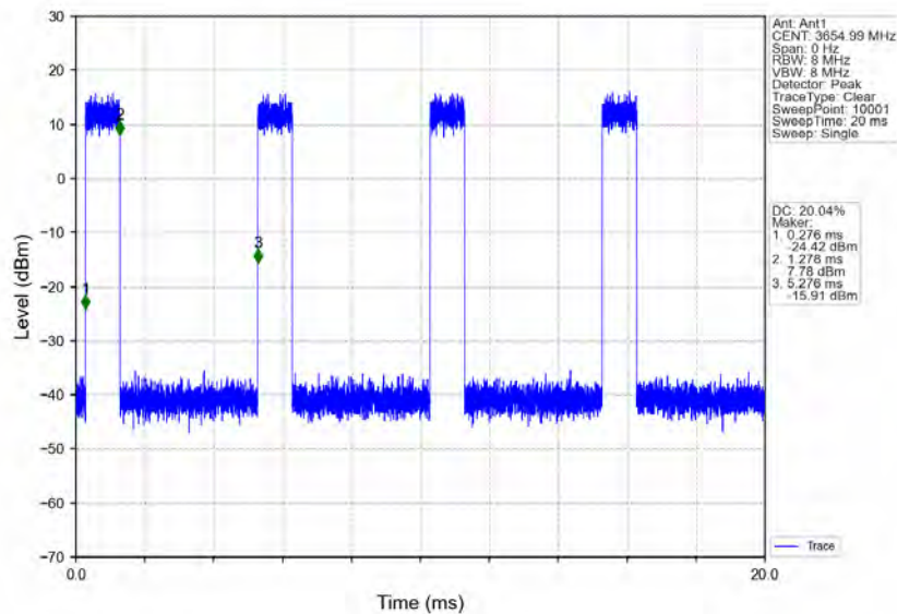
n78d_30kHz_MIMO_NTNV_90MHz_CP-OFDM_256_QAM_3654.99MHz_Inner_Full
