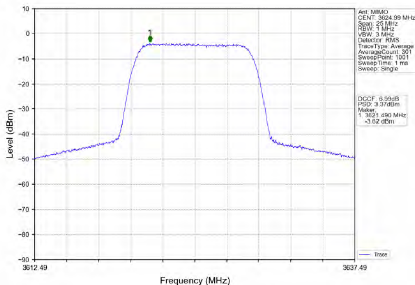
n78d_30kHz_MIMO_NTNV_10MHz_CP-OFDM_16_QAM_3624.99MHz_Inner_Full
