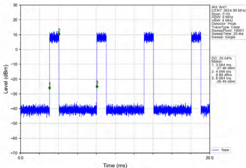
n78d_30kHz_MIMO_NTNV_100MHz_CP-OFDM_256_QAM_3624.99MHz_Inner_Full
