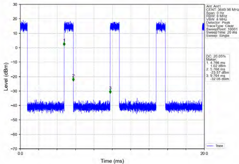
n78d_30kHz_MIMO_NTNV_100MHz_CP-OFDM_16_QAM_3649.98MHz_Inner_Full
