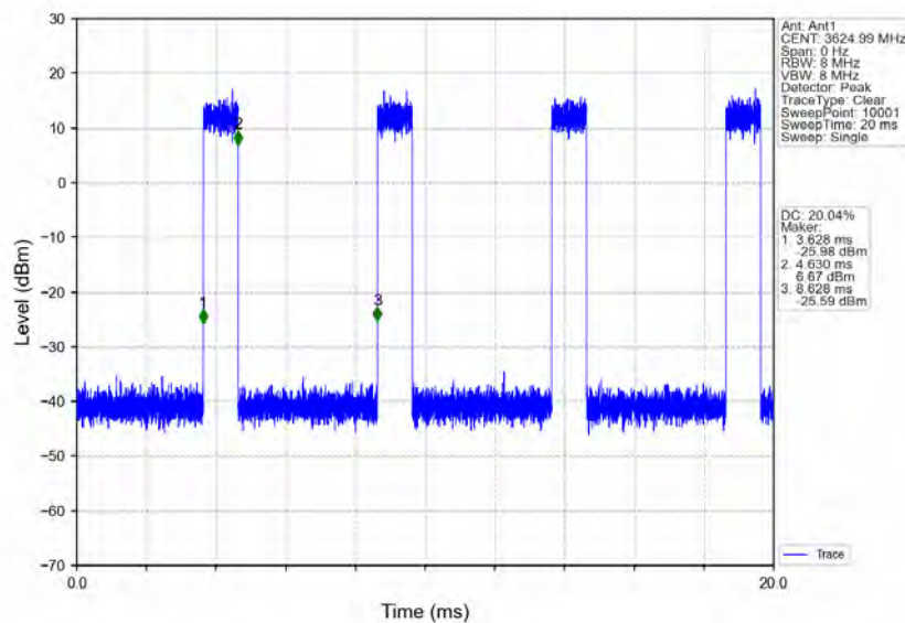
n78d_30kHz_MIMO_NTNV_90MHz_CP-OFDM_QPSK_3624.99MHz_Inner_Full
