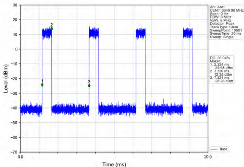
n78d_30kHz_MIMO_NTNV_100MHz_CP-OFDM 64 QAM_3649.98MHz_Inner_Full
