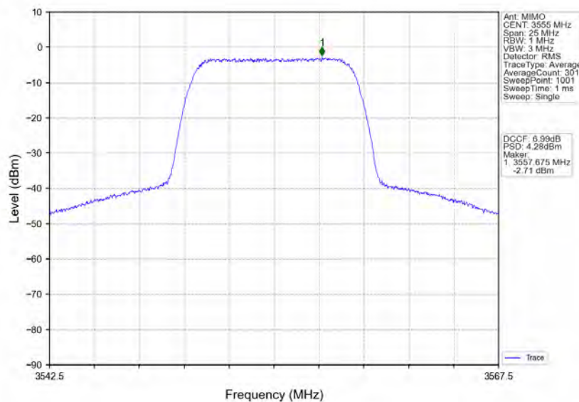
n78d_30kHz_MIMO_NTNV_10MHz_CP-OFDM_QPSK_3555MHz_Inner_Full
