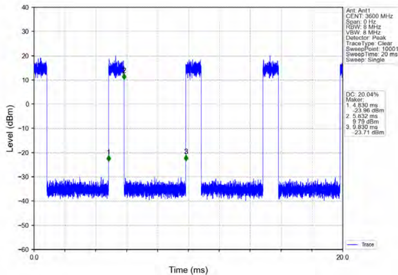
n78d_30kHz_MIMO_NTNV_100MHz_CP-OFDM_QPSK_3600MHz_Inner_Full
