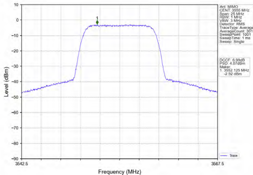
n78d_30kHz_MIMO_NTNV_10MHz_CP-OFDM_64_QAM_3555MHz_Inner_Full
