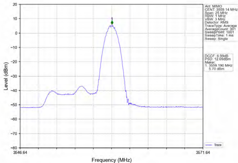
n78d_30kHz_MIMO_NTNV_10MHz_CP-OFDM 64 QAM_3555MHz_Edge_1RB_Right
