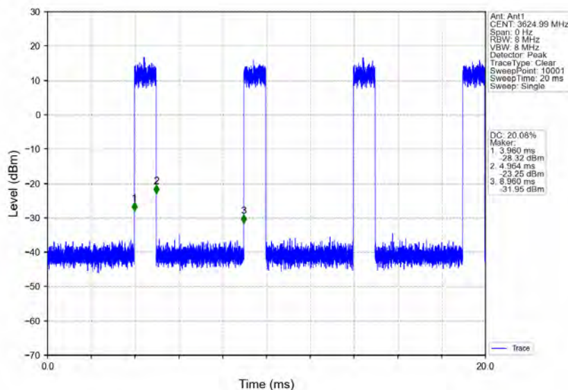
n78d_30kHz_MIMO_NTNV_100MHz_CP-OFDM_16_QAM_3624.99MHz_Inner_Full
