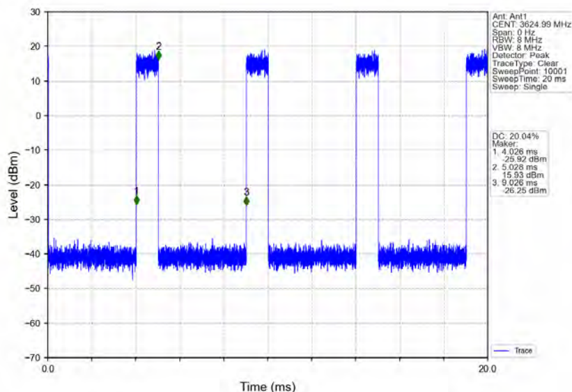
n78d_30kHz_MIMO_NTNV_90MHz_CP-OFDM_16_QAM_3624.99MHz_Inner_Full
