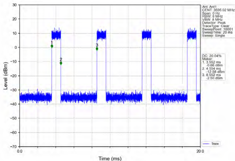
n78d_30kHz_MIMO_NTNV_90MHz_CP-OFDM_256_QAM_3595.02MHz_Inner_Full
