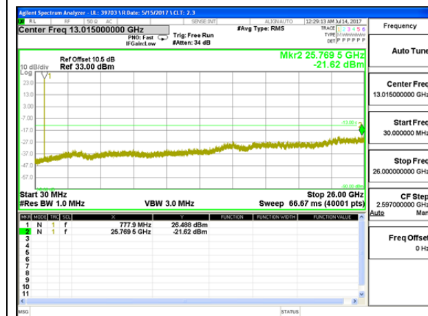
LTE B13 10MHz QPSK Middle Channel
