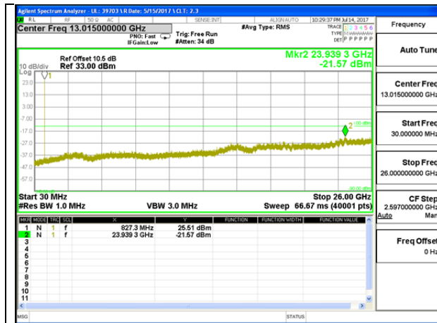
LTE B26 10MHz QPSK Middle Channel
