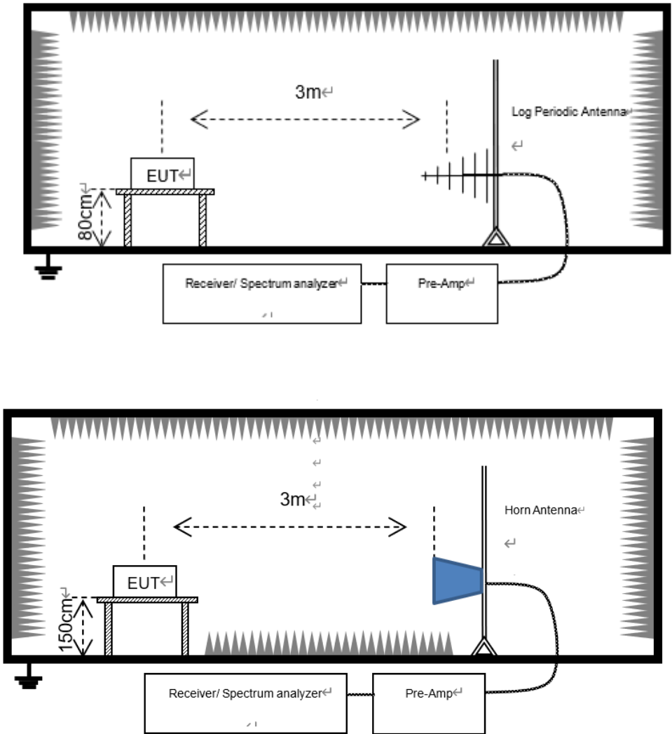
Diagram of Measurement Configuration for Radiation Test
