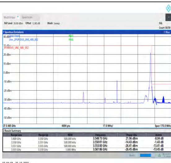
1-N77-3450-3550-PC2-30-70-H-2-DFT-PI2BPSK-Edge_1RB_Right-1@188-Ant1-1--PASS-see graph
