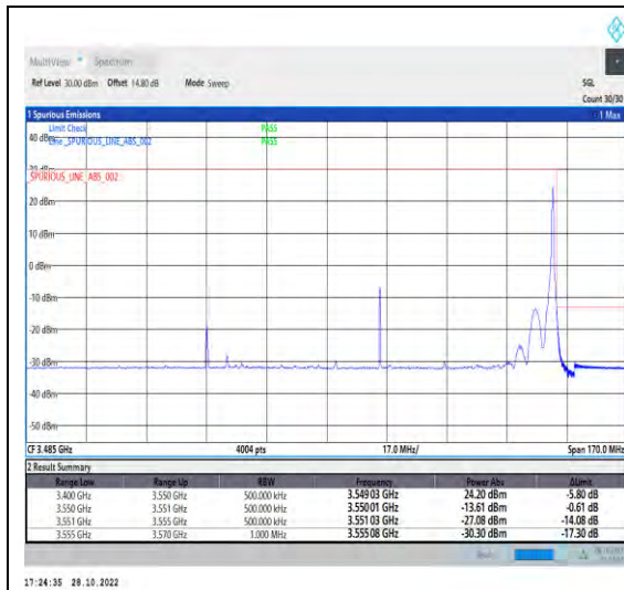
1-N77-3450-3550-PC2-30-100-H-2-DFT-PI2 BPSK-Edge_1RB_Right-1@272-Ant1-1--PAS S-see graph
