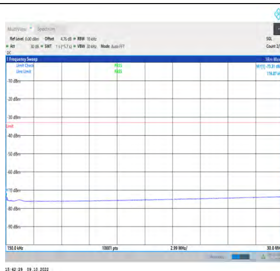
1-N77-3450-3550-PC2-30-100-L-1-DFT-QPSK-Edge _1RB_Left-1@0-0.15-30-Ant1-0.18--73.31--33-PASS
