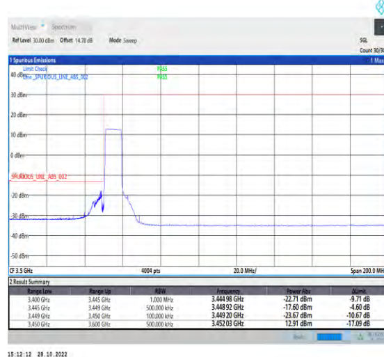
1-N77-3450-3550-PC2-30-10-L-6-CP-QPSK-Outer_Full-24@0-Ant1-1--PASS-see graph
