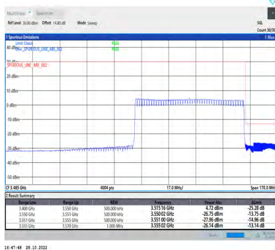
1-N77-3450-3550-PC2-30-70-H-6-CP-QPSK-Outer_Full-189@0-Ant1-1--PASS-see graph
