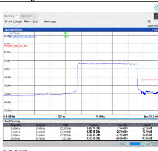
1-N77-3450-3550-PC2-30-70-H-3-DFT-PI2BPSK-Outer_Full-180@0-Ant1-1--PASS-see graph
