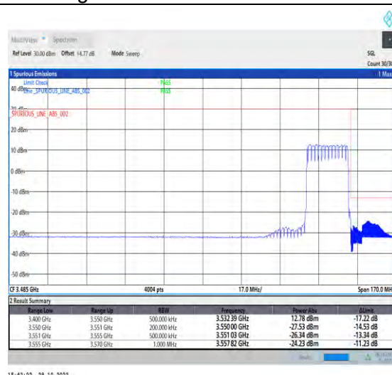
1-N77-3450-3550-PC2-30-20-H-3-DFT-PI2BPSK-Outer_Full-50@0-Ant1-1--PASS-see graph
