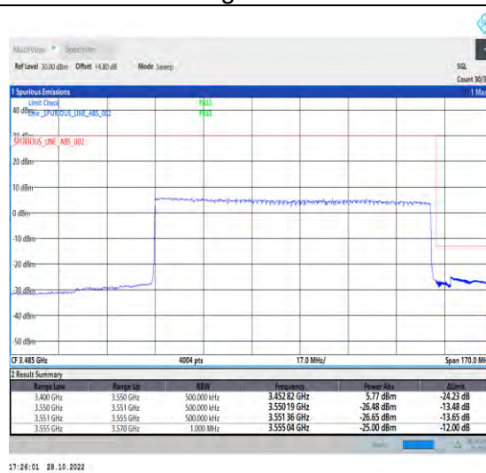
1-N77-3450-3550-PC2-30-100-H-3-DFT-PI2 BPSK-Outer_Full-270@0-Ant1-1--PASS-see graph
