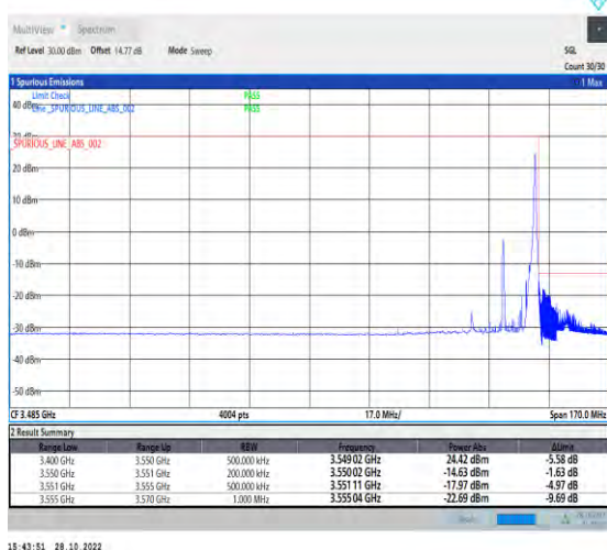
1-N77-3450-3550-PC2-30-20-H-5-CP-QPSK-Edge_1RB_Right-1@50-Ant1-1--PASS-see graph
