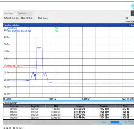
1-N77-3450-3550-PC2-30-10-L-3-DFT-PI2BPSK-Outer_Full-24@0-Ant1-1--PASS-see graph
