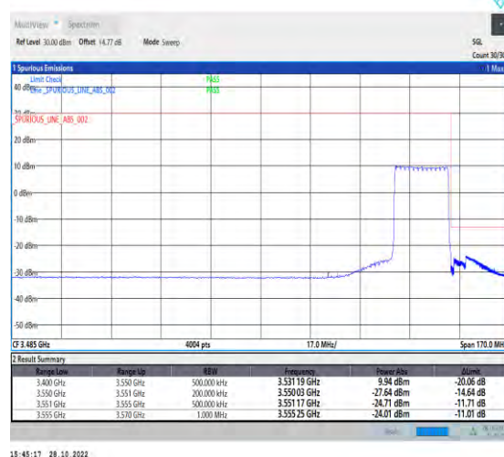
1-N77-3450-3550-PC2-30-20-H-6-CP-QPSK-Outer_Full-51@0-Ant1-1--PASS-see graph
