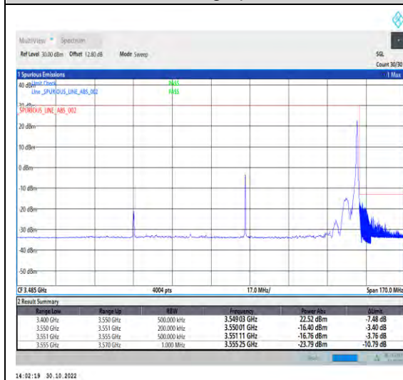
1-N77-3450-3550-PC2-30-100-H-5-CP-QPS K-Edge_1RB_Right-1@272-Ant1-1--PASS-s ee graph
