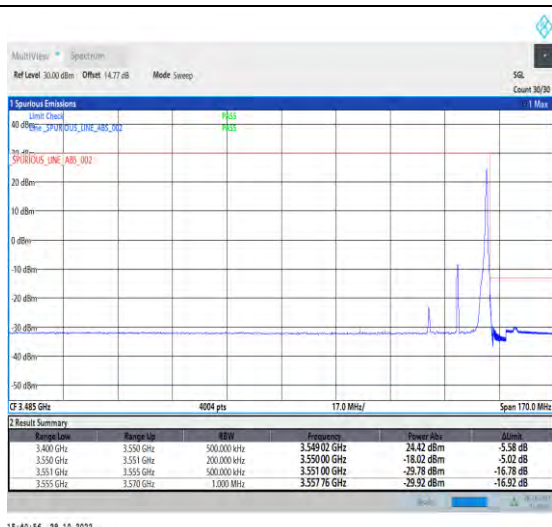
1-N77-3450-3550-PC2-30-20-H-2-DFT-PI2BPSK-Edge_1RB_Right-1@50-Ant1-1--PASS-see graph
