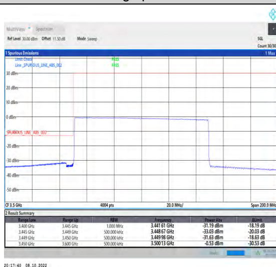
1-N77-3450-3550-PC2-30-100-L-6-CP-QPSK -Edge_1RB_Left-1@0-Ant1-1--PASS-see graph
