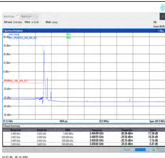
1-N77-3450-3550-PC2-30-10-L-1-DFT-PI2BPSK-Edge_1RB_Left-1@0-Ant1-1--PASS-see graph
