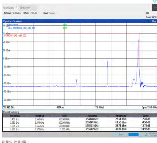
1-N77-3450-3550-PC2-30-70-H-5-CP-QPSK-Edge_1RB_Right-1@188-Ant1-1--PASS-see graph
