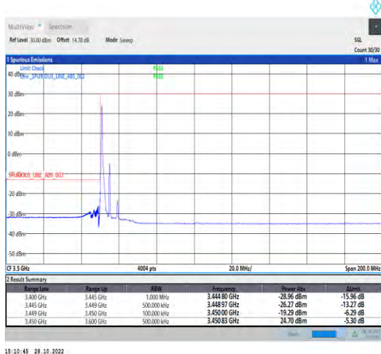
1-N77-3450-3550-PC2-30-10-L-4-CP-QPSK-Edge_1RB_Left-1@0-Ant1-1--PASS-see graph
