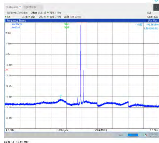
1-N77-3450-3550-PC2-30-100-L-1-DFT-QPSK-Inner_1RB_Left-1@1-1000-6000-Ant1-5953.50--35.03--13 -PASS
