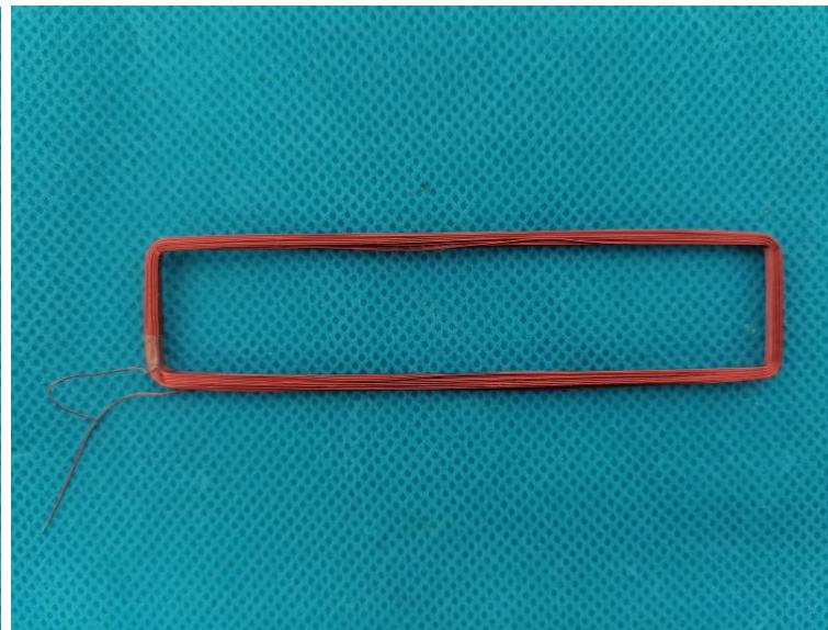
125kHz Antenna
