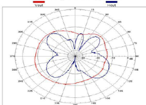
Far-field amplitude of XZ_plane.nsi
