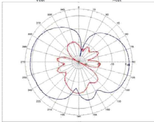
Far-field amplitude of XY_plane.nsi
