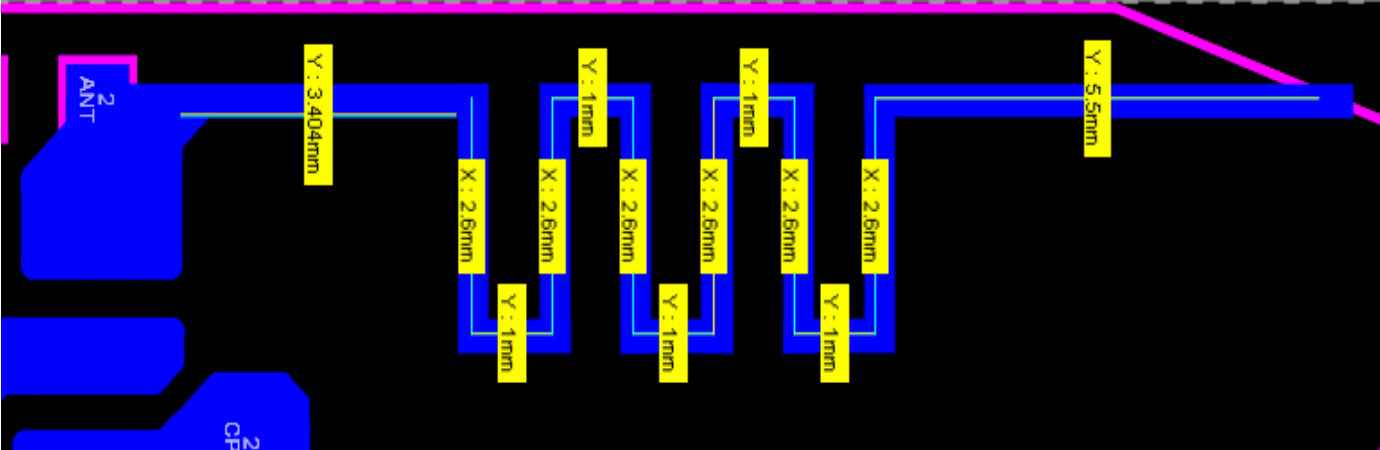
AntennaPhoto&Length
