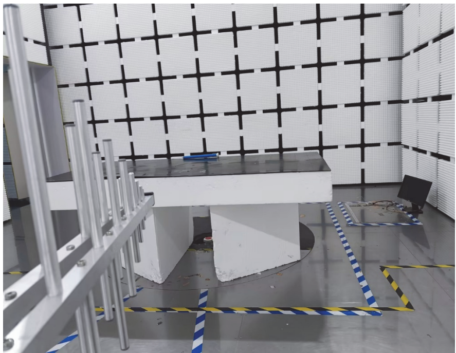
Radiation Emission Test Setup (30MHz to 1GHz)
