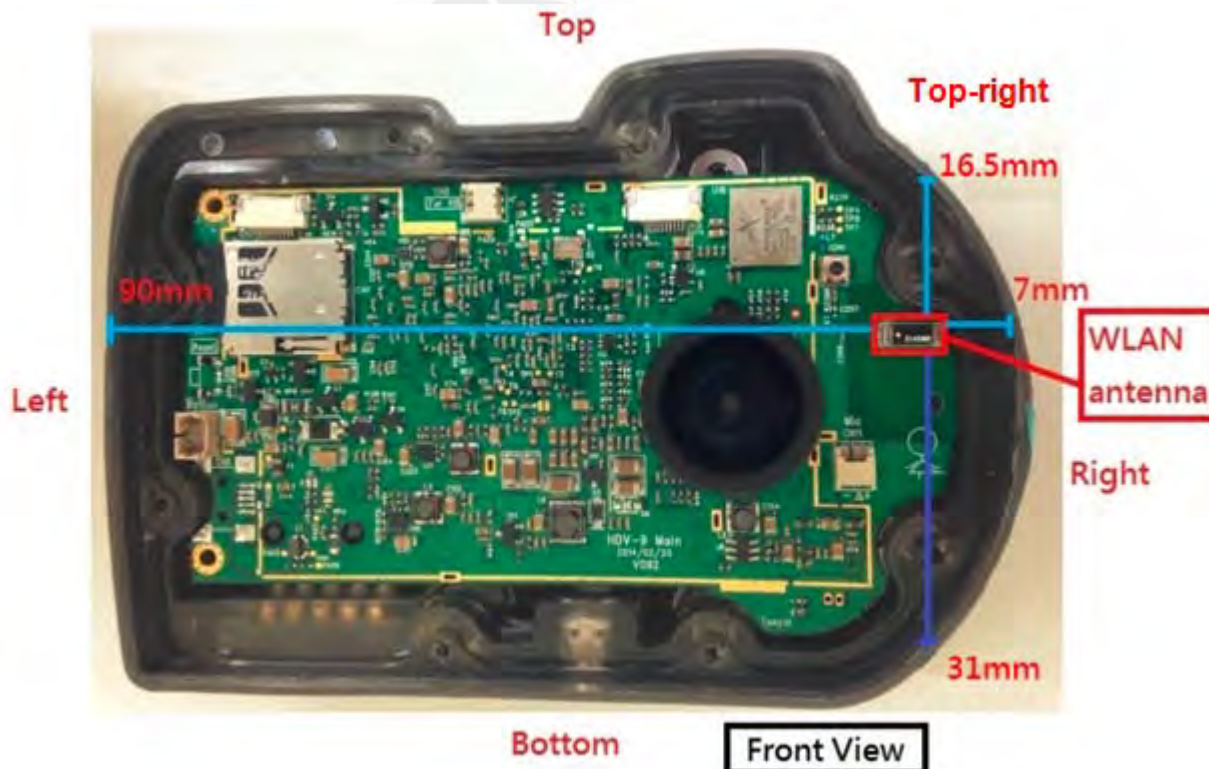
Fig.9 Antenna position (Front view)
