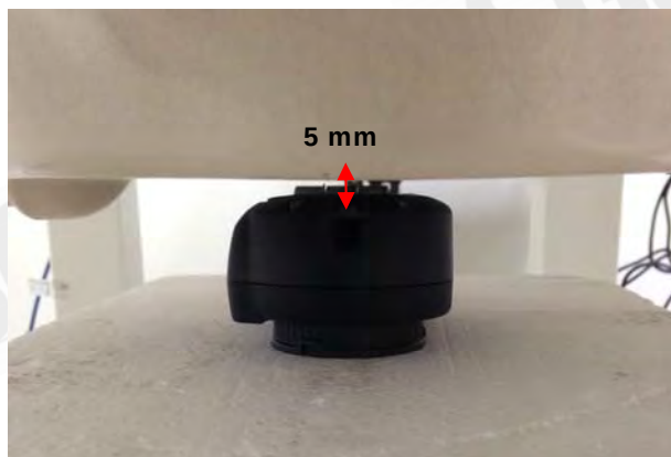
Fig.4 Back side to flat phantom
