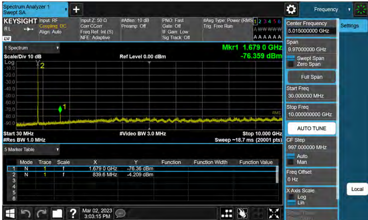
Sub6 n5. Conducted Spurious Plot (168800ch_10 MHz_BPSK_RB 1_1)
