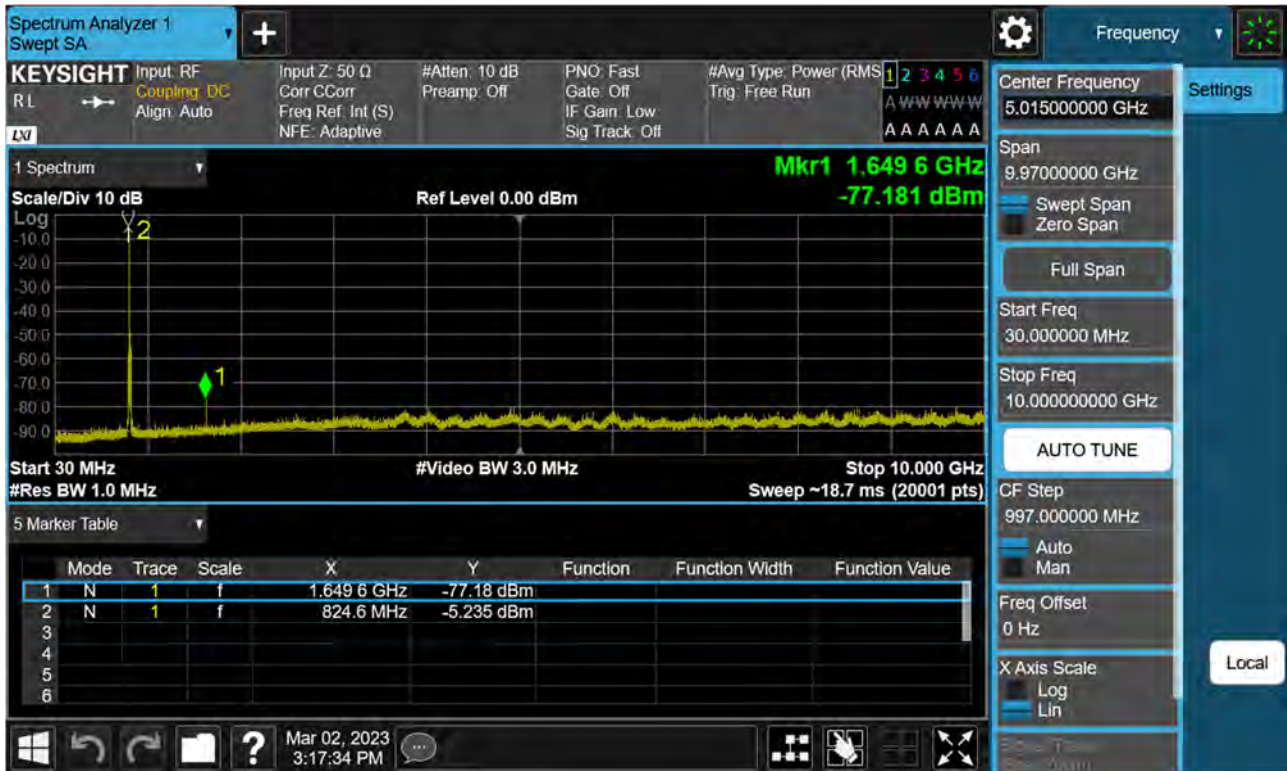
Sub6 n5. Conducted Spurious Plot (166800ch_20 MHz_BPSK_RB 1_1)
