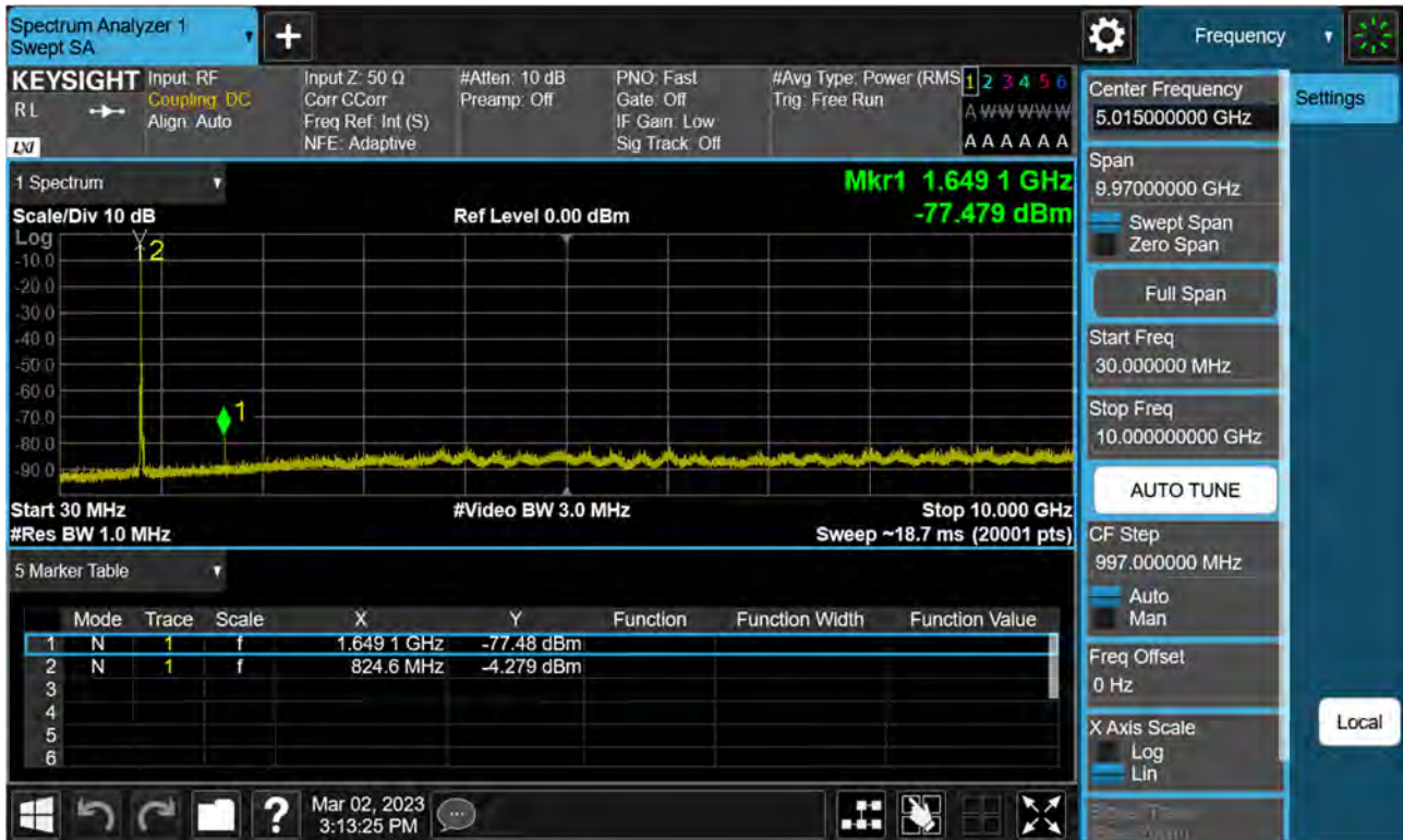
Sub6 n5. Conducted Spurious Plot (166300ch_15 MHz_BPSK_RB 1_1)
