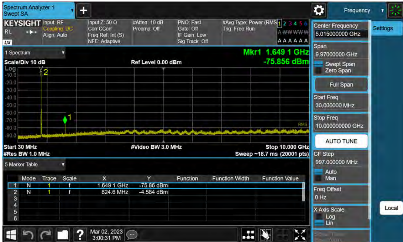
Sub6 n5. Conducted Spurious Plot (165800ch_10 MHz_BPSK_RB 1_1)
