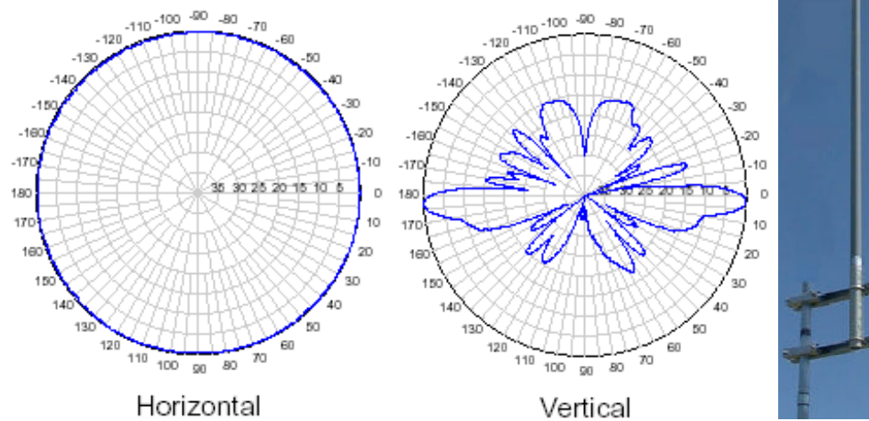
Figure H-5: Omni-Directional 360°/12 dBi (3° Lobe Tilt) radiation pattern (at mid-band)
