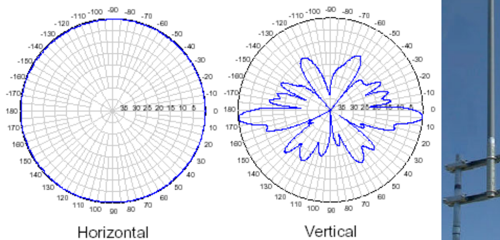
Figure H-6: Omni-Directional 360°/12 dBi (5° Lobe Tilt) radiation pattern (at mid-band)
