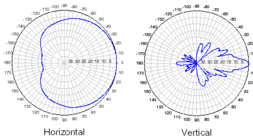
Figure H-2: Panel 120°/16 dBi antenna radiation pattern (at mid-band)
