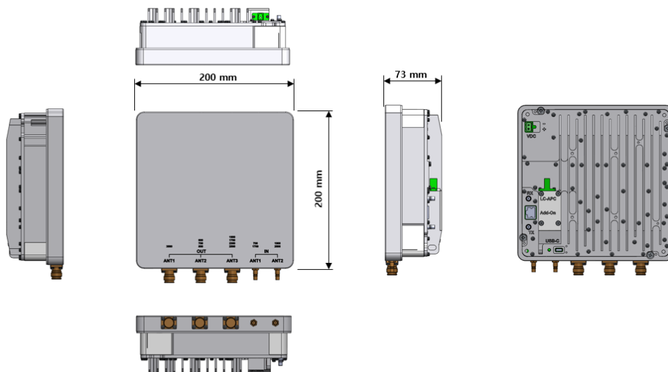
Figure 3. Dimension used to install eROU (internal)
